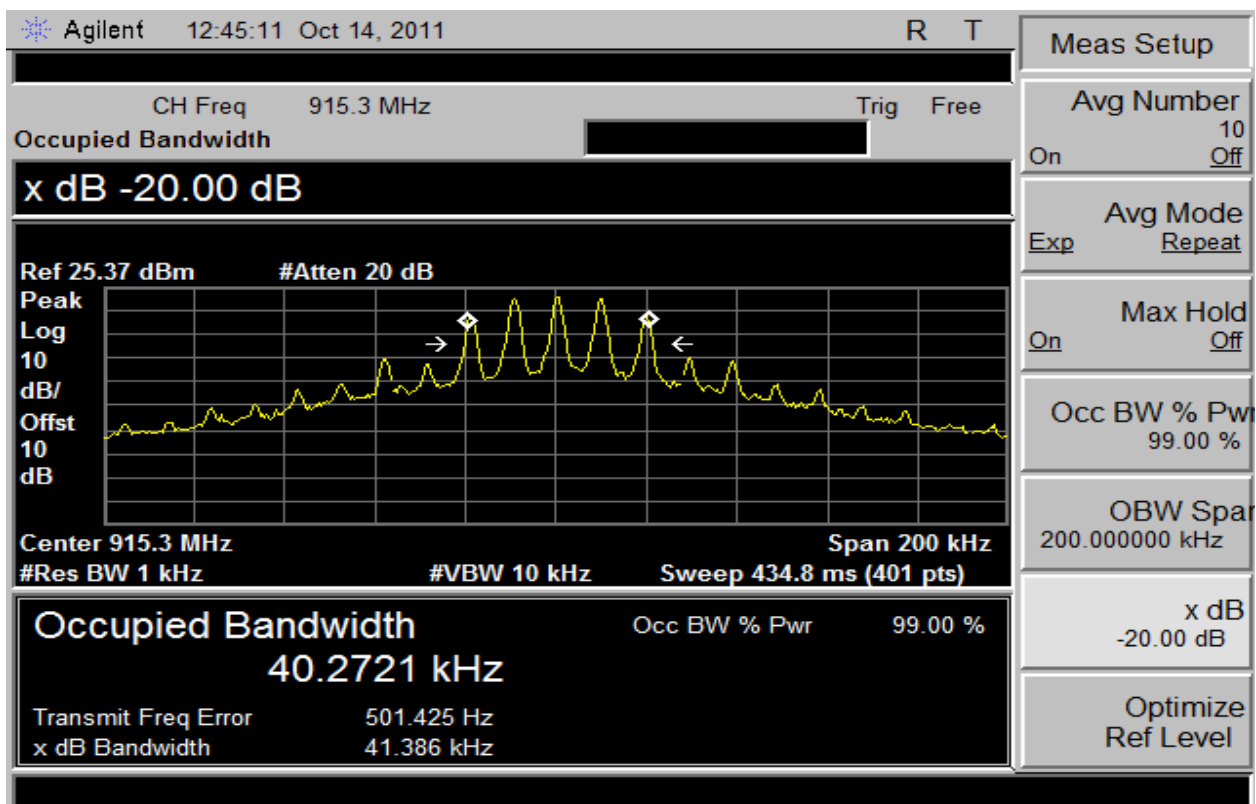
Plot 4 – Middle Channel – 20 BW FM Modulation
