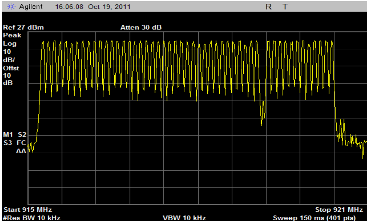
Plot 21 – Set 3 (915-920MHz)
