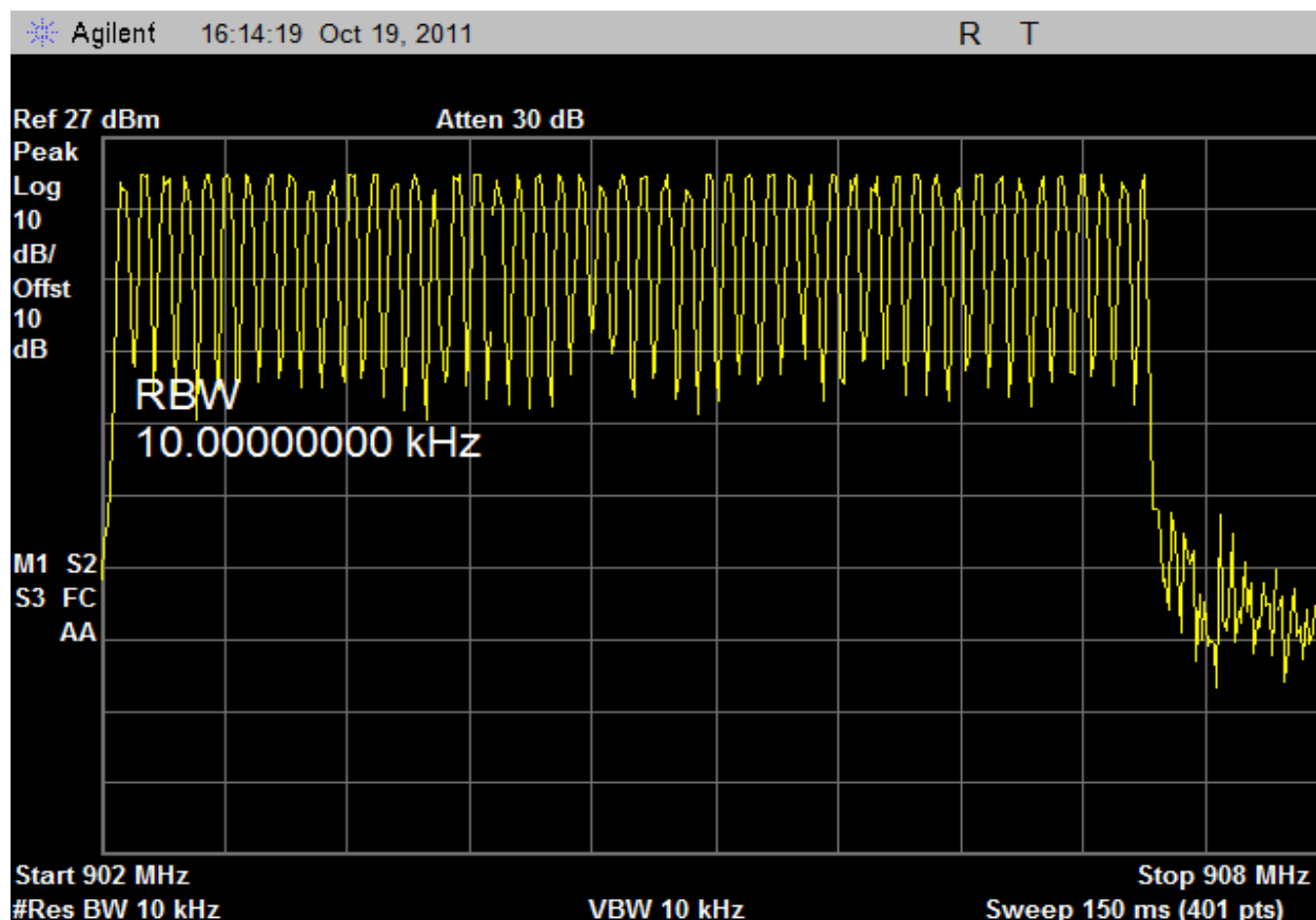
Plot 19 – Set 1 (902-907MHz)
