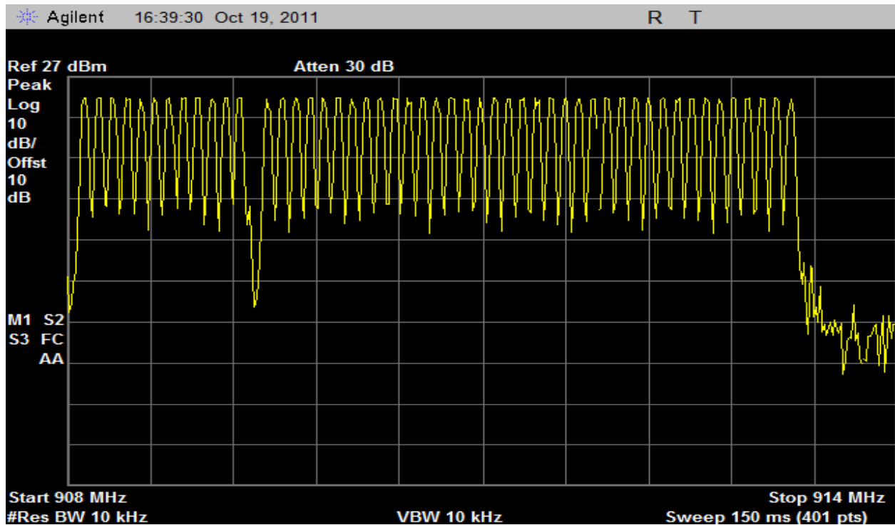
Plot 20 – Set 2 (908-913MHz)
