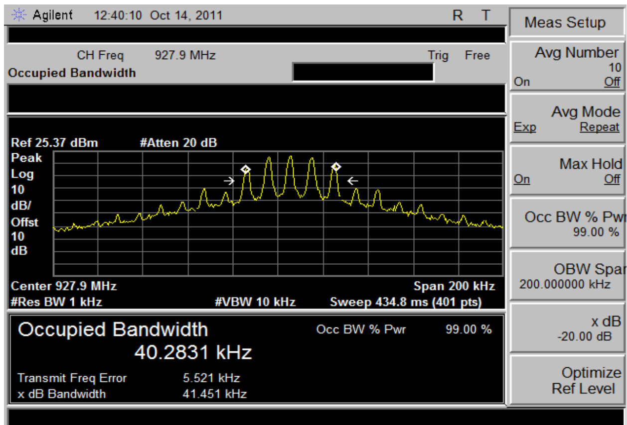
Plot 5 – Highest Channel – 20dB BW FM Modulation
