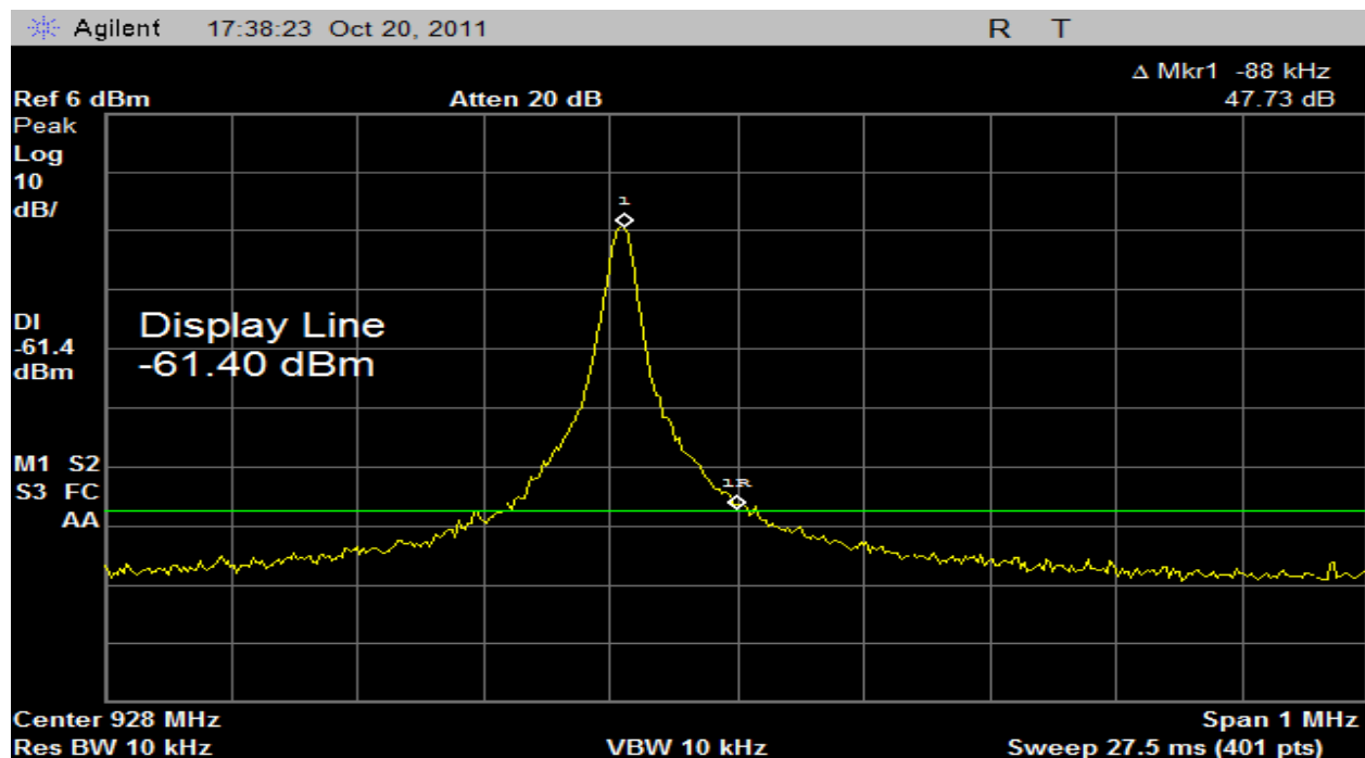
Plot 16 – Highest Channel (Band Edge)
