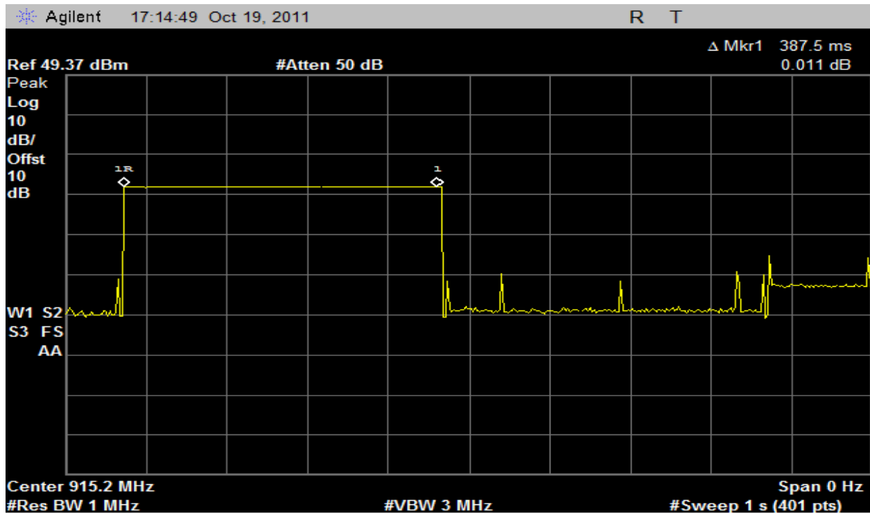
Plot 17 – Dwell Time
