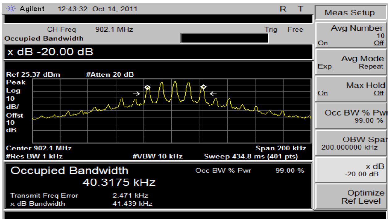
Plot 3 – Lowest Channel – 20dB BW FM Modulation
