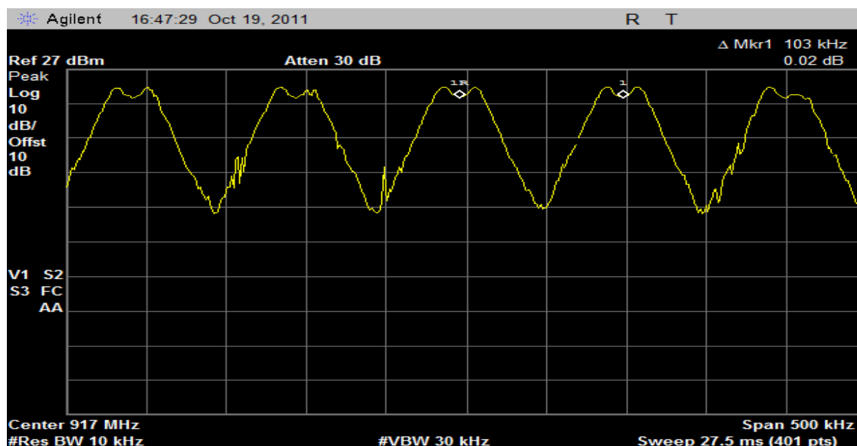
Plot 23 – Carrier Frequency Separation (Using Delta Marker Method)
