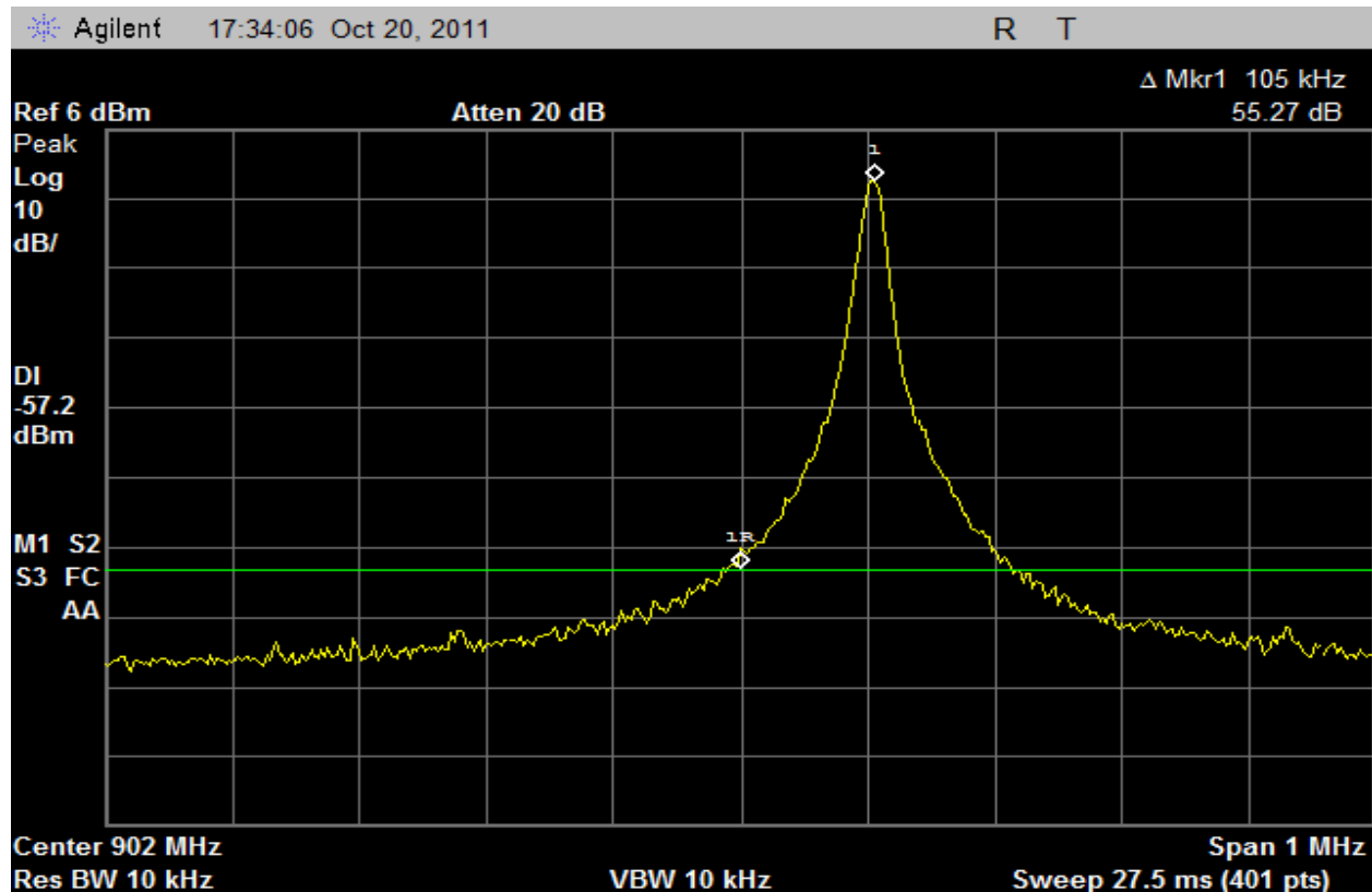
Plot 15 – Lowest Channel (Band Edge)
