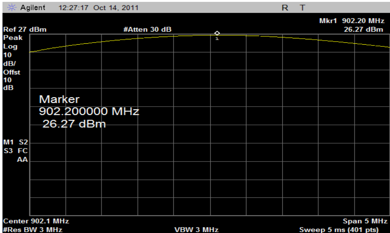
Plot 6 – Lowest Channel - Output Power
