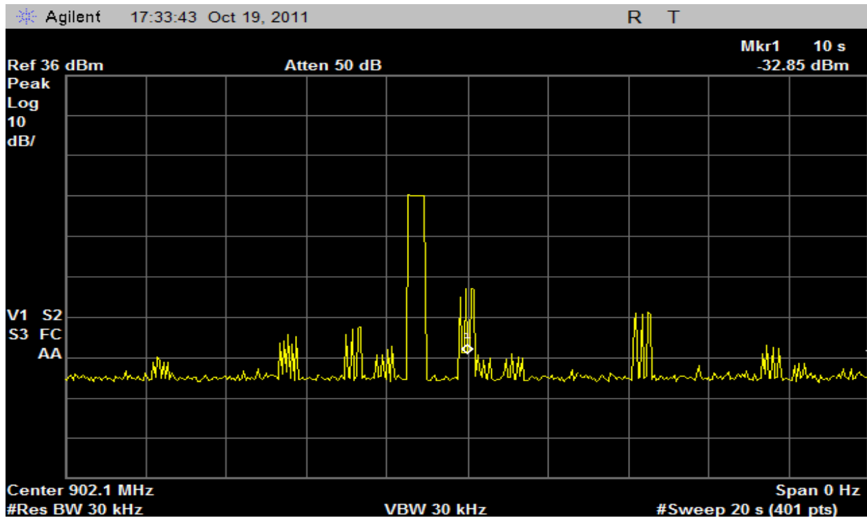
Plot 18 – # of Hops in 20 second period
