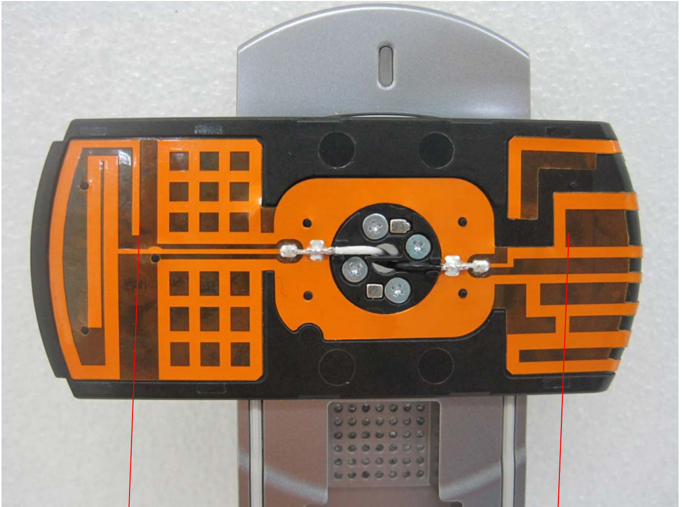
Diversity / MIMO antenna (TX and RX)
