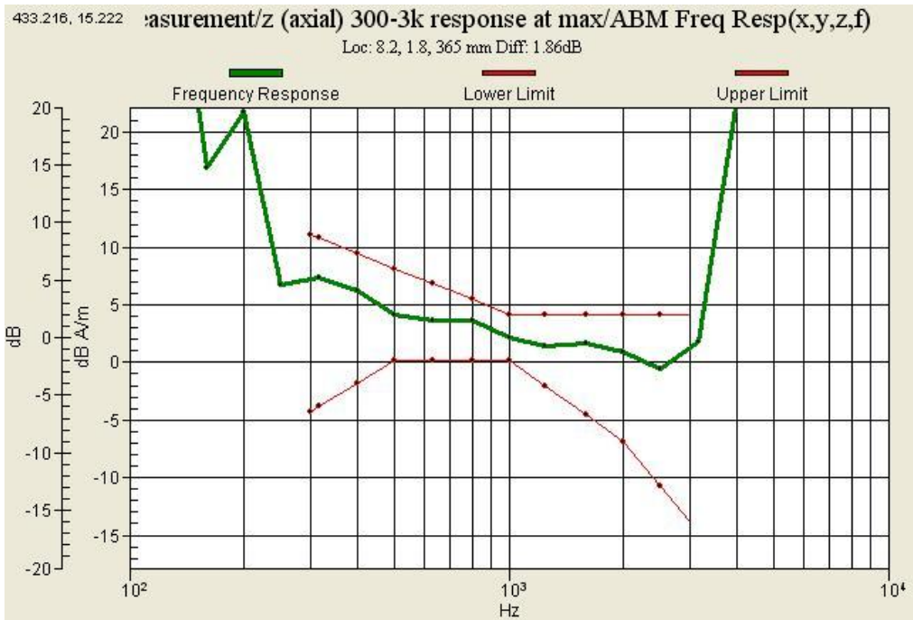
Graph 20 : GSM 1900 (CH 661) Frequency Response_Wireless Charger Battery
