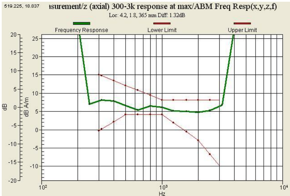
Graph 4 : CDMA 800 (CH 384) Frequency Response_Extended Battery
