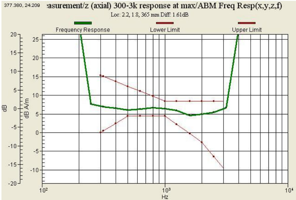
Graph 7 : PCS 1900 (CH 600) Frequency Response
