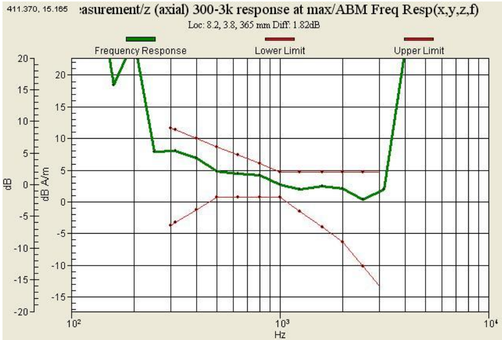
Graph 15 : GSM850 (CH 190) Frequency Response_Wireless charger cover
