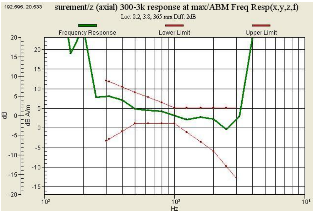
Graph 12 : GSM850 (CH 190) Frequency Response
