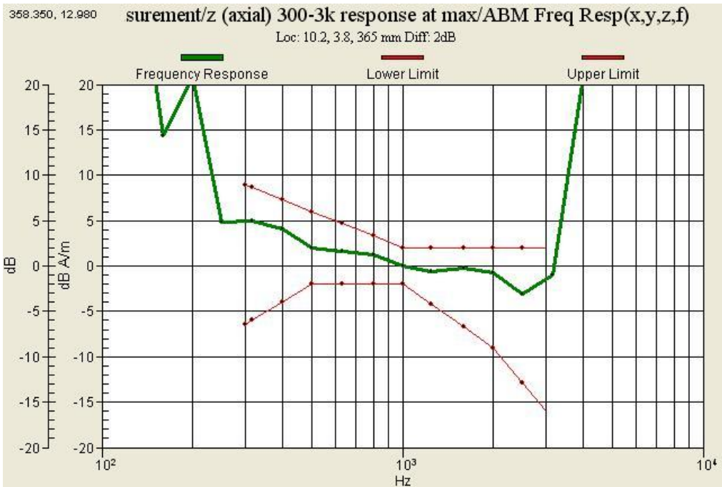
Graph 16 : GSM 1900 (CH 512) Frequency Response
