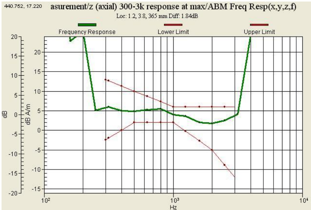
Graph 8 : PCS 1900 (CH 1175) Frequency Response
