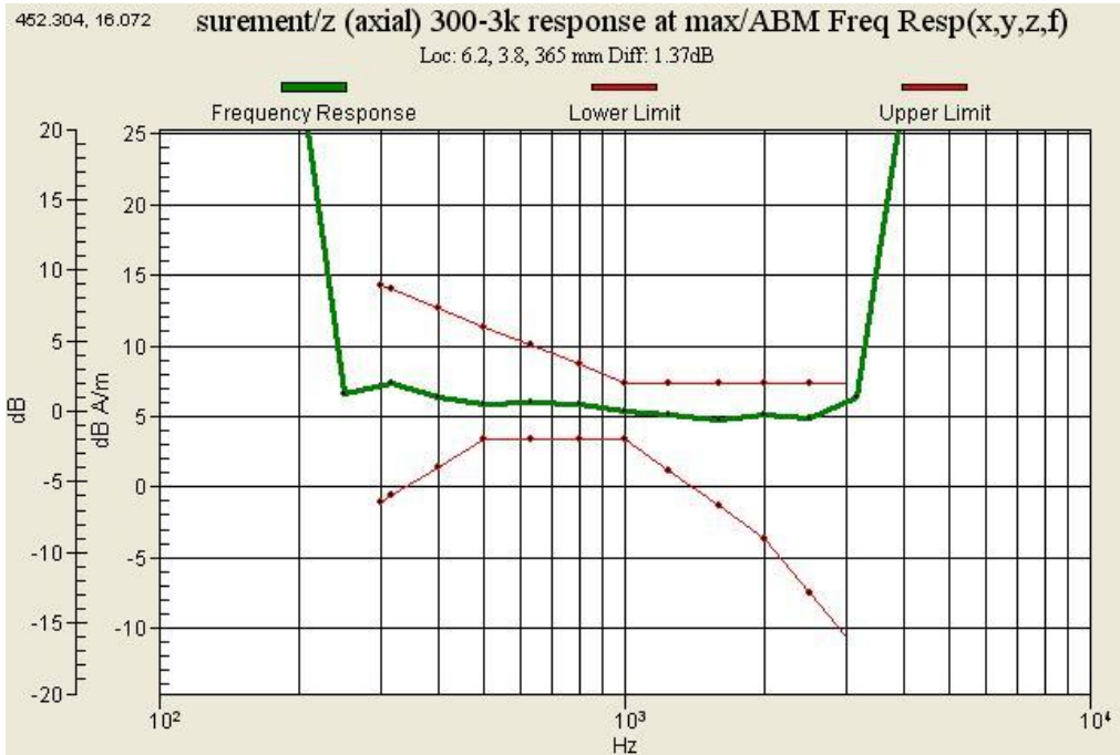
Graph 5 : CDMA 800 (CH 384) Frequency Response _ Wireless charger cover
