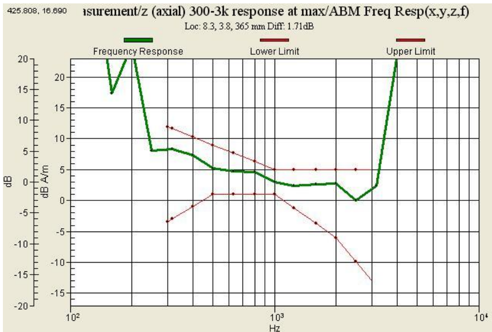
Graph 14 : GSM850 (CH 190) Frequency Response_Extended Battery
