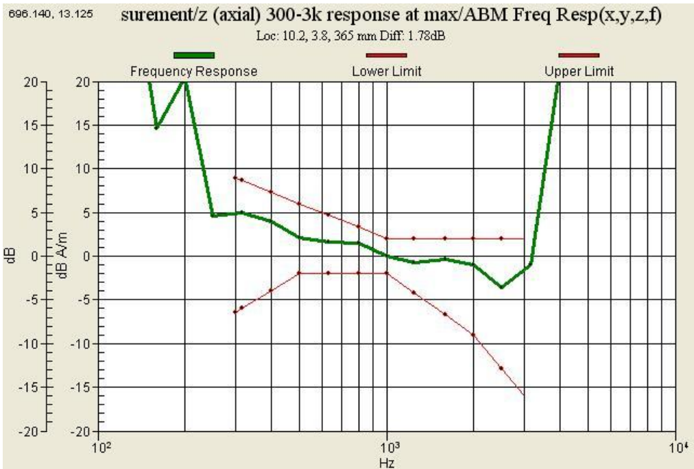
Graph 18 : GSM 1900 (CH 810) Frequency Response
