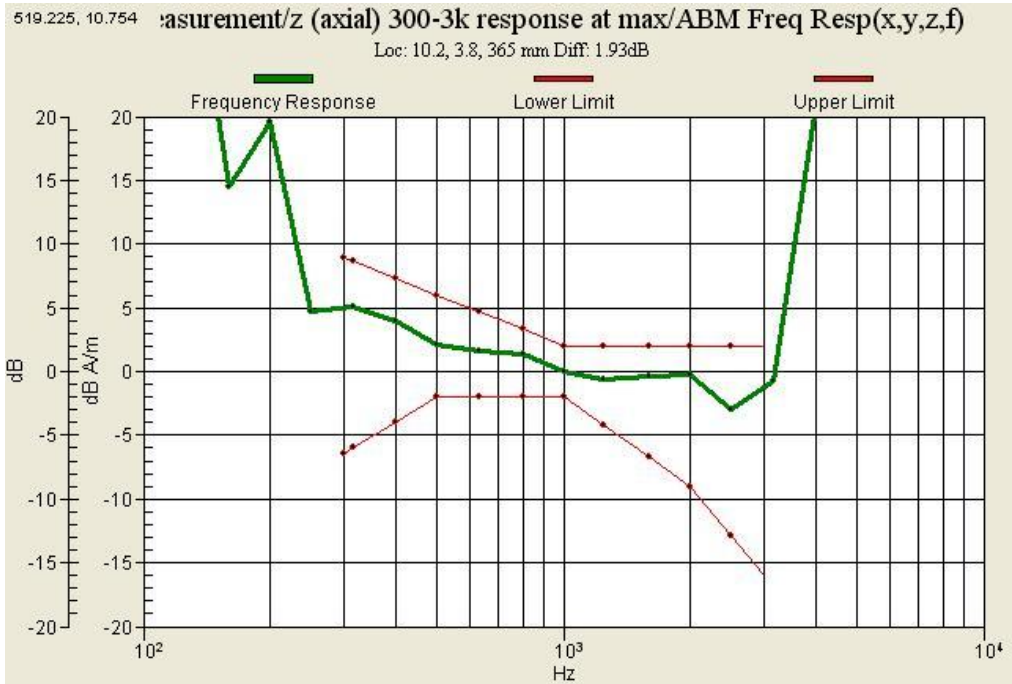
Graph 17 : GSM 1900 (CH 661) Frequency Response
