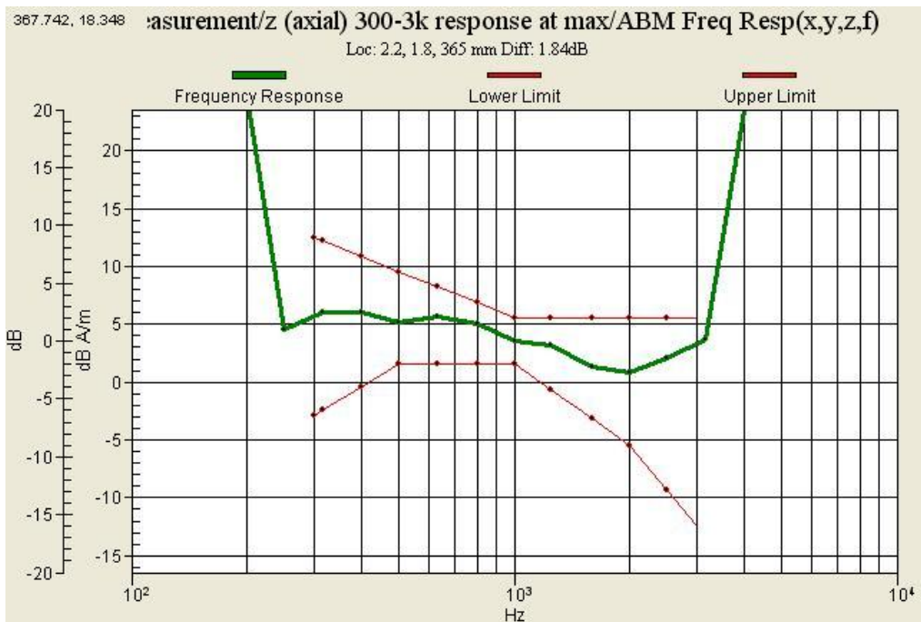
Graph 10 : PCS 1900 (CH 600) Frequency Response_Wireless charger cover
