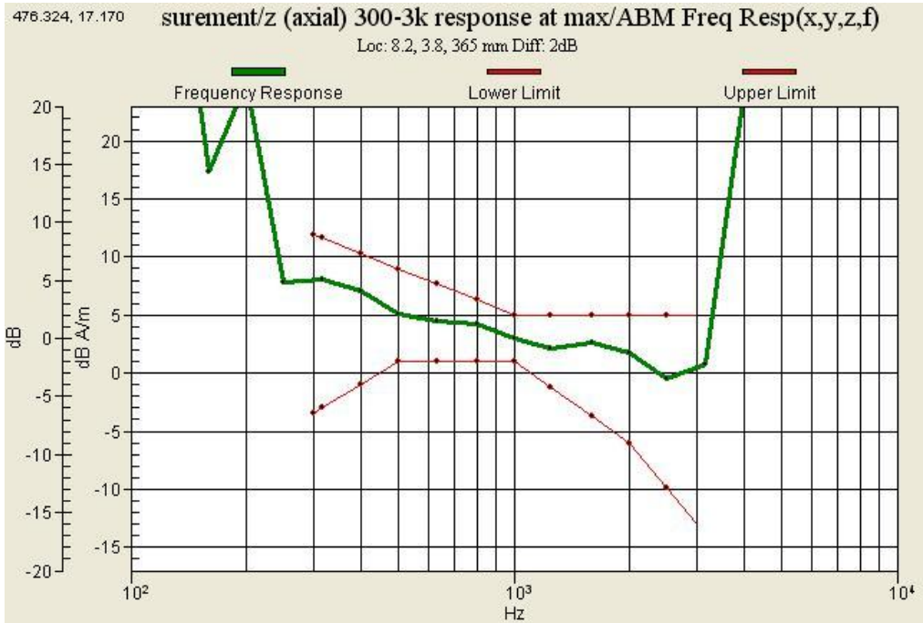
Graph 11 : GSM850 (CH 128) Frequency Response
