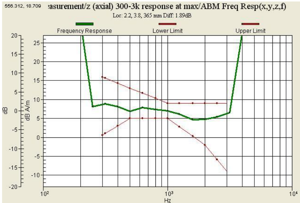
Graph 9 : PCS 1900 (CH 600) Frequency Response_Extended Battery
