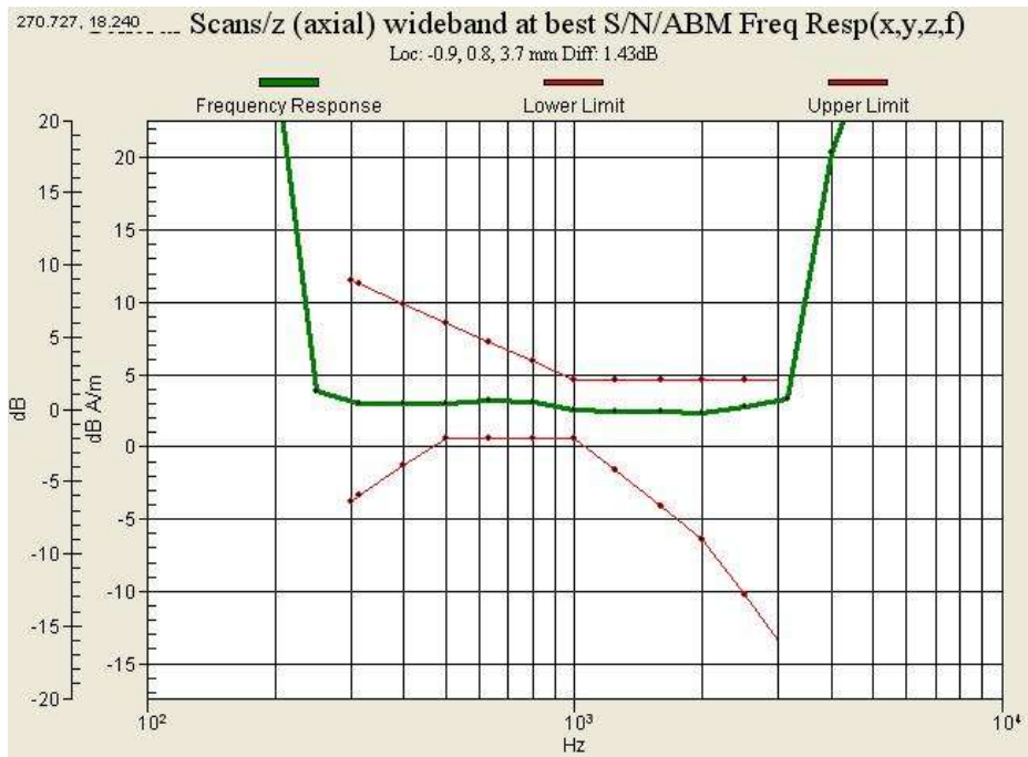
Graph 8 : WCDMA 850(CH 4183) Frequency Response
