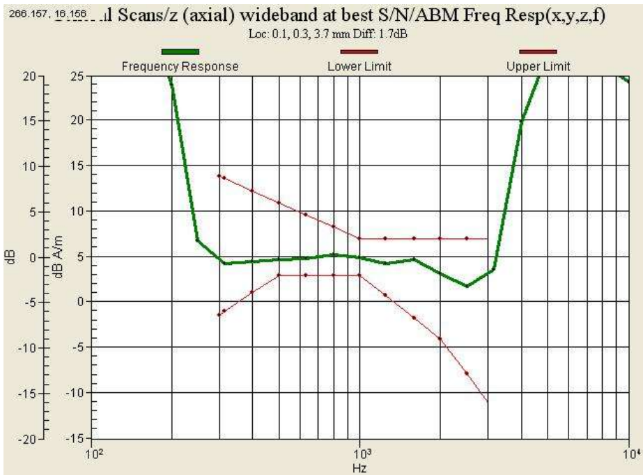
Graph 4 : GSM 1900(CH 512) Frequency Response
