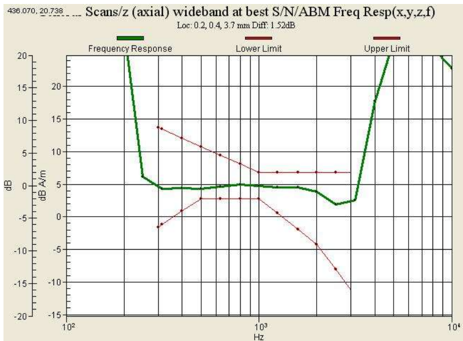
Graph 2 : GSM 850(CH 190) Frequency Response
