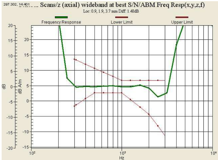
Graph 6 : GSM 1900 (CH 810) Frequency Response
