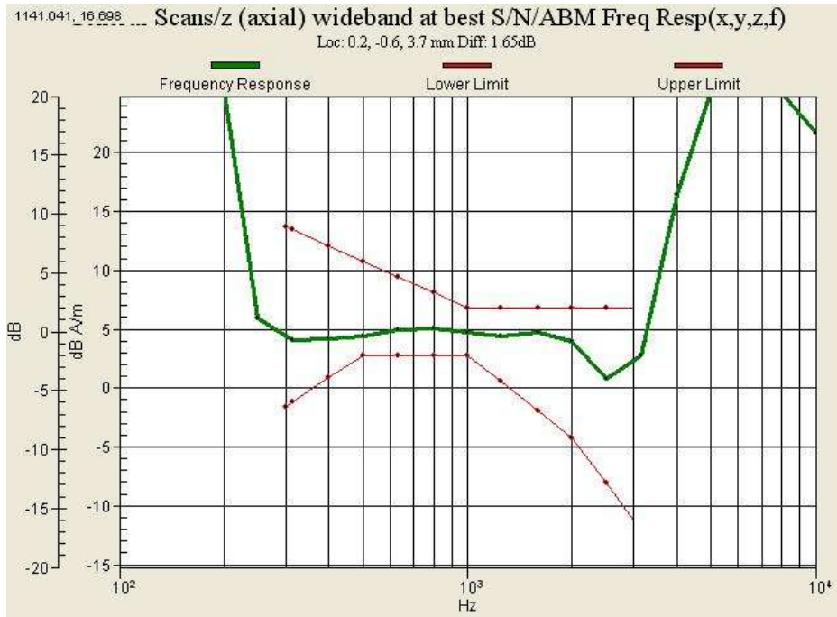
Graph 5 : GSM 1900 (CH 661) Frequency Response
