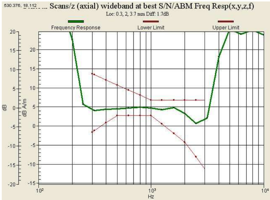
Graph 3 : GSM 850 (CH 251) Frequency Response
