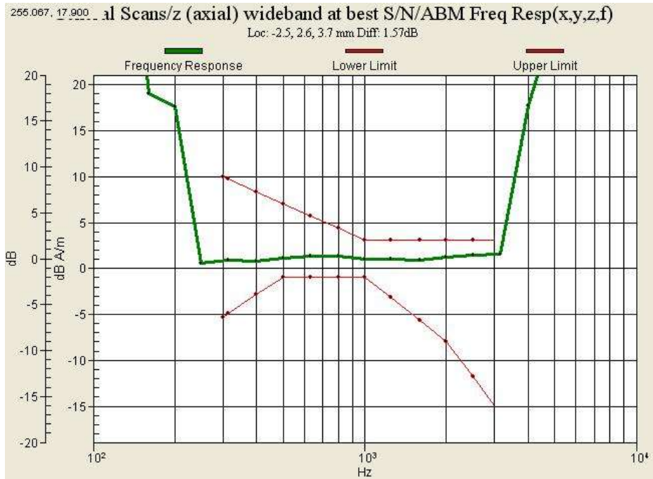
Graph 10 : WCDMA 1900 (CH 9262) Frequency Response
