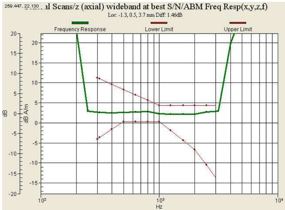
Graph 12 : WCDMA 1900 (CH 9583) Frequency Response
