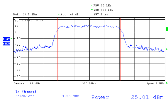
Figure. 8 Wireless Device Modulated Signal
