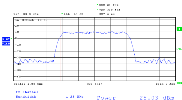
Figure. 7 Signal Generator Modulated Signal
