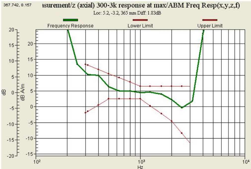
Graph 6 : GSM 1900 (CH 810) Frequency Response
