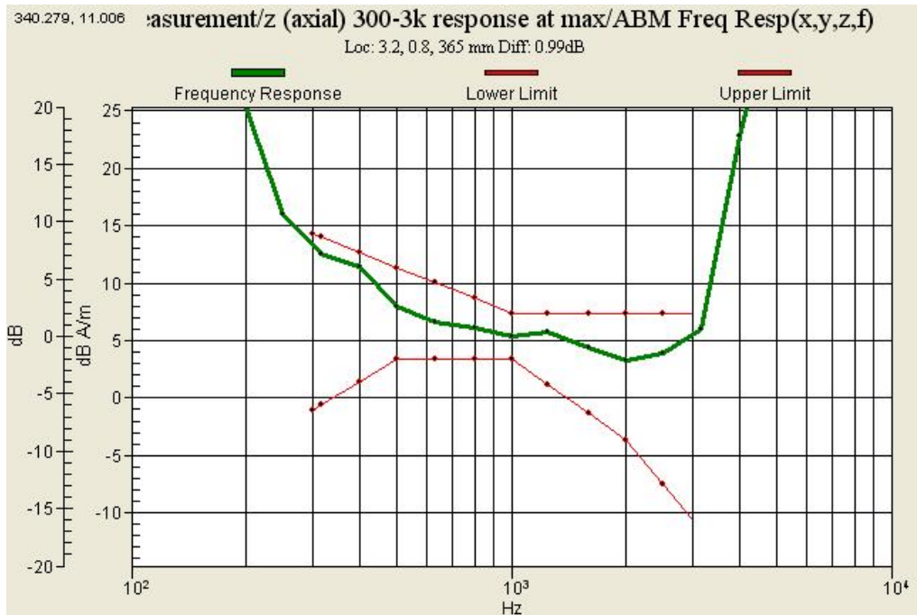
Graph 12 : WCDMA 1900 (CH 9583) Frequency Response Slide down
