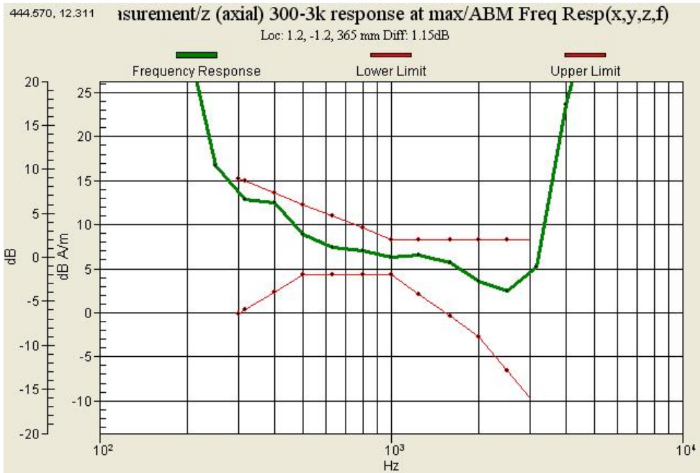
Graph 5 : GSM 1900 (CH 661) Frequency Response
