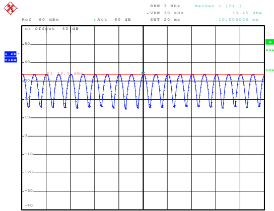
835MHz - 80% AM
