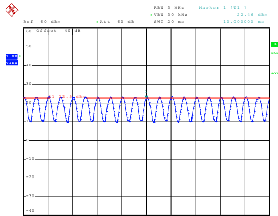
1880MHz - 80% AM
