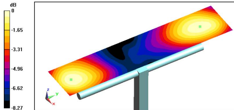
0 dB = 145.9V/m
