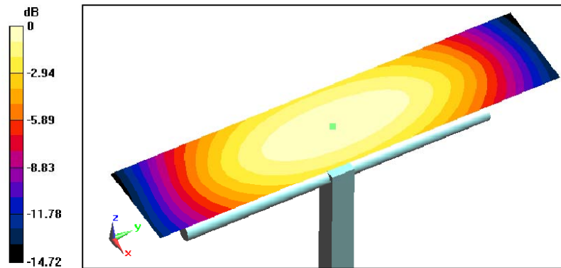
0 dB = 0.460A/m
