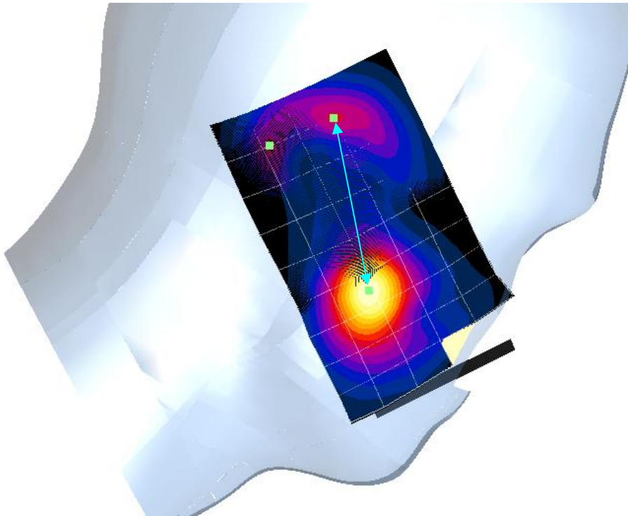
WiFi Max. SAR Peak Location
