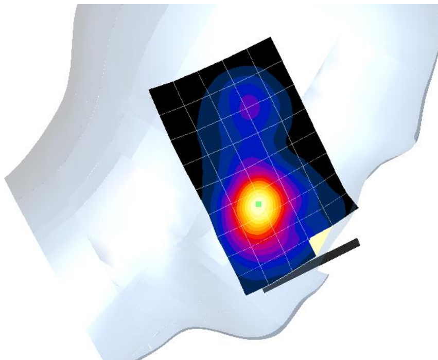
3G Max.SAR Peak Location
