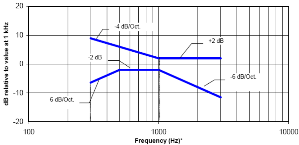
Figure 4 : Magnetic field frequency response for WDs with field strength \leq -15 dB (A/m) at 1 kHz
