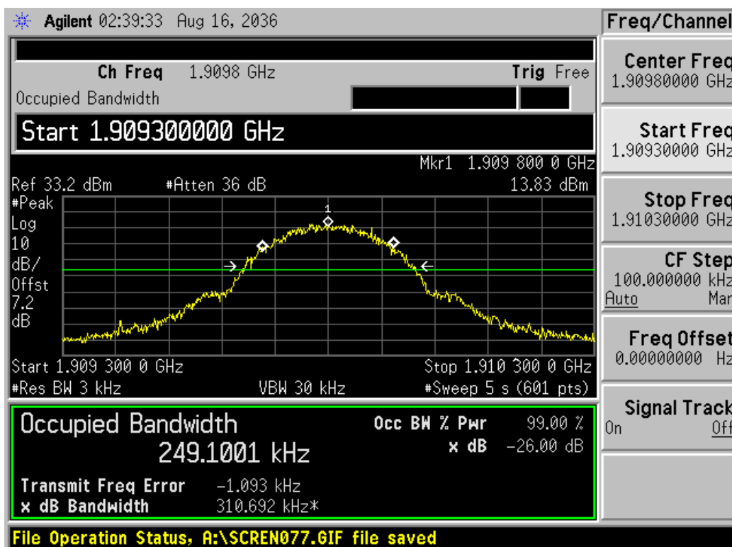
Channel 810
