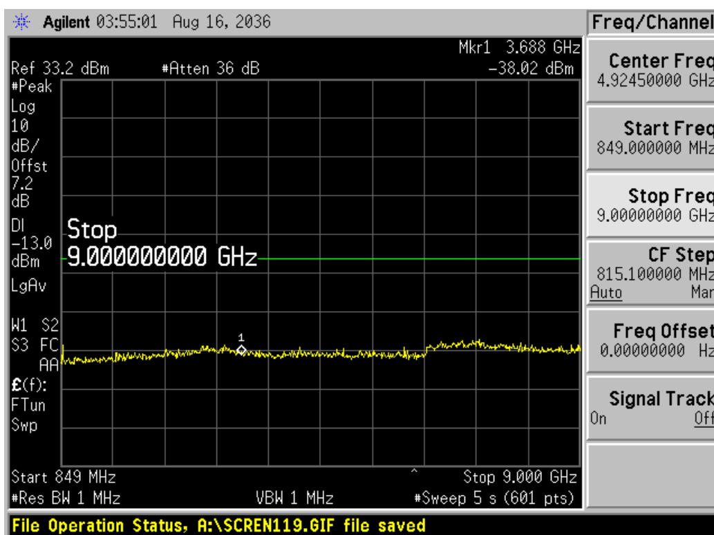
Channel 189, 849MHz~9GHz
