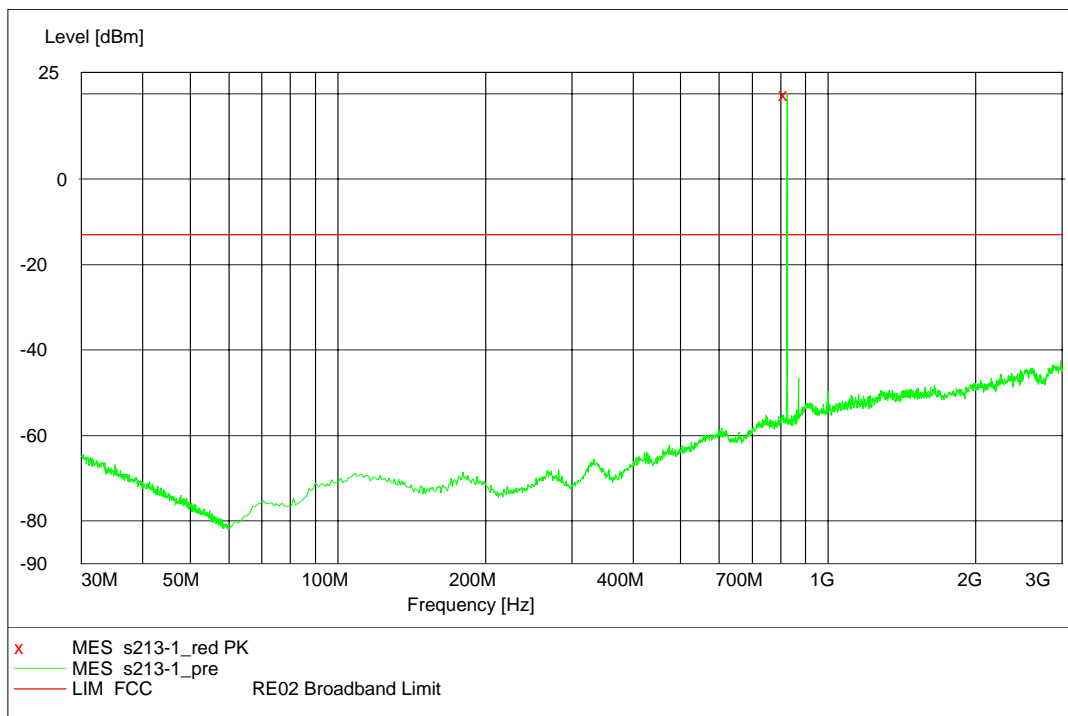
Channel 189, 30MHz~3GHz
