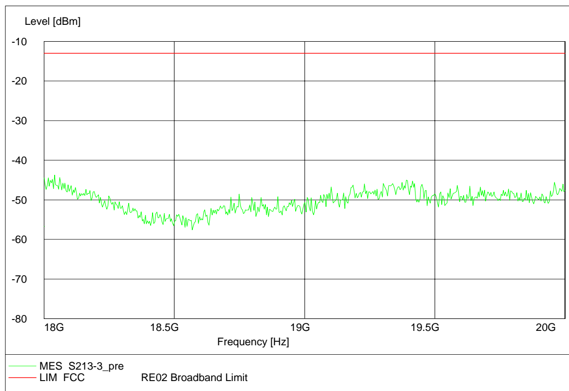
Channel 661, 18GHz~20GHz
