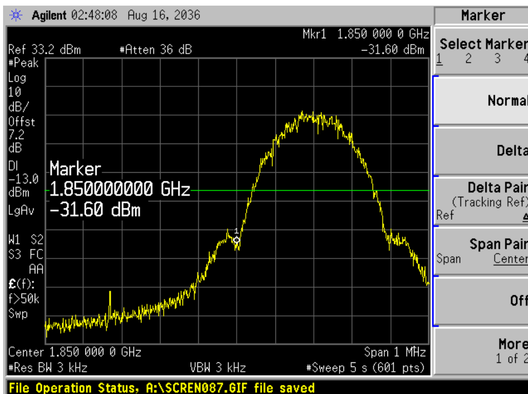
Channel 512
