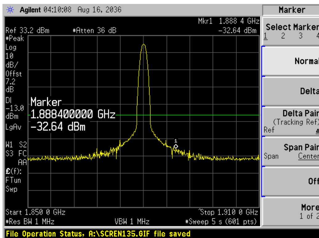
Channel 661, 1850MHz~1910MHz
