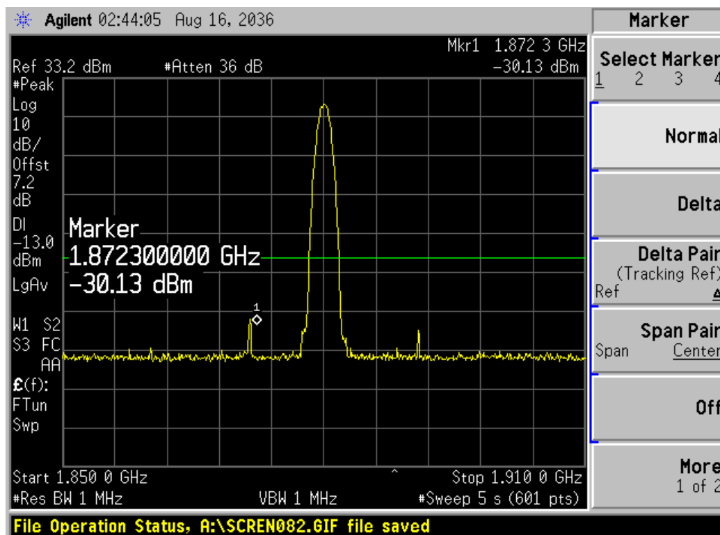
Channel 661, 1850MHz~1910MHz
