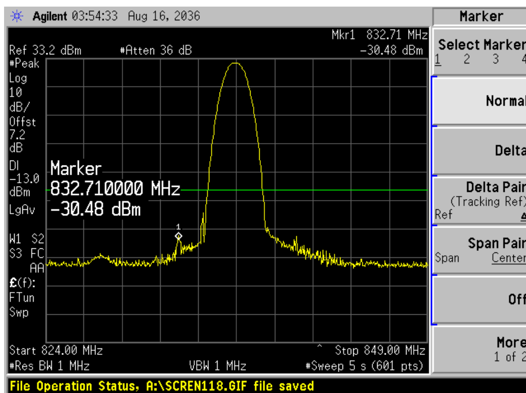
Channel 189, 824MHz~849MHz
