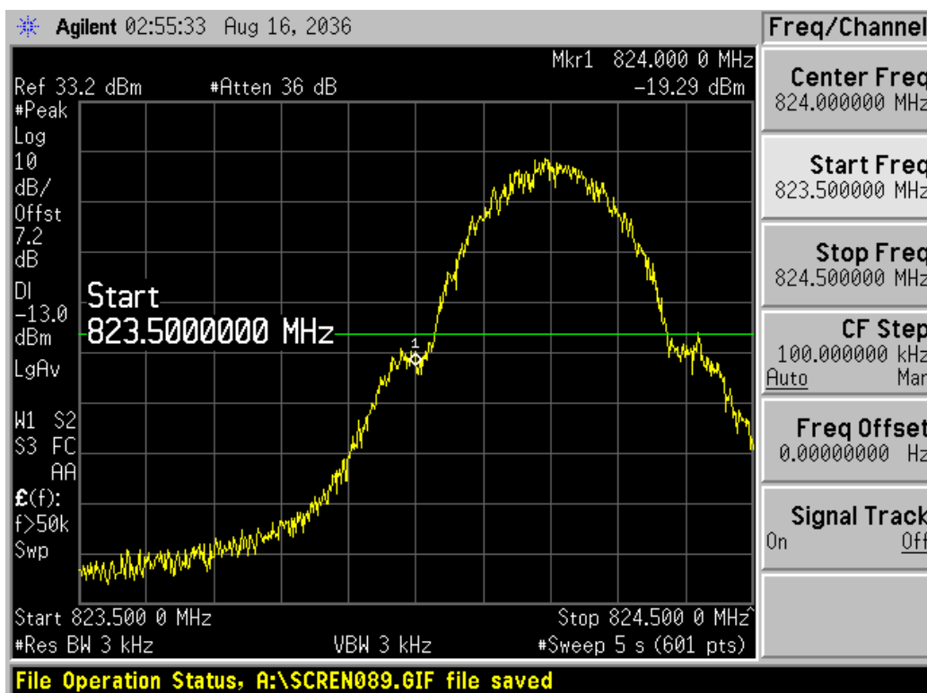
Channel 128
