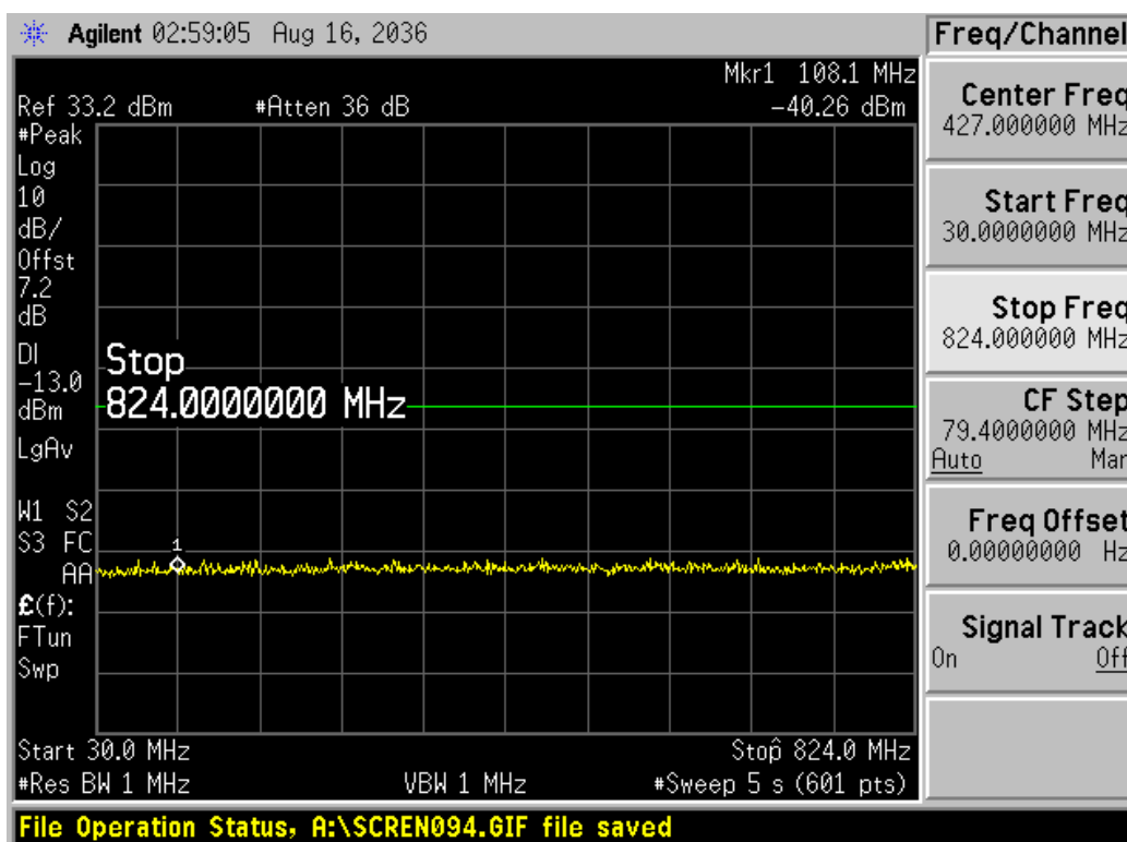
Channel 189, 30MHz~824MHz
