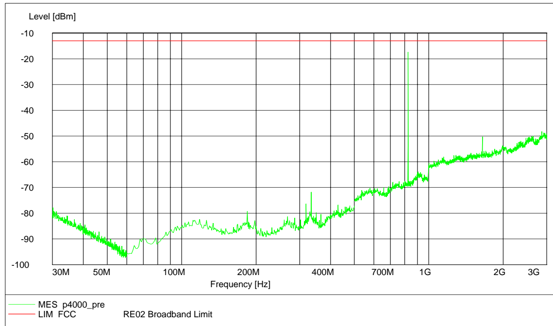
Channel 189, 30MHz~3GHz
