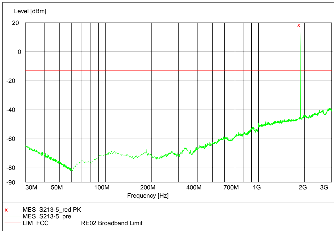
Channel 661, 30MHz~3GHz
