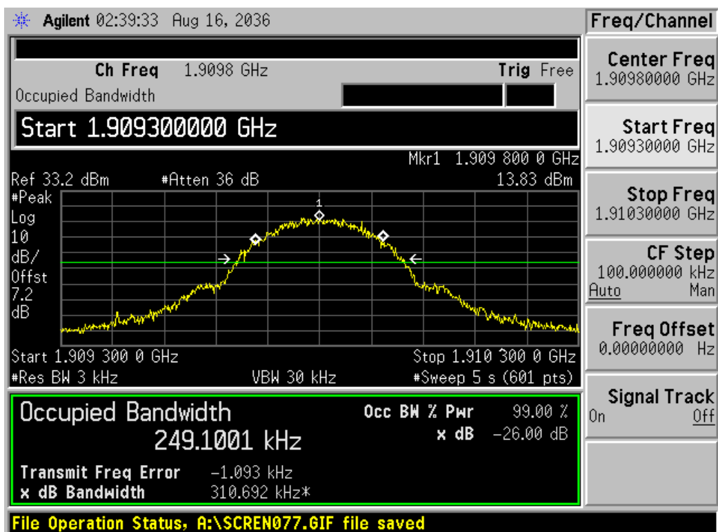
Channel 810
