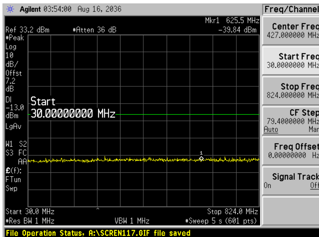
Channel 189, 30MHz~824MHz
