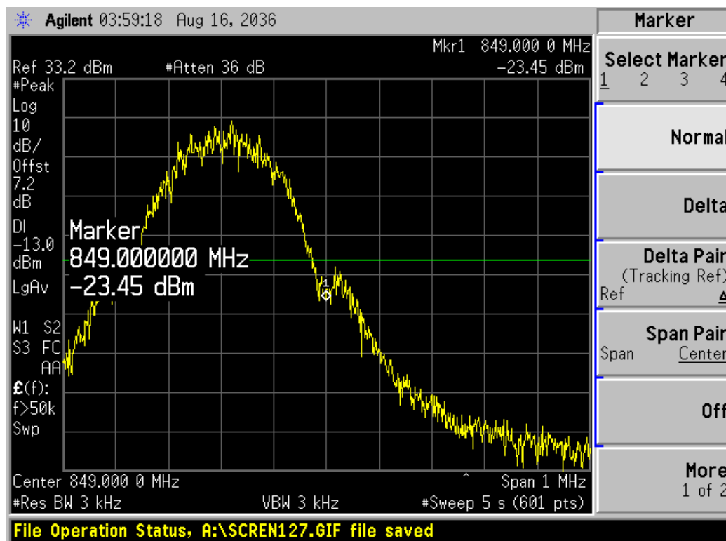
Channel 251
