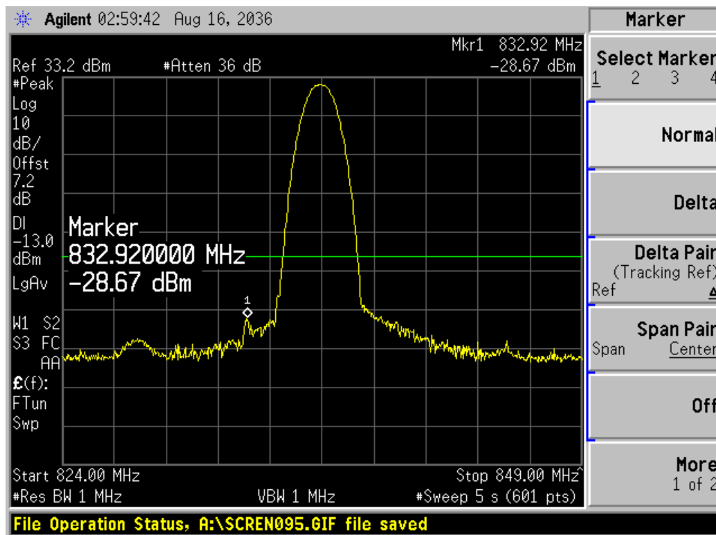
Channel 189, 824MHz~849MHz
