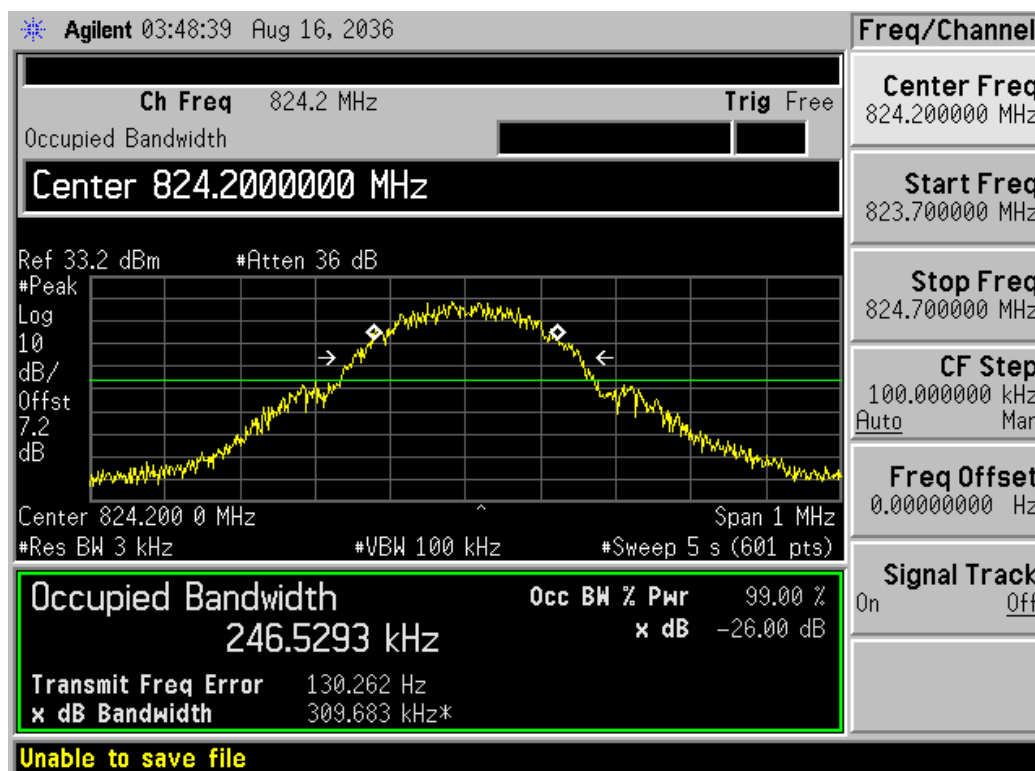
Channel 128
