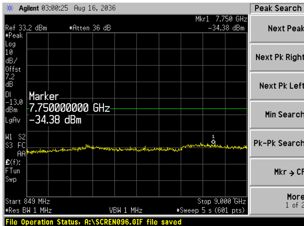
Channel 189, 849MHz~9GHz
