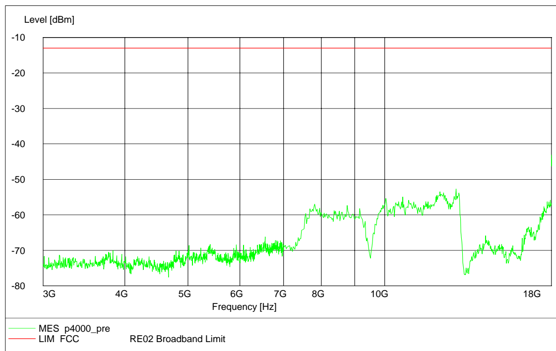
Channel 661, 3GHz~18GHz
