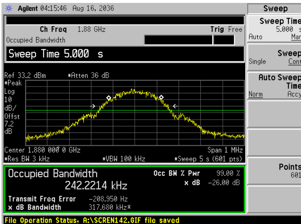
Channel 661
