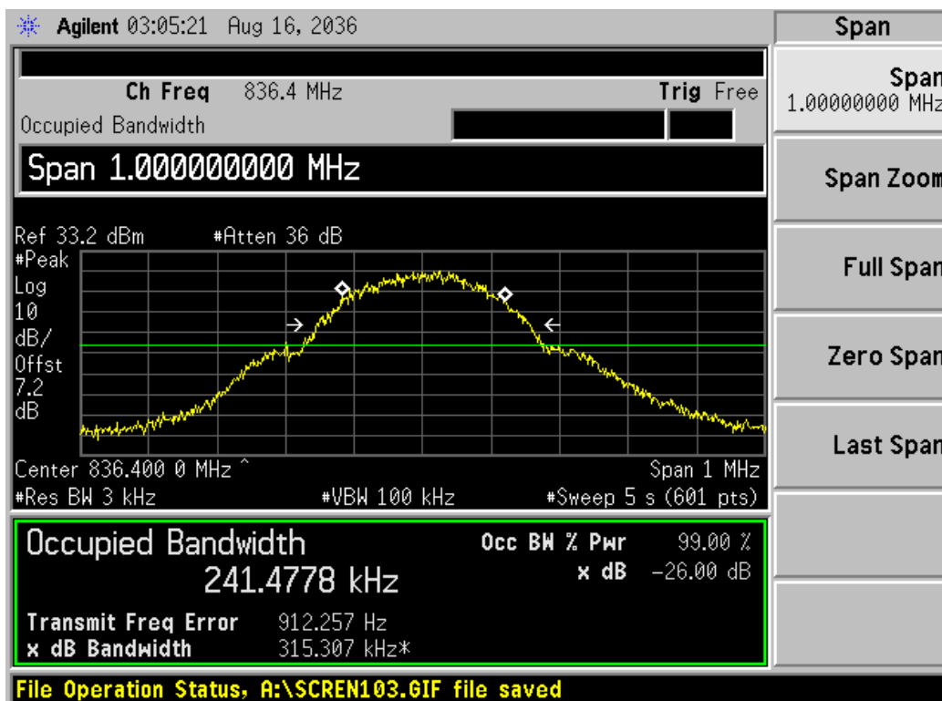
Channel 189
