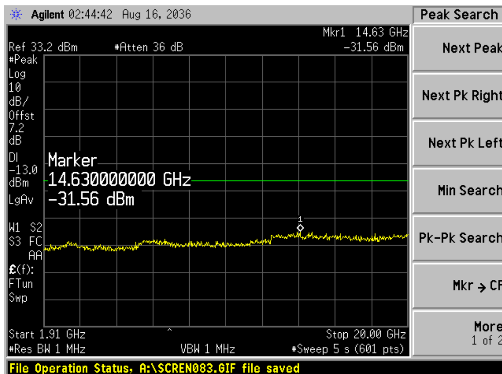
Channel 661, 1910MHz~20GHz
