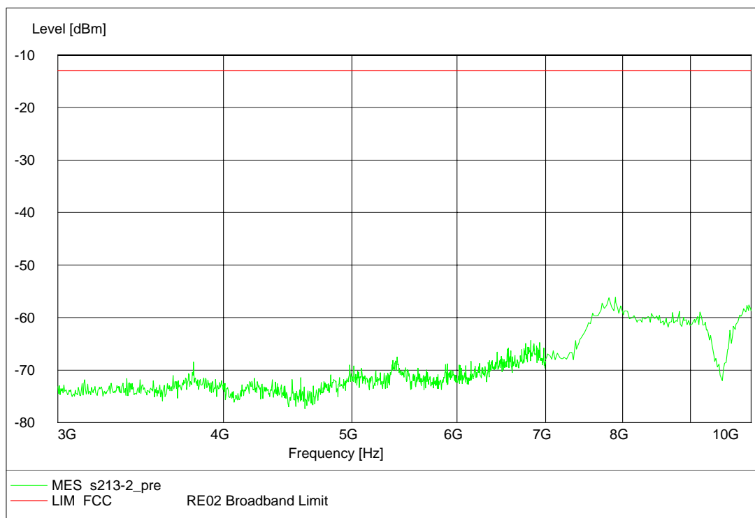
Channel 189, 3GHz~10GHz
