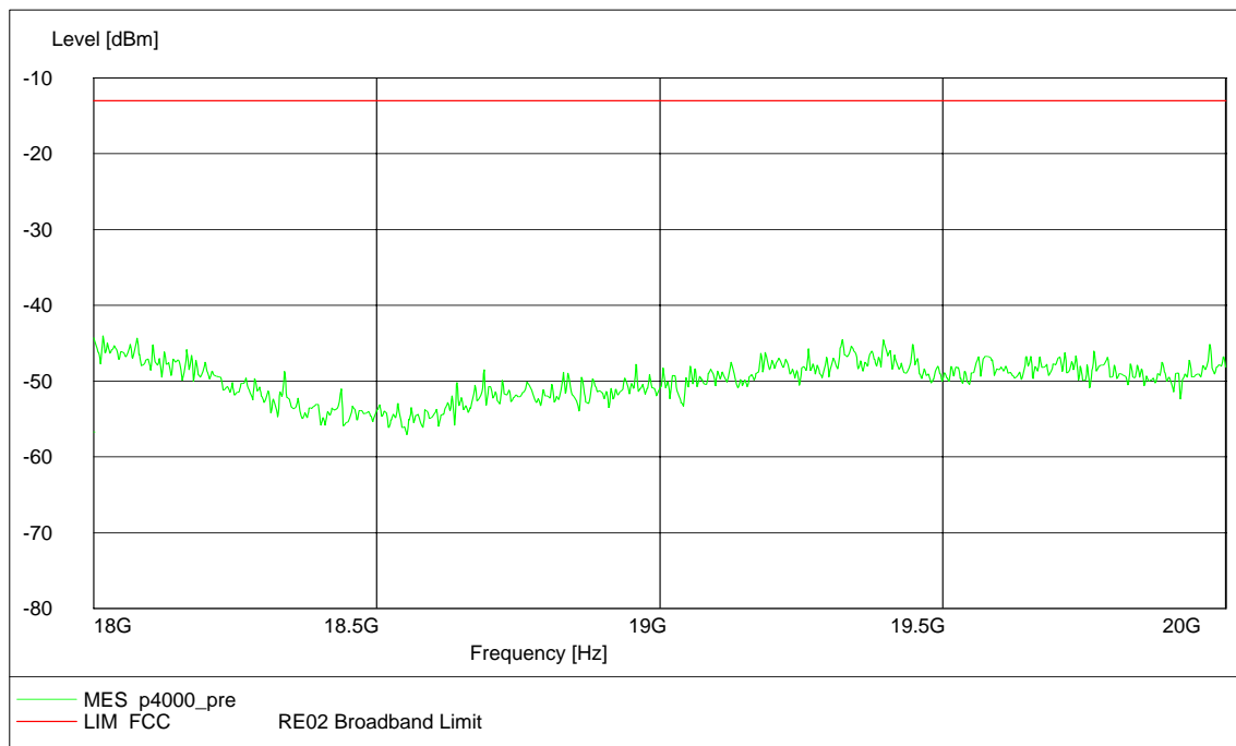
Channel 661, 18GHz~20GHz
