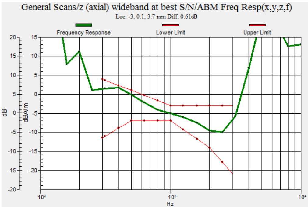
Graph 2 : GSM 850(CH 190) Frequency Response
