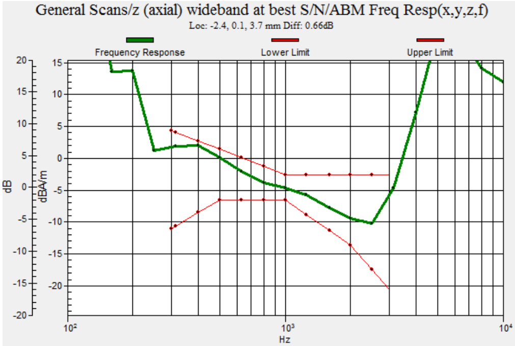
Graph 1 : GSM 850 (CH 128) Frequency Response
