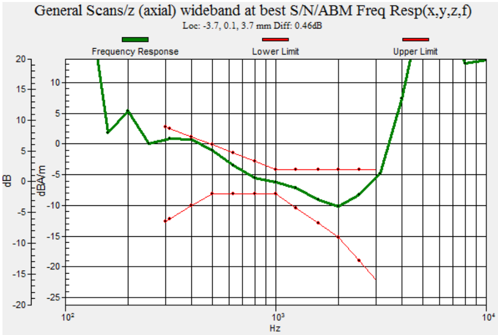
Graph 9 : WCDMA 850 (CH 4233) Frequency Response
