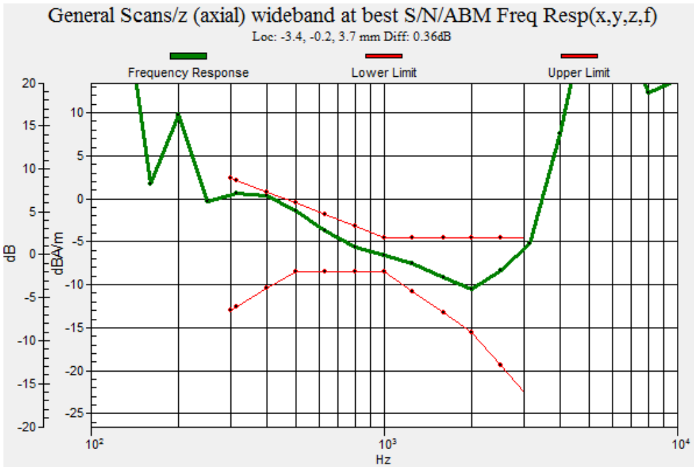
Graph 10 : WCDMA 1900 (CH 9262) Frequency Response
