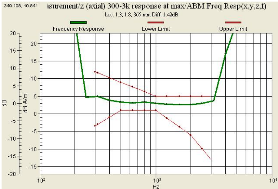
Graph 20 : WCDMA 850(CH 4183) Frequency Response (Slide up)
