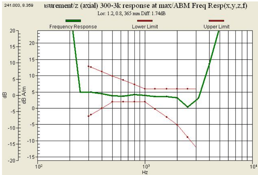
Graph 5 : GSM 1900 (CH 661) Frequency Response (Slide down)
