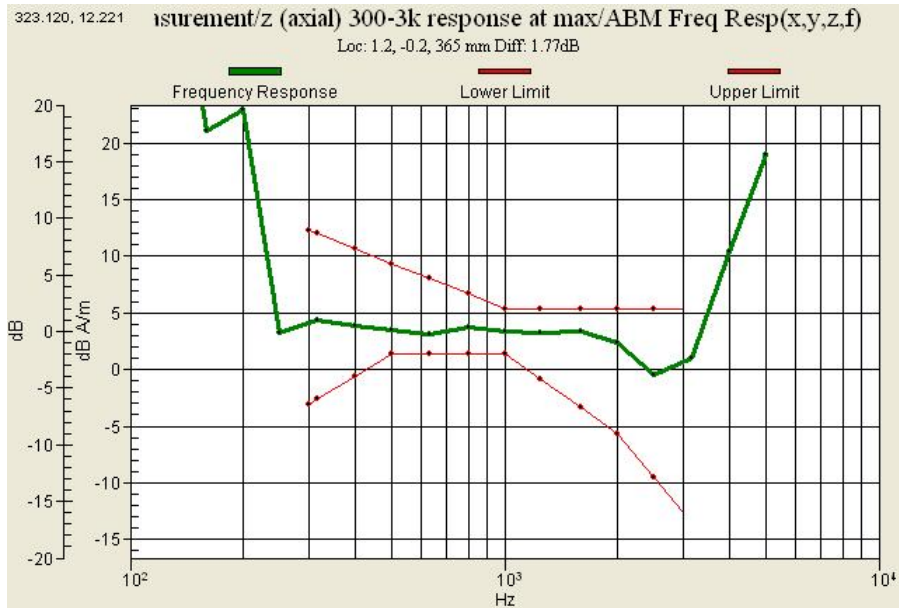
Graph 15 : GSM 850 (CH 251) Frequency Response (Slide up)
