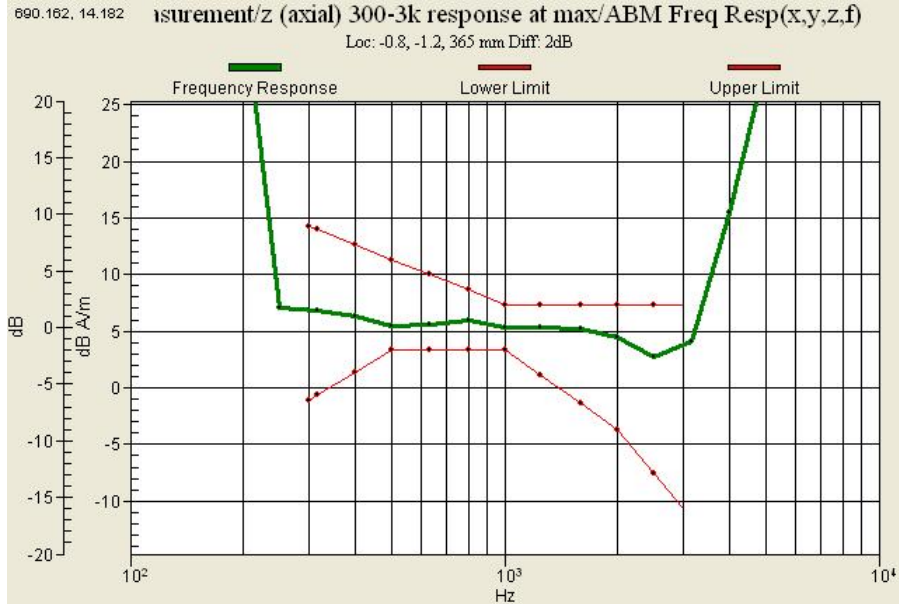
Graph 1 : GSM 850 (CH 128) Frequency Response (Slide down)
