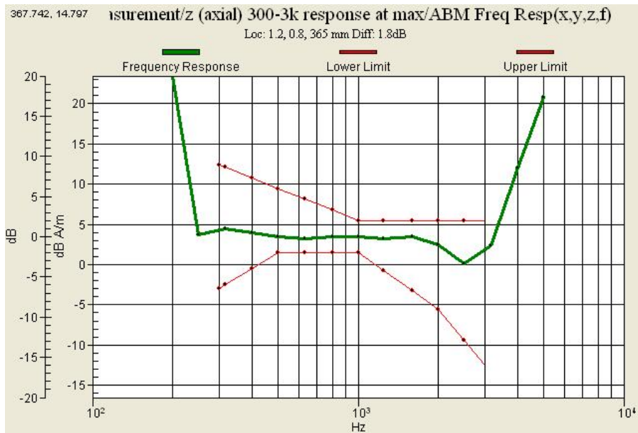
Graph 16 : GSM 1900(CH 512) Frequency Response (Slide up)
