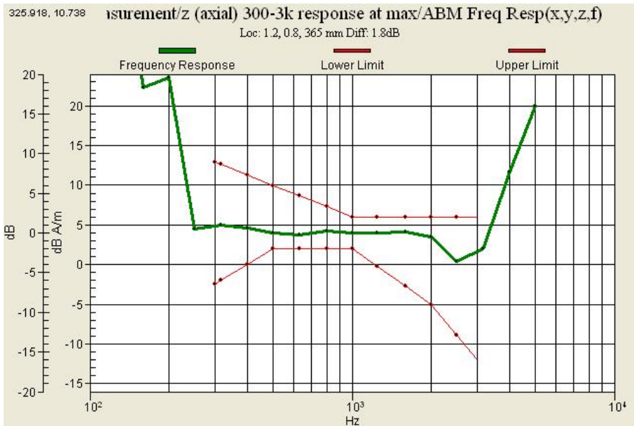
Graph 18 : GSM 1900 (CH 810) Frequency Response (Slide up)
