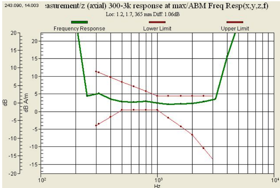
Graph 22 : WCDMA 1900 (CH 9262) Frequency Response (Slide up)
