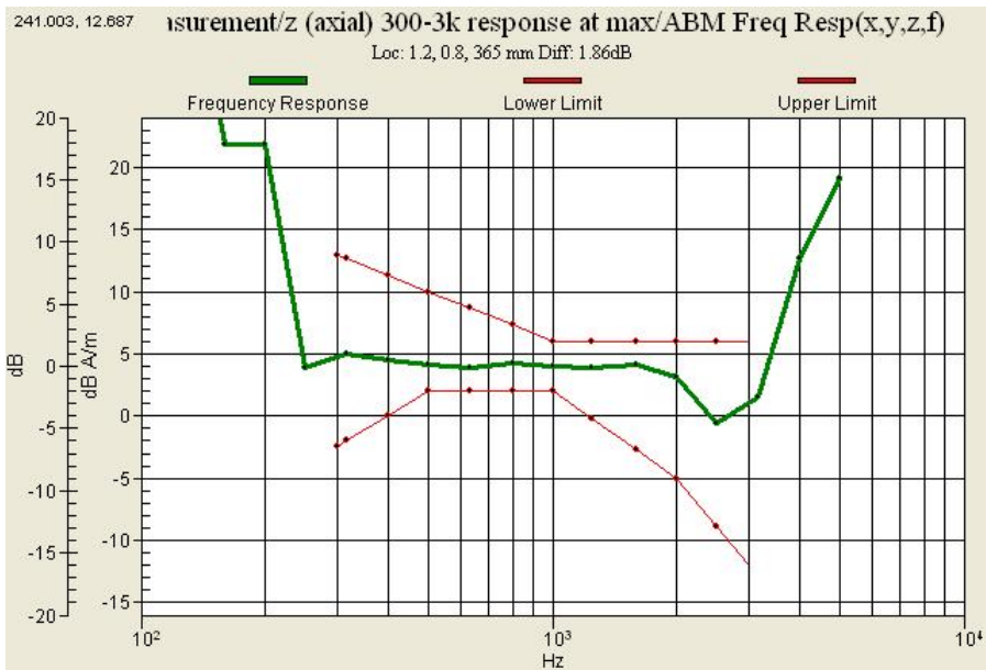
Graph 14 : GSM 850(CH 190) Frequency Response (Slide up)
