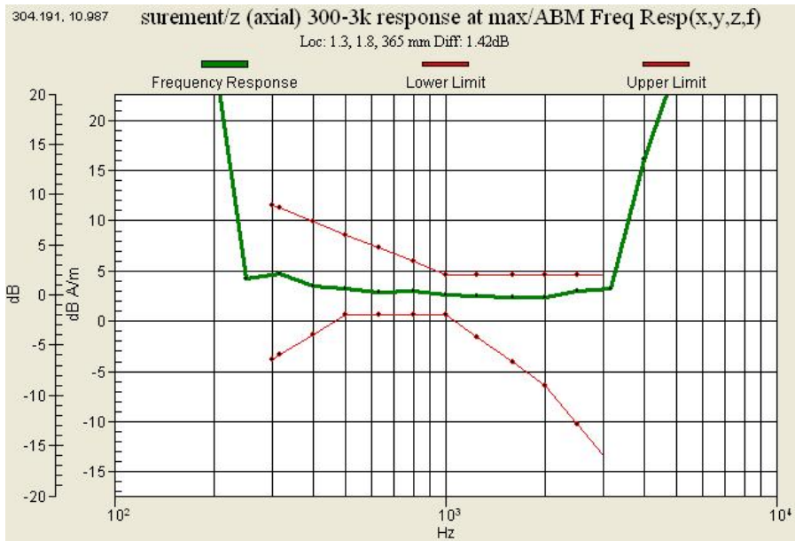
Graph 19 : WCDMA 850 (CH 4132) Frequency Response (Slide up)
