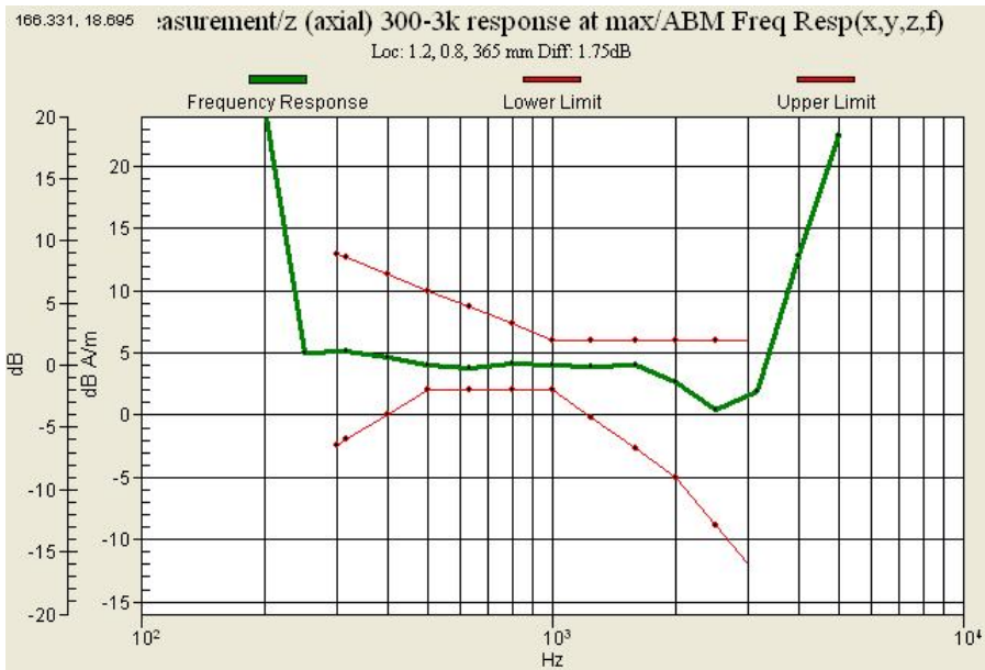
Graph 13 : GSM 850 (CH 128) Frequency Response (Slide up)
