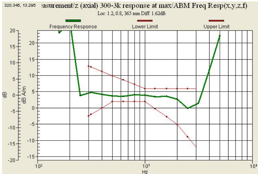
Graph 6 : GSM 1900 (CH 810) Frequency Response (Slide down)
