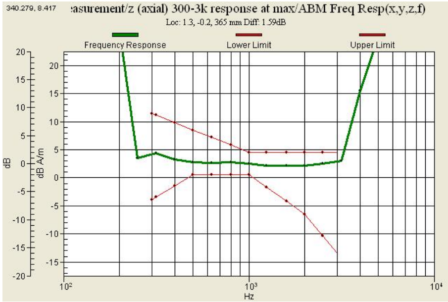
Graph 11 : WCDMA 1900 (CH 9400) Frequency Response (Slide down)
