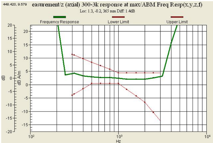
Graph 24 : WCDMA 1900 (CH 9583) Frequency Response (Slide up)
