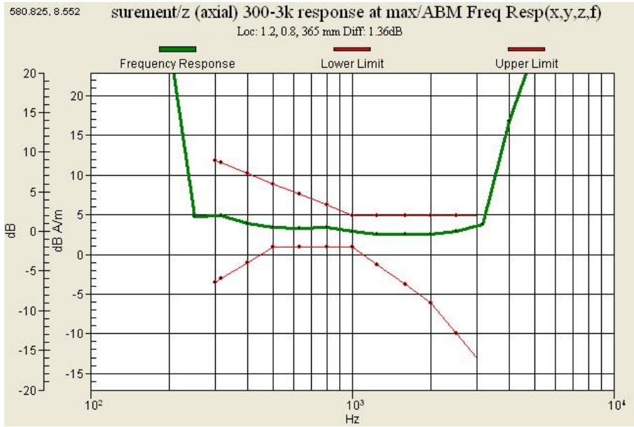
Graph 7 : WCDMA 850 (CH 4132) Frequency Response (Slide down)
