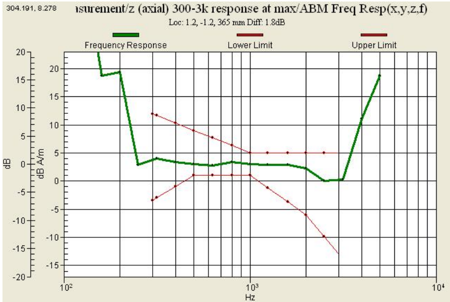
Graph 17 : GSM 1900 (CH 661) Frequency Response (Slide up)
