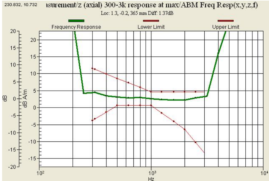
Graph 10 : WCDMA 1900 (CH 9262) Frequency Response (Slide down)
