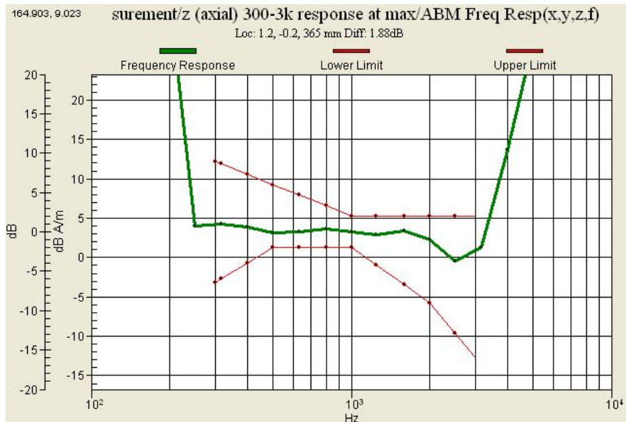
Graph 2 : GSM 850(CH 190) Frequency Response (Slide down)
