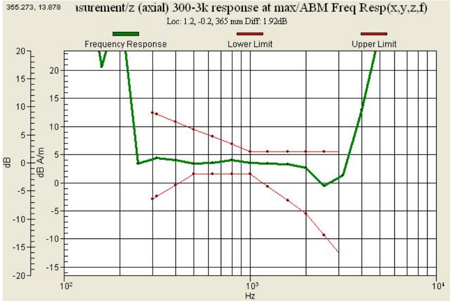
Graph 3 : GSM 850 (CH 251) Frequency Response (Slide down)
