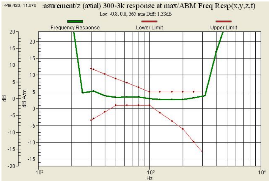
Graph 8 : WCDMA 850(CH 4183) Frequency Response (Slide down)
