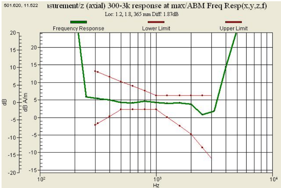
Graph 4 : GSM 1900(CH 512) Frequency Response (Slide down)
