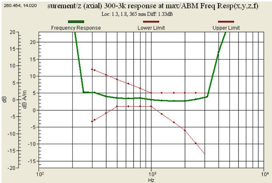
Graph 12 : WCDMA 1900 (CH 9583) Frequency Response (Slide down)
