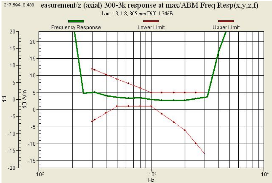
Graph 23 : WCDMA 1900 (CH 9400) Frequency Response (Slide up)
