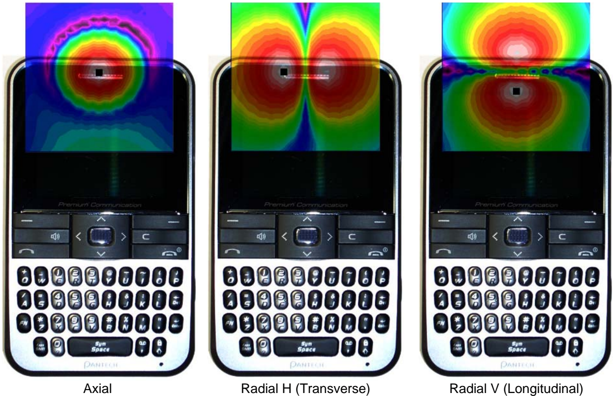
Figure 12-3 T-Coil Scan Overlay Magnetic Field Distributions
