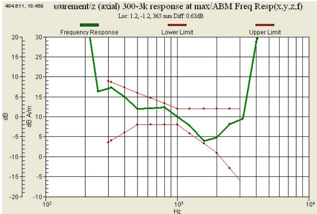
Graph 11 : GSM 1900 (CH 661) Frequency Response Slide down
