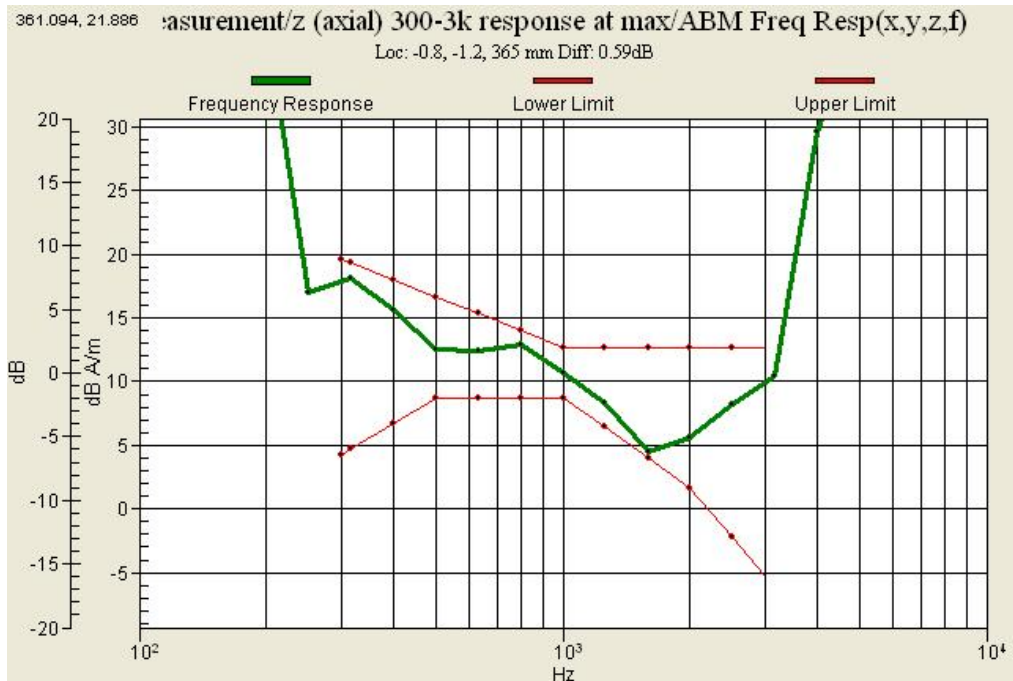
Graph 12 : GSM 1900 (CH 810) Frequency Response Slide down
