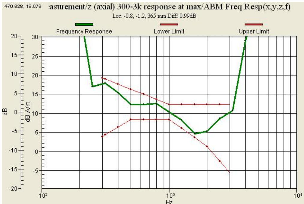
Graph 22 : GSM 1900 (CH 512) Frequency Response Slide up
