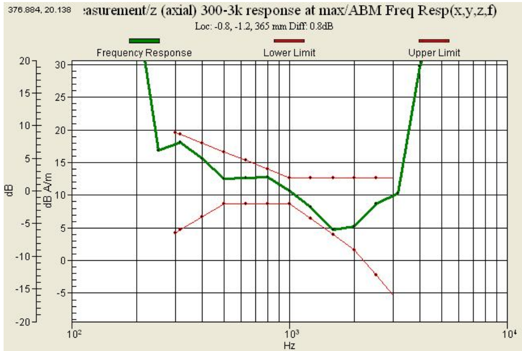
Graph 7 : GSM850 (CH 128) Frequency Response Slide down
