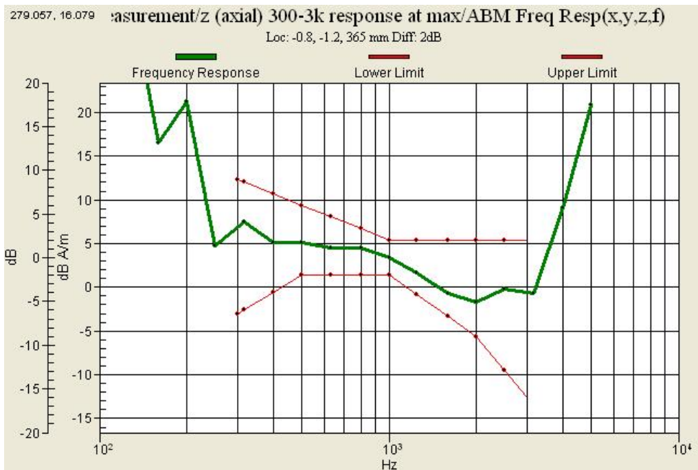
Graph 14 : CDMA 835 (CH 384) Frequency Response Slide up
