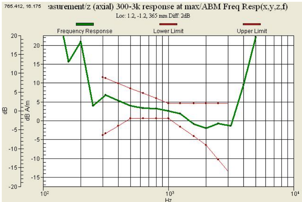
Graph 16 : PCS 1900 (CH 25) Frequency Response Slide up
