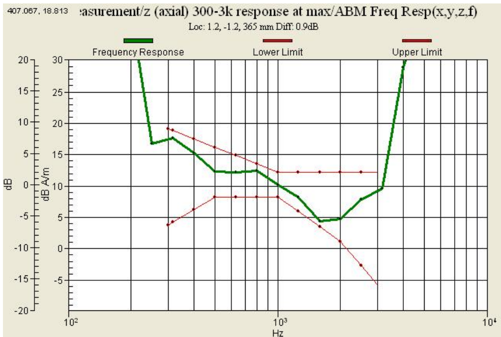
Graph 20 : GSM 850 (CH 190) Frequency Response Slide up
