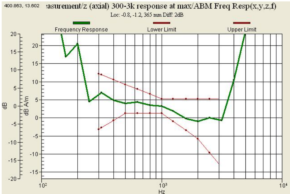
Graph 15 : CDMA 835 (CH 777) Frequency Response Slide up
