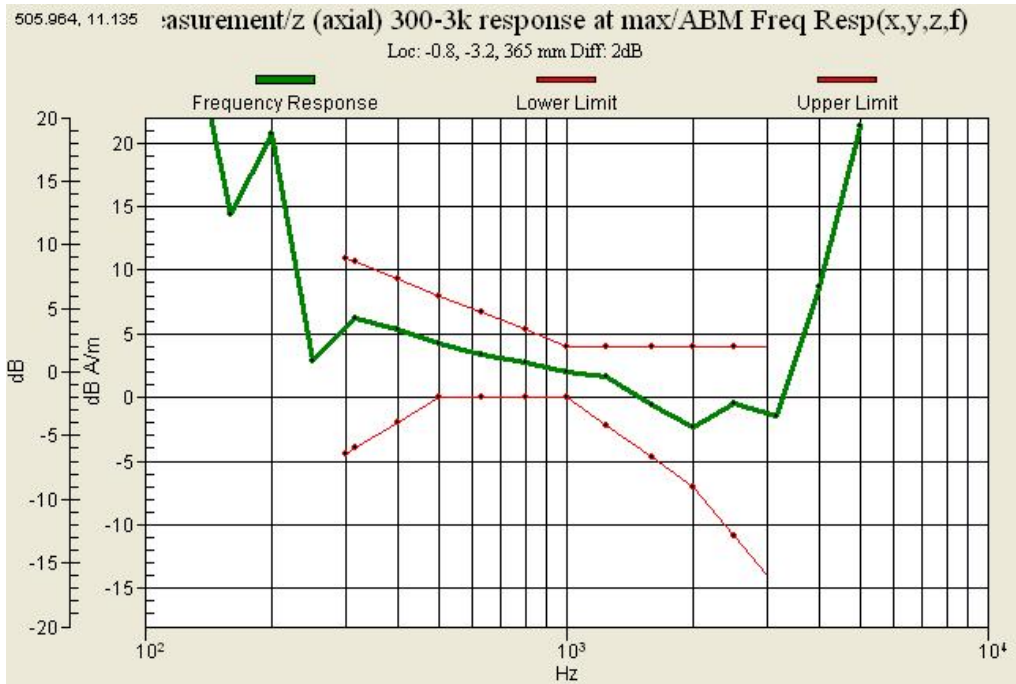
Graph 13 : CDMA 835 (CH 1013) Frequency Response Slide up
