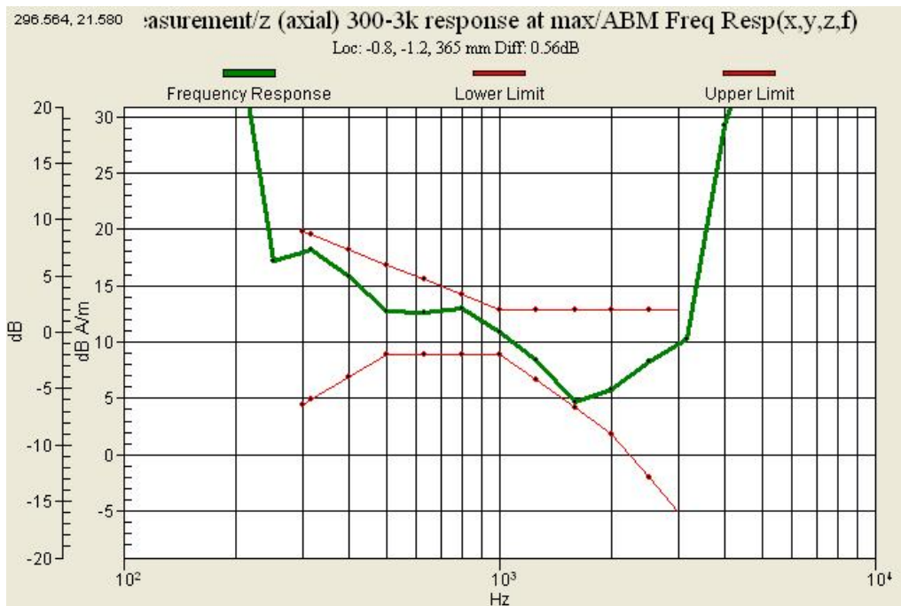
Graph 8 : GSM850 (CH 190) Frequency Response Slide down
