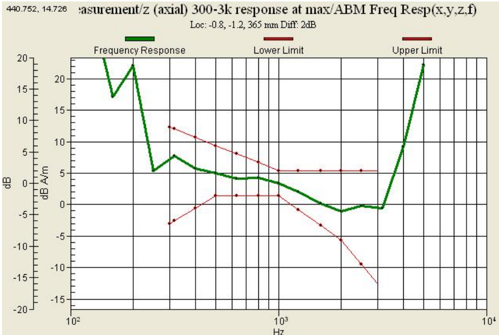
Graph 18 : PCS 1900 (CH 1175) Frequency Response Slide up
