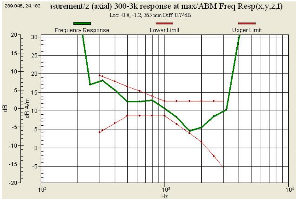
Graph 9 : GSM850 (CH 251) Frequency Response Slide down
