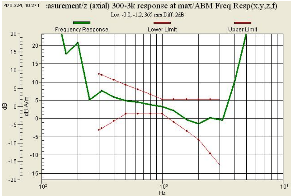
Graph 17 : PCS 1900 (CH 600) Frequency Response Slide up
