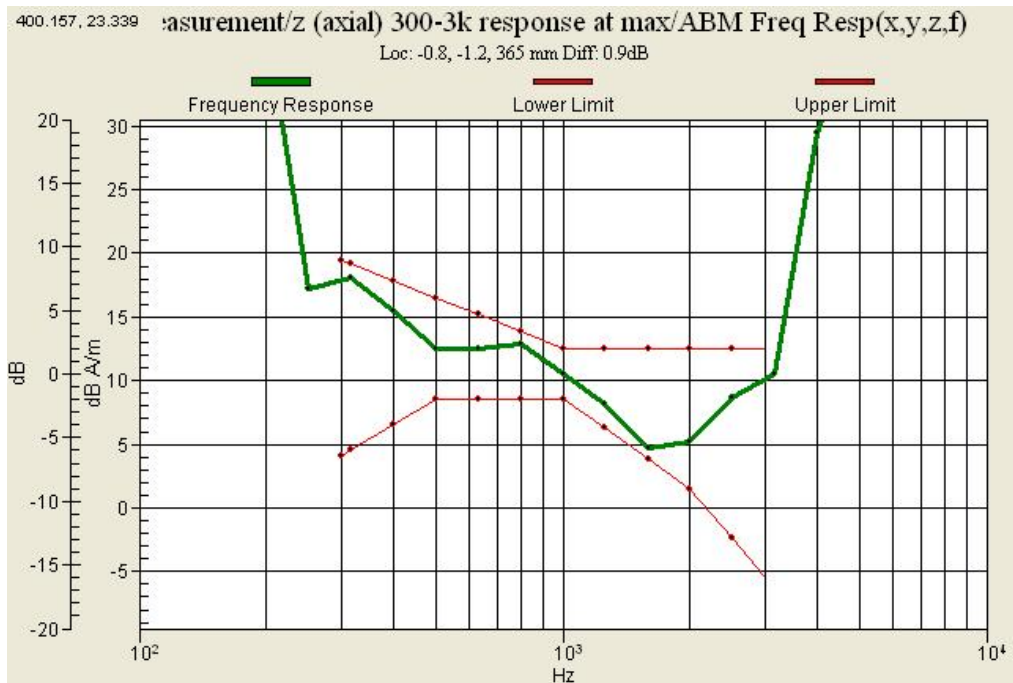
Graph 10 : GSM 1900 (CH 512) Frequency Response Slide down
