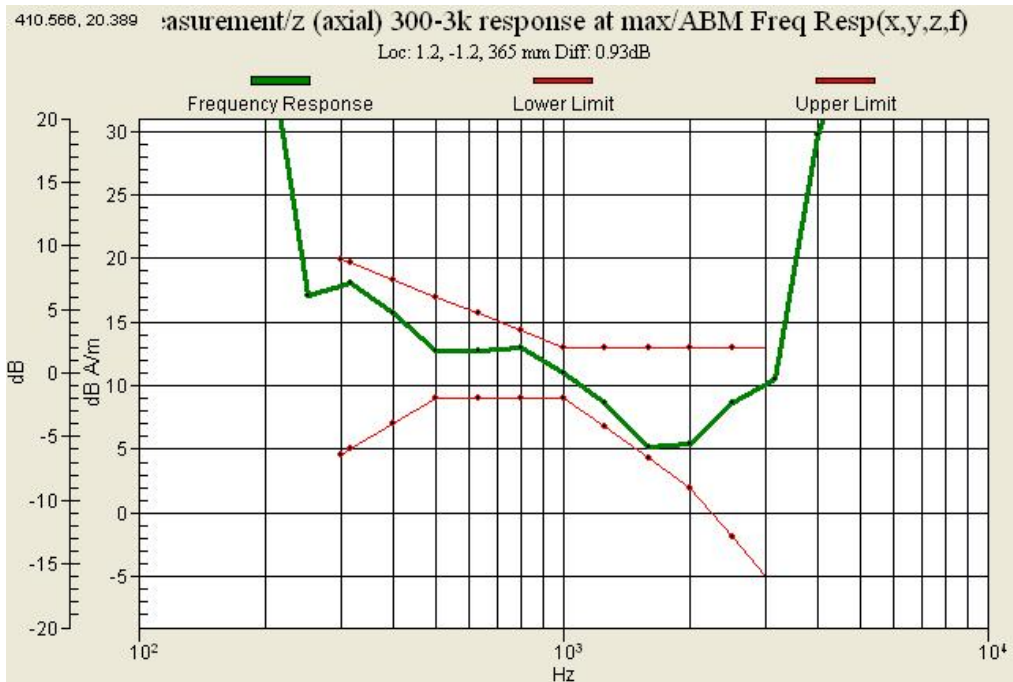
Graph 21 : GSM 850 (CH 251) Frequency Response Slide up
