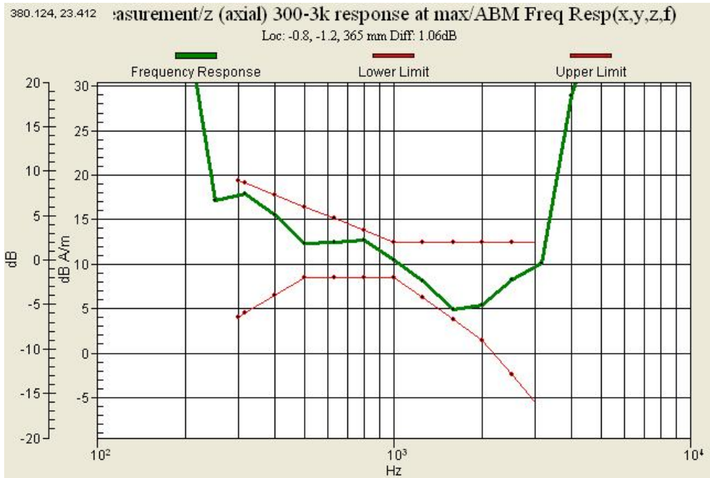
Graph 19 : GSM 850 (CH 128) Frequency Response Slide up
