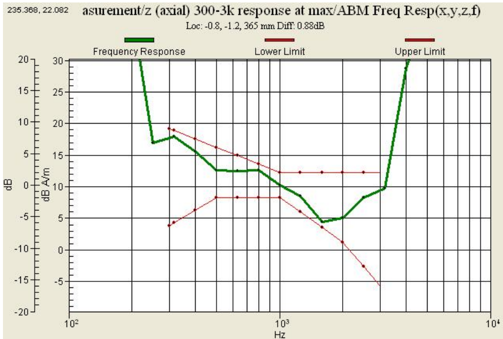
Graph 24 : GSM 1900 (CH 810) Frequency Response Slide up
