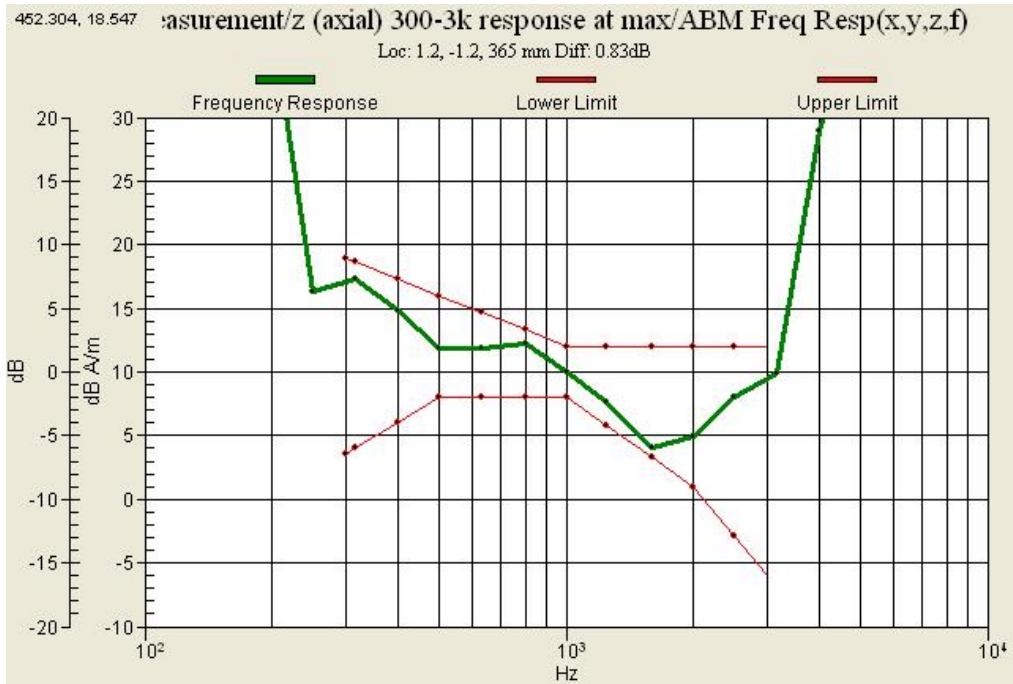
Graph 23 : GSM 1900 (CH 661) Frequency Response Slide up
