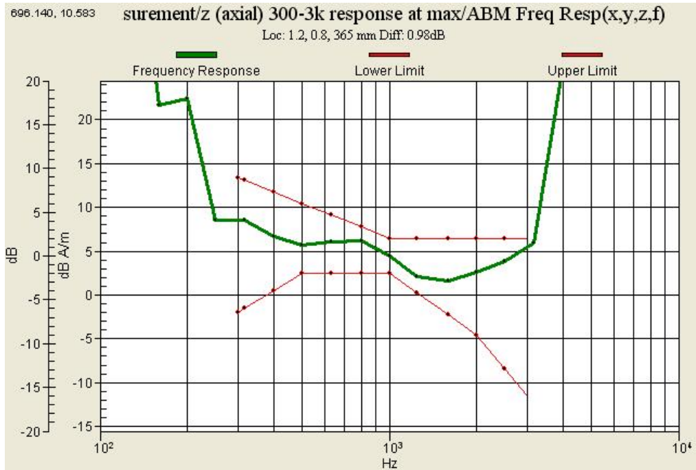
Graph 8 : PCS 1900 (CH 25) Frequency Response (wireless charging cover)
