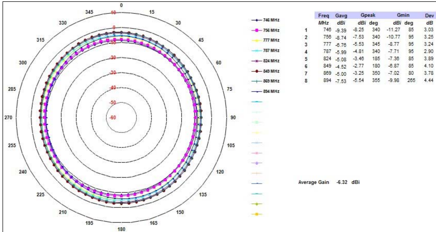
H Plane _ LTE Band 13/Cellular
