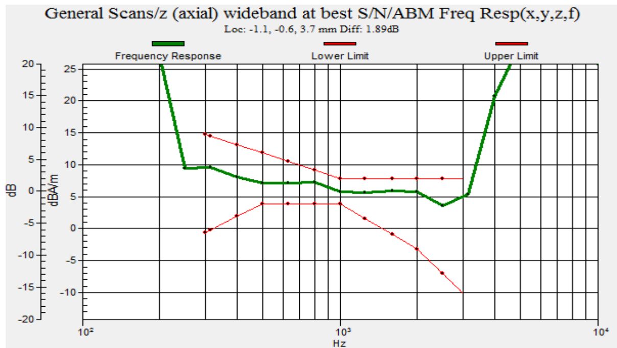
Graph 14 : GSM 1900 (CH 661) Frequency Response
