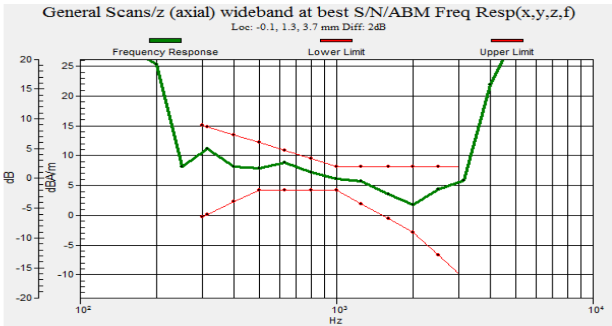
Graph 2 : CDMA (CH 384) Frequency Response
