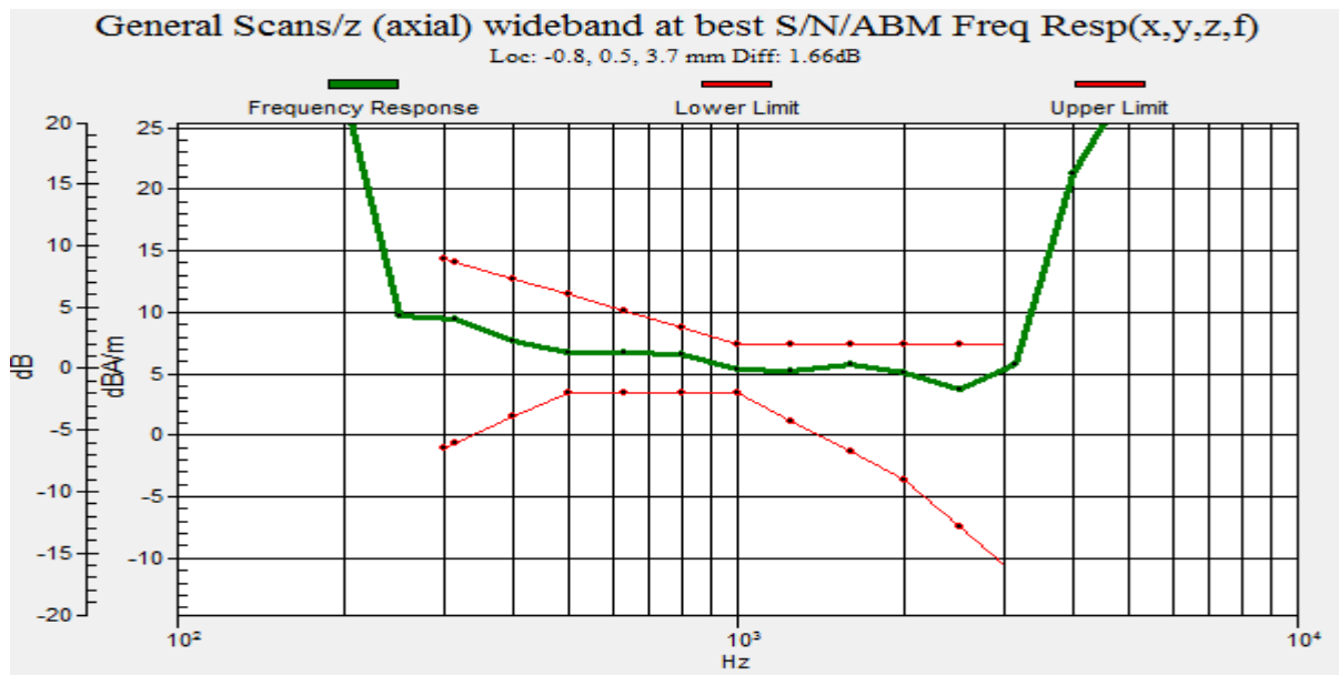
Graph 9 : GSM 850 (CH 128) Frequency Response
