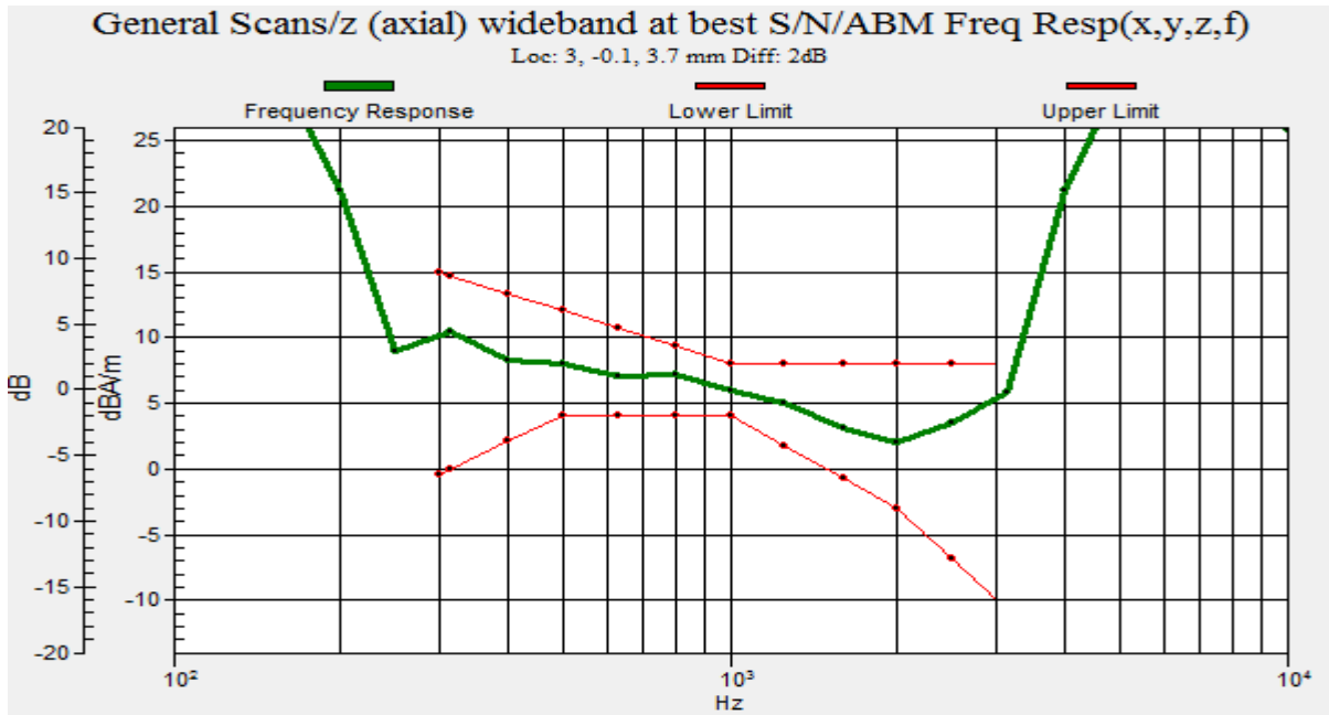
Graph 1 : CDMA (CH 1013) Frequency Response
