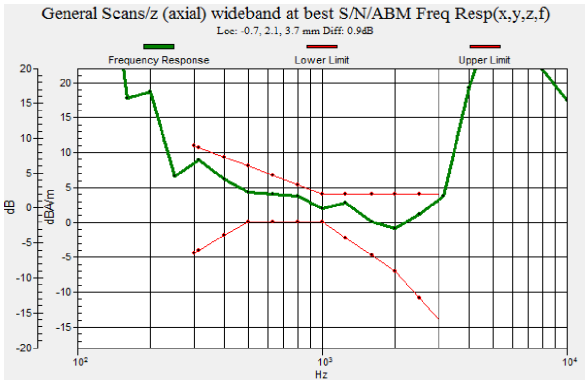
Graph 8 : PCS CDMA (CH 600) Frequency Response
