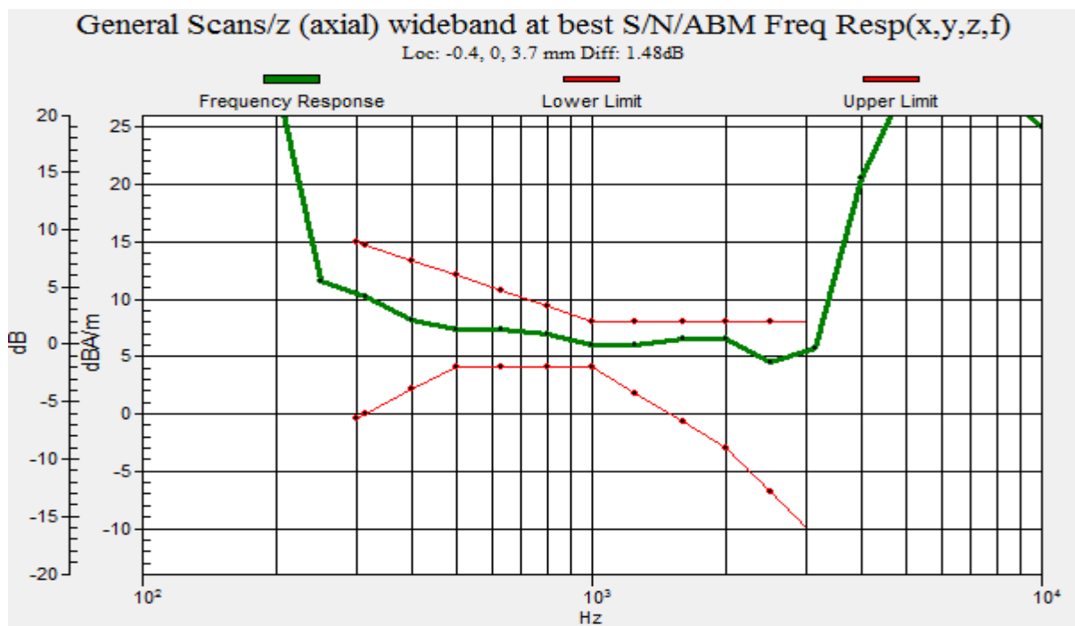
Graph 16 : GSM 1900 (CH 661) Frequency Response
