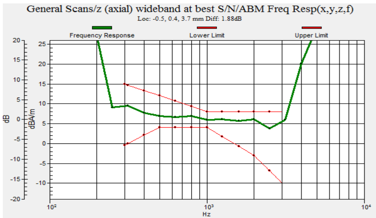
Graph 10 : GSM 850(CH 190) Frequency Response
