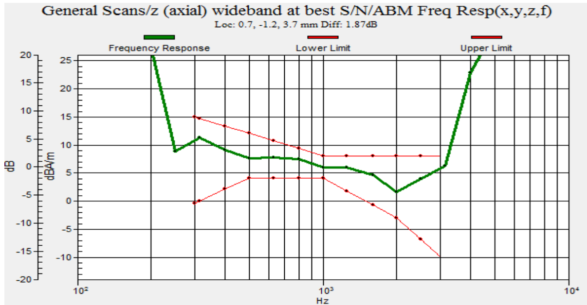
Graph 3 : CDMA (CH 777) Frequency Response
