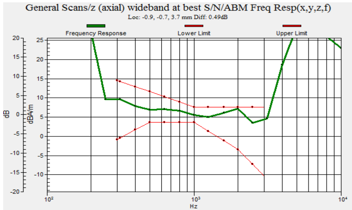
Graph 13 : GSM 1900 (CH 512) Frequency Response
