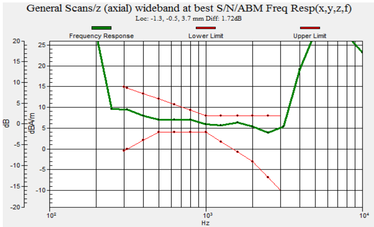
Graph 11 : GSM 850 (CH 251) Frequency Response
