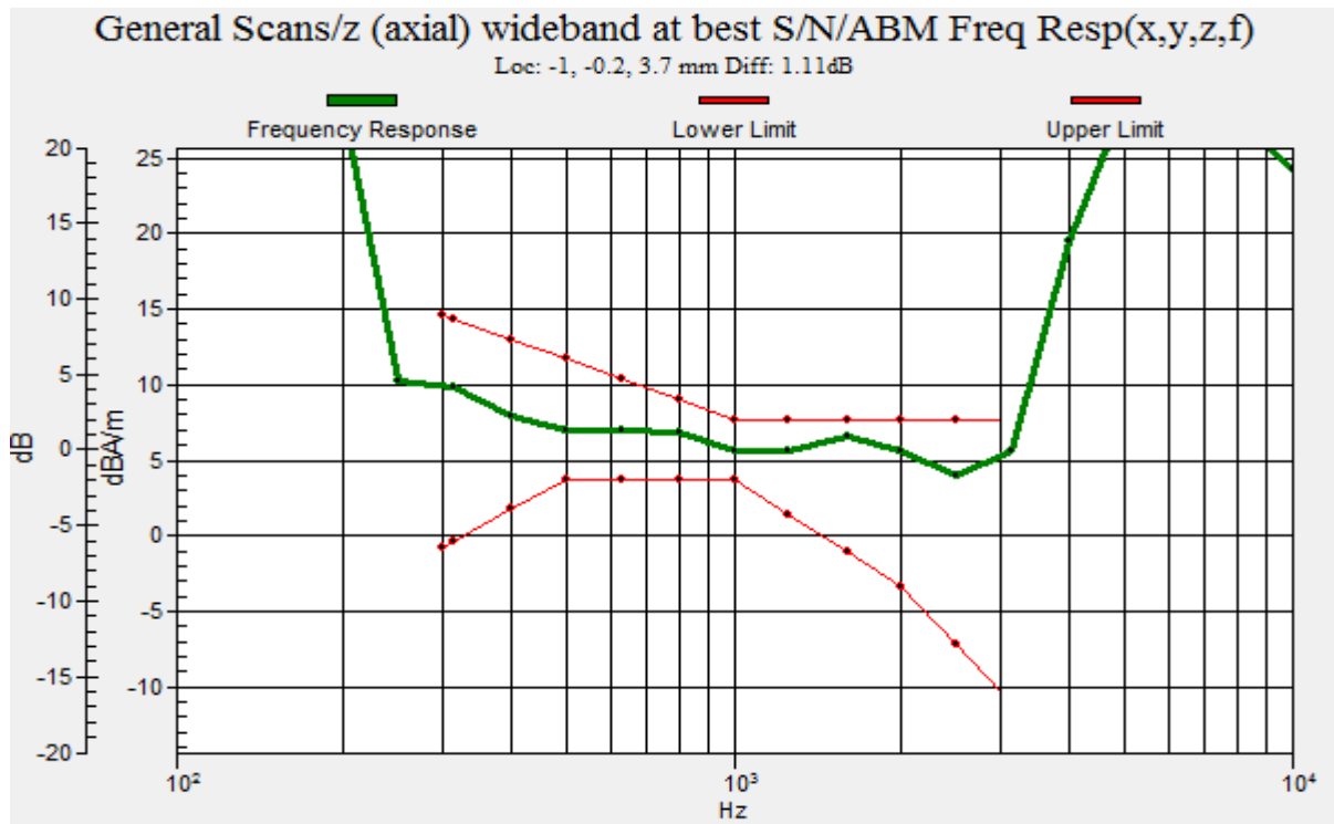
Graph 15 : GSM 1900 (CH 810) Frequency Response
