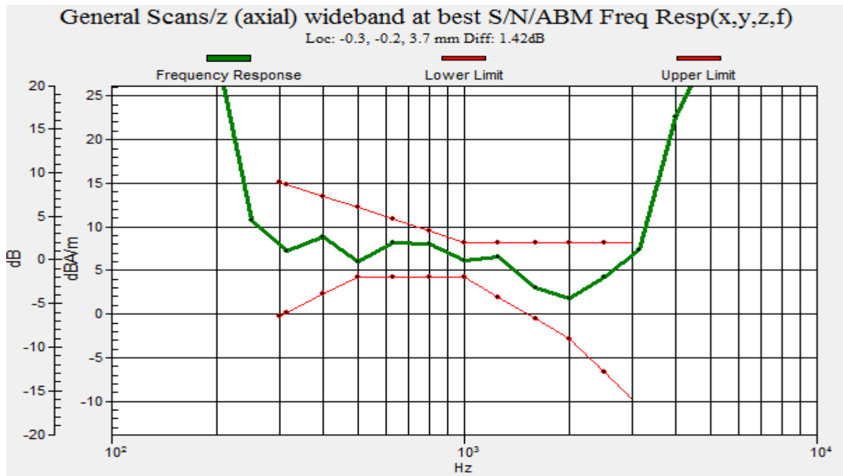
Graph 7 : PCS CDMA (CH 1175) Frequency Response
