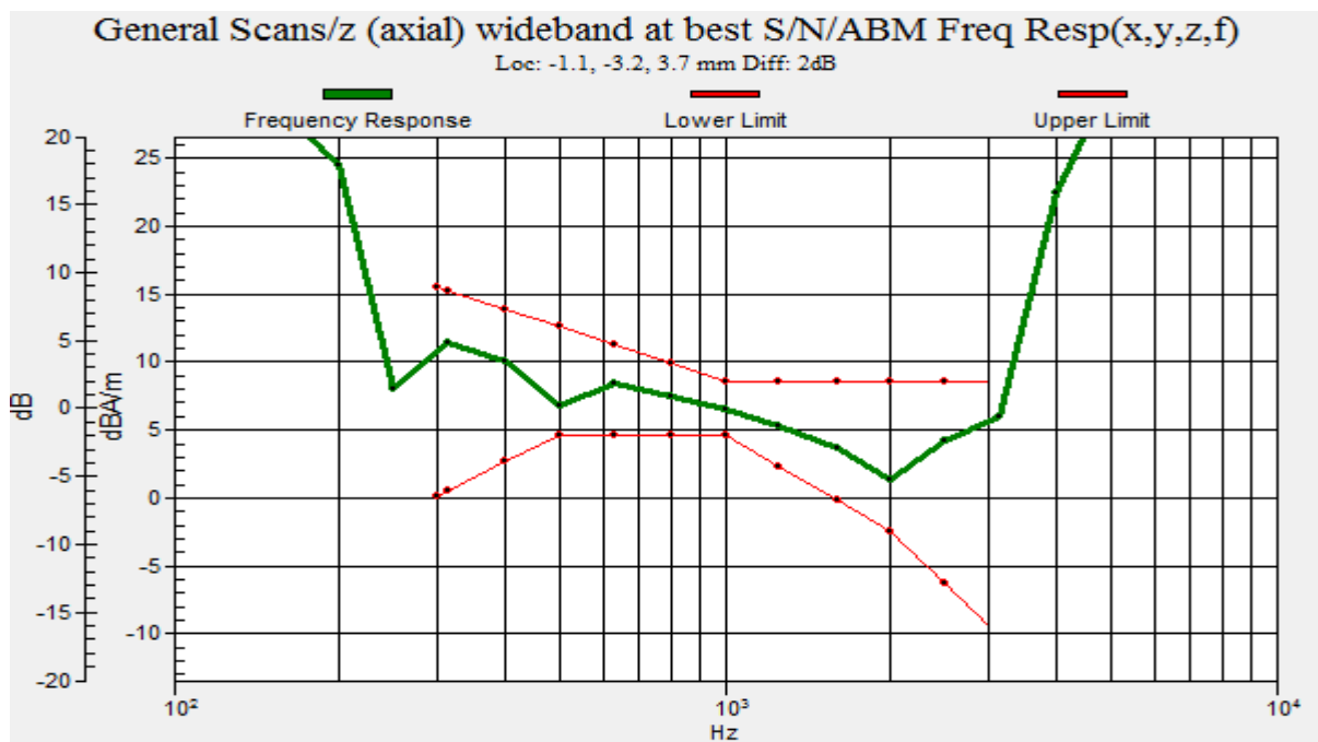
Graph 6 : PCS CDMA (CH 600) Frequency Response
