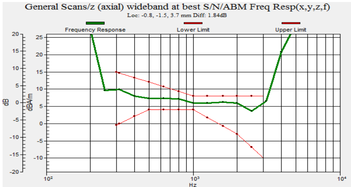
Graph 12 : GSM 850(CH 190) Frequency Response
