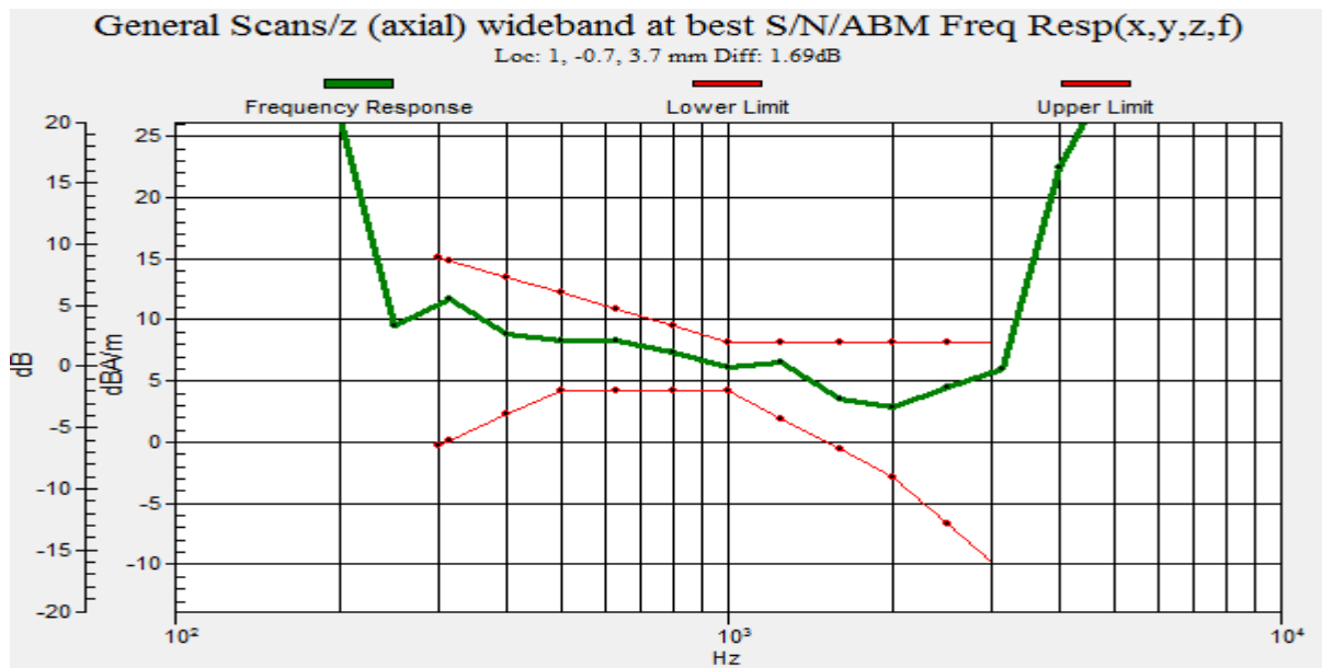
Graph 4 : CDMA (CH 384) Frequency Response
