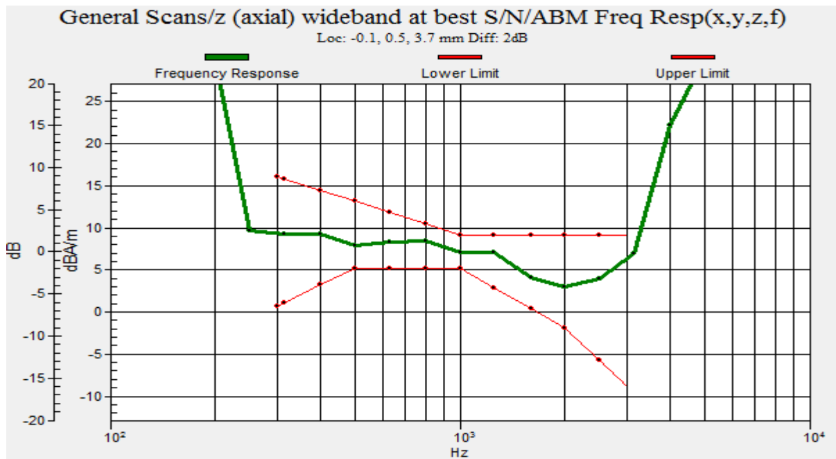
Graph 5 : PCS CDMA (CH 25) Frequency Response
