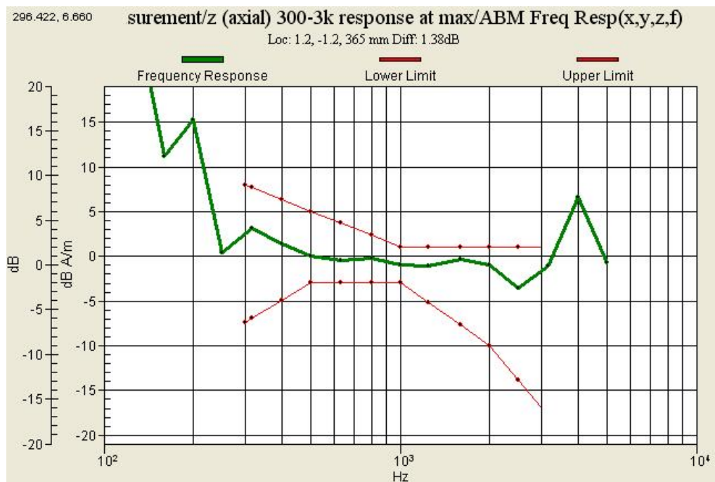
Graph 8 : GSM850 (CH 190) Frequency Response
