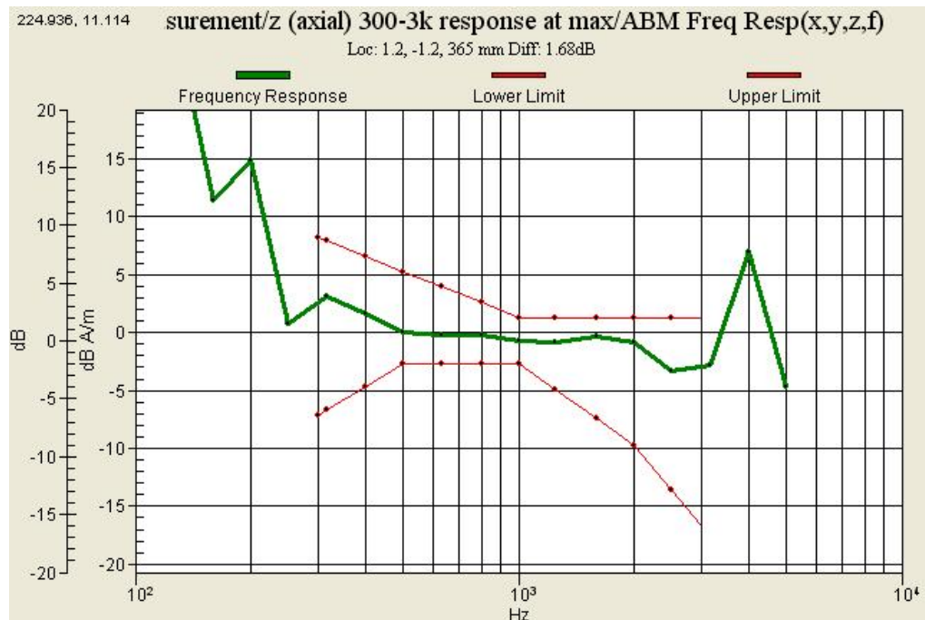
Graph 12 : GSM 1900 (CH 810) Frequency Response
