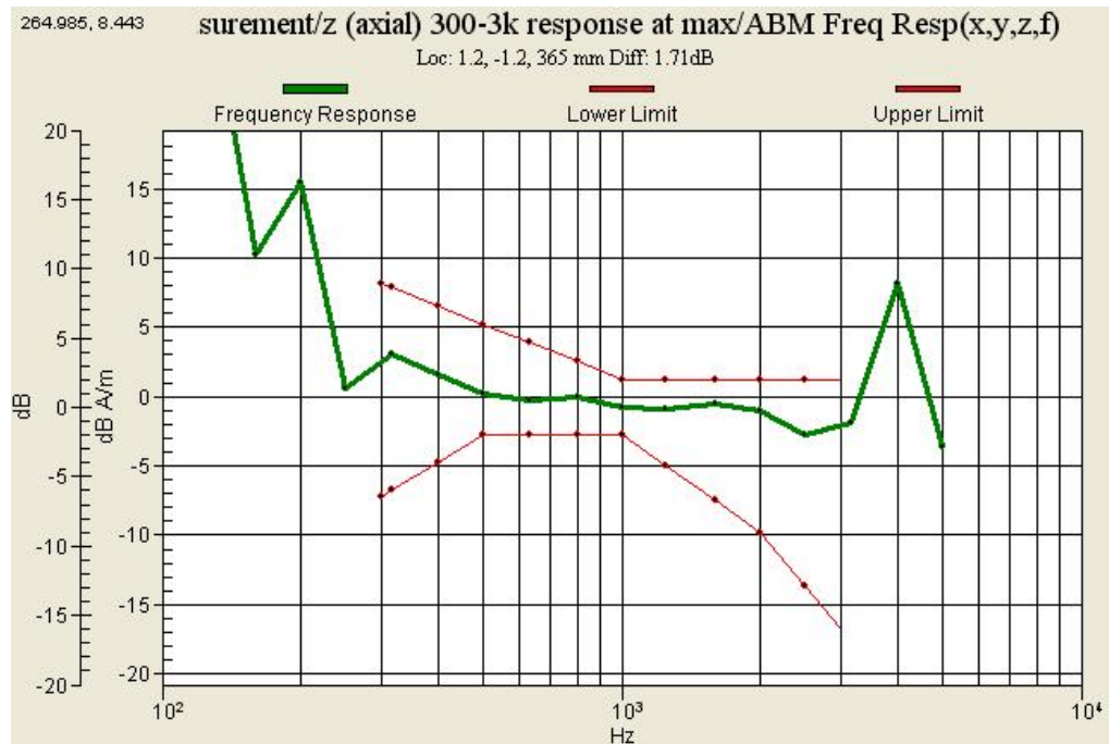
Graph 11 : GSM 1900 (CH 661) Frequency Response
