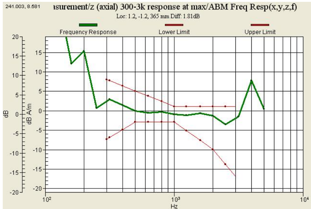
Graph 7 : GSM850 (CH 128) Frequency Response
