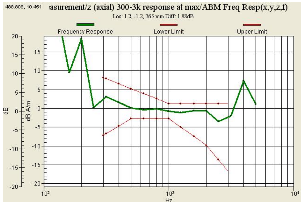
Graph 10 : GSM 1900 (CH 512) Frequency Response
