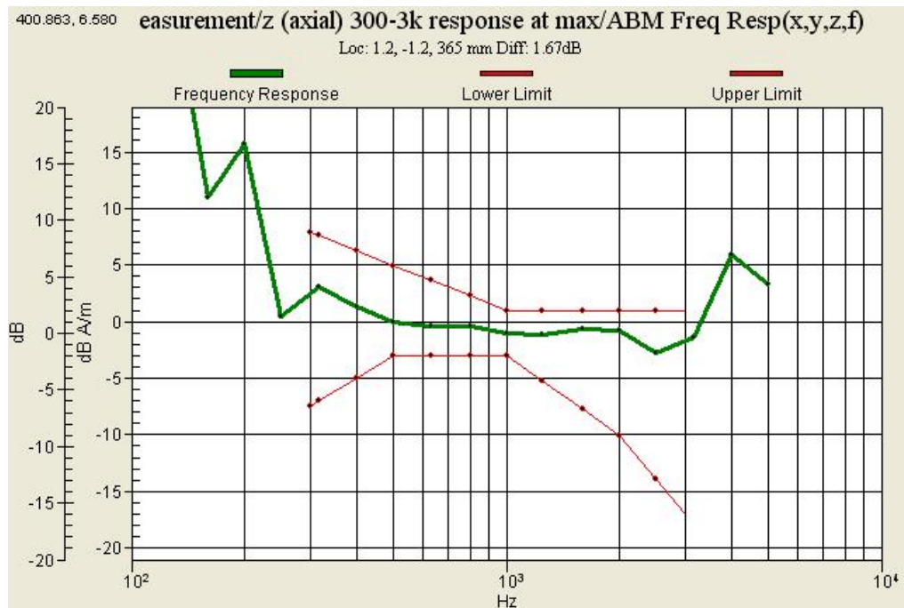
Graph 9 : GSM850 (CH 251) Frequency Response
