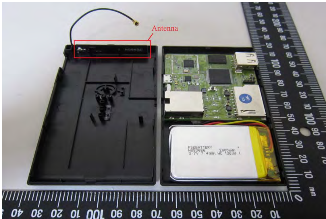
Antenna Location
