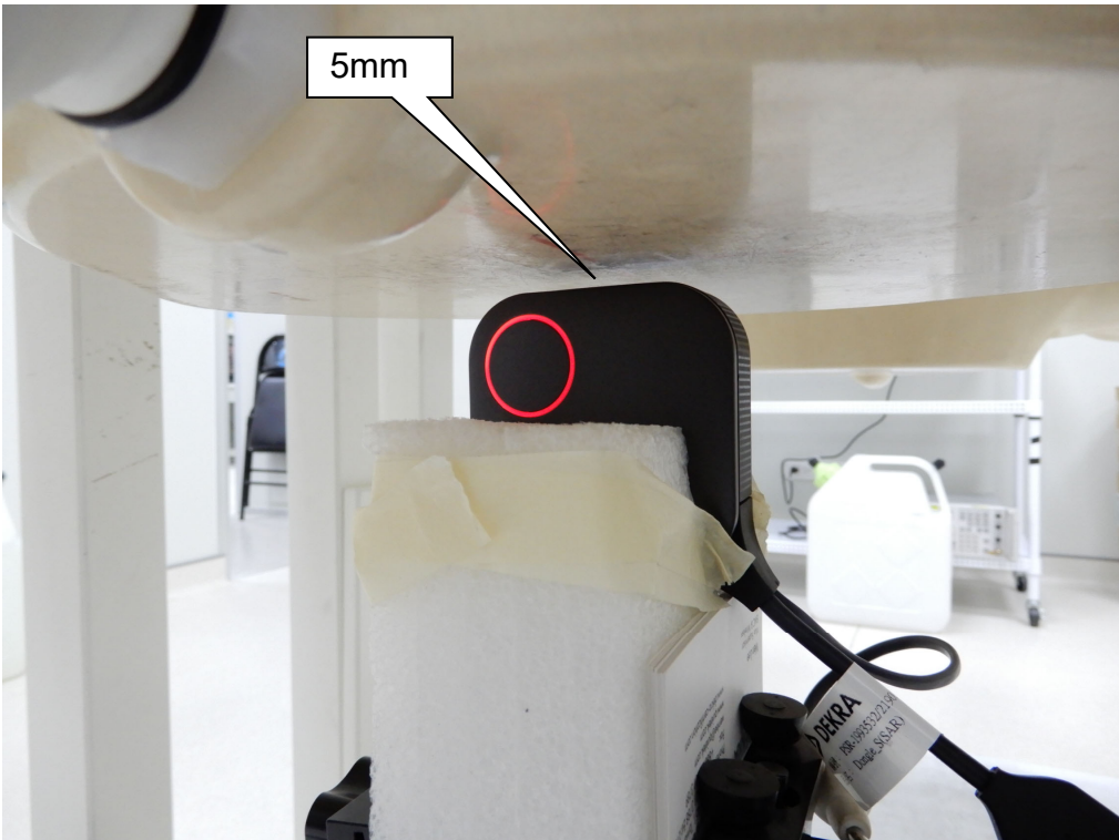
EUT Right-side_5mm
