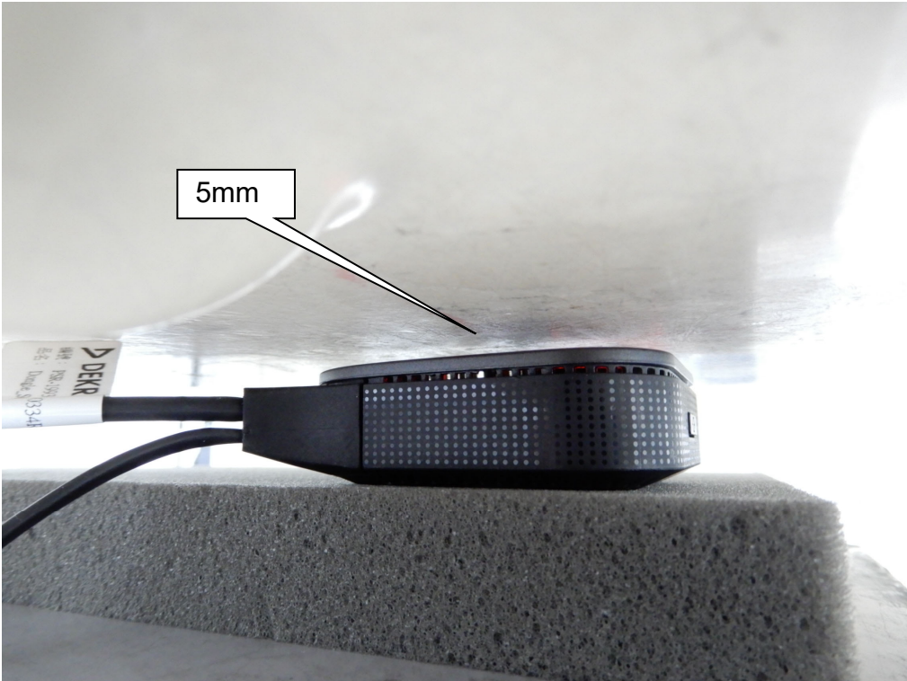
EUT Front_5mm
