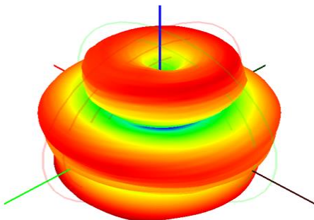
5700.0MHz H+V, Eff. 48.76%
