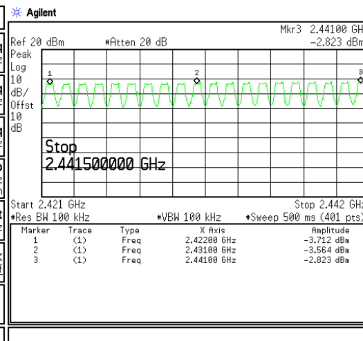
2422-2441MHz
