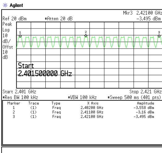
2402-2421MHz
