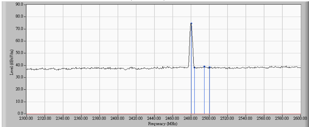
Figure Channel 78: (Horizontal)
