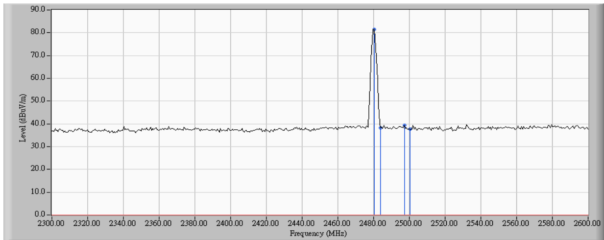
Figure Channel 78: (Vertical)
