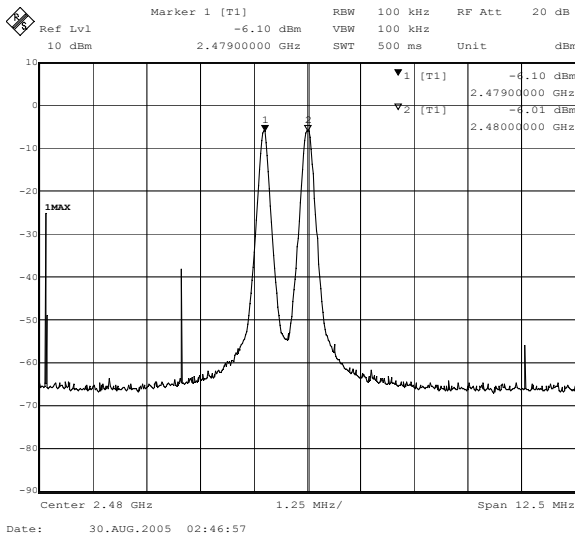
Channel 78 2480 MHz
