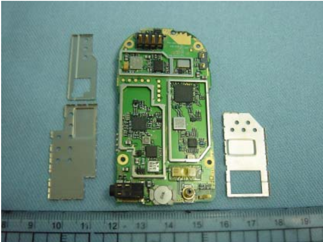
Internal of EUT --- 19
