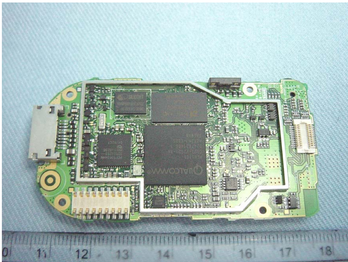
Internal of EUT --- 17
