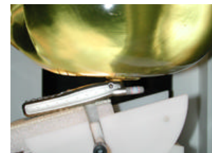
Fig. 19 Head SAR Test Setup
