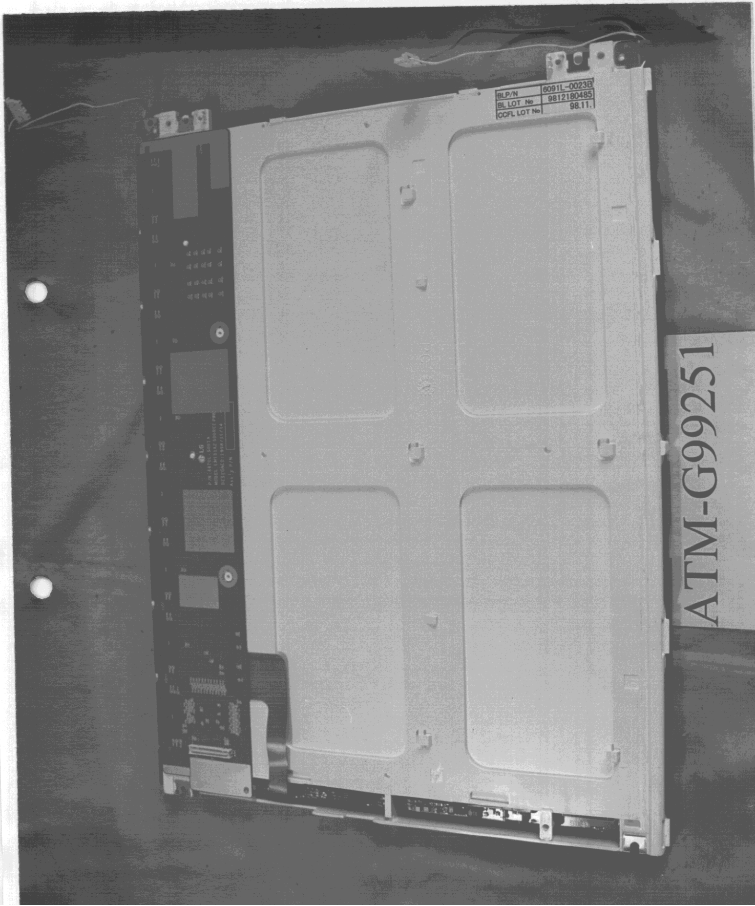
Figure 15 LCD Panel (Back Side)
