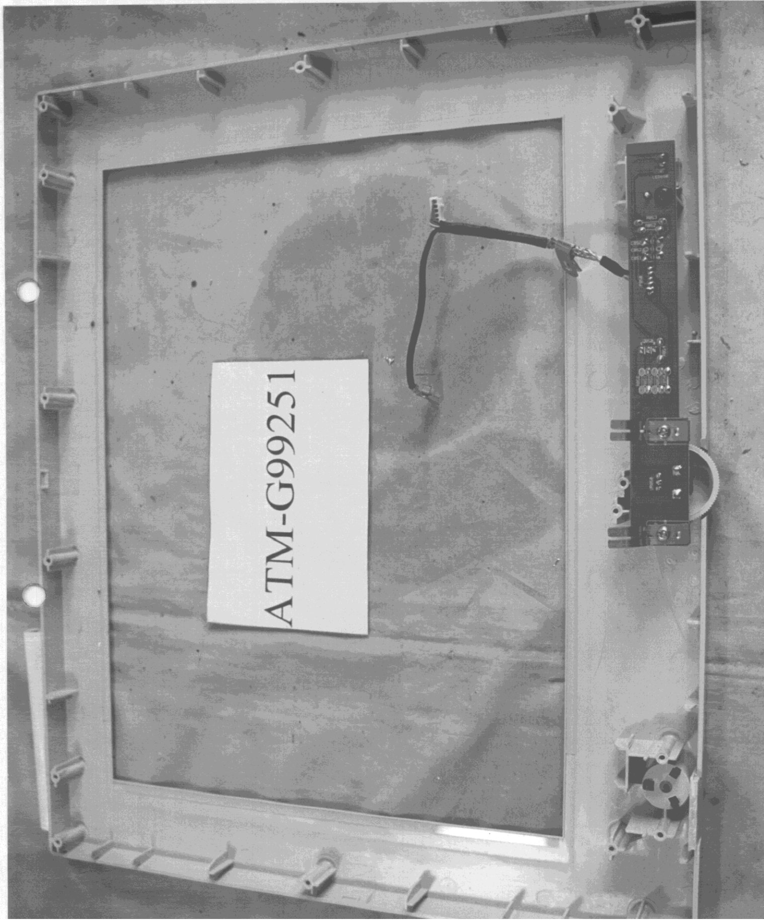
Figure 18 Front Cover (Internal View) & Control Board
