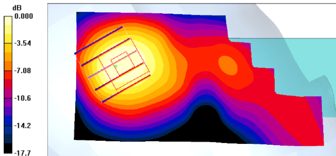
0 dB = 0.317mW/g
