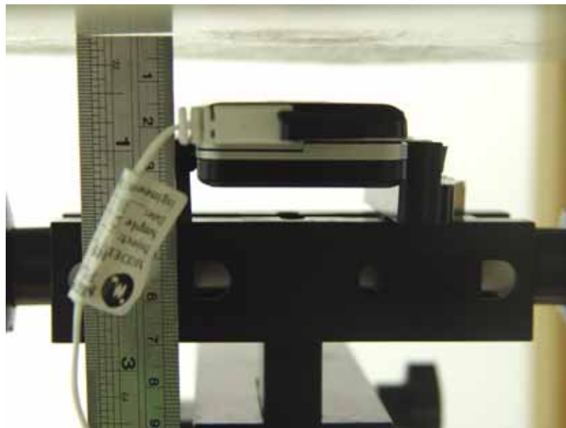
Fig. 9.12 Keypad Down with 1.5cm Gap
