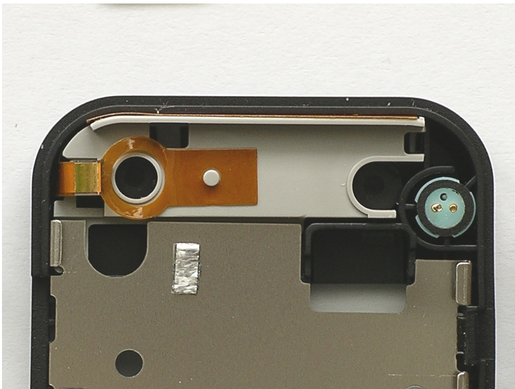
AF51 tri-band antenna (assembled)
