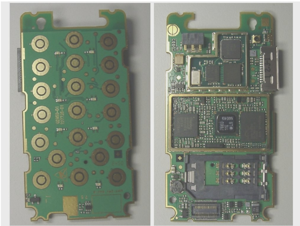
AF51 PCB (removed shieldings)
