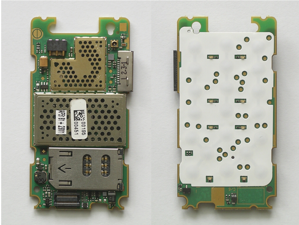
AF51 PCB (top and bottom view)
