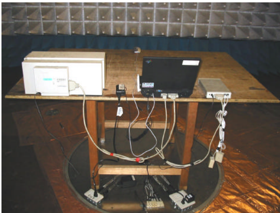
Rear View of the Test Configuration of Unintentional
