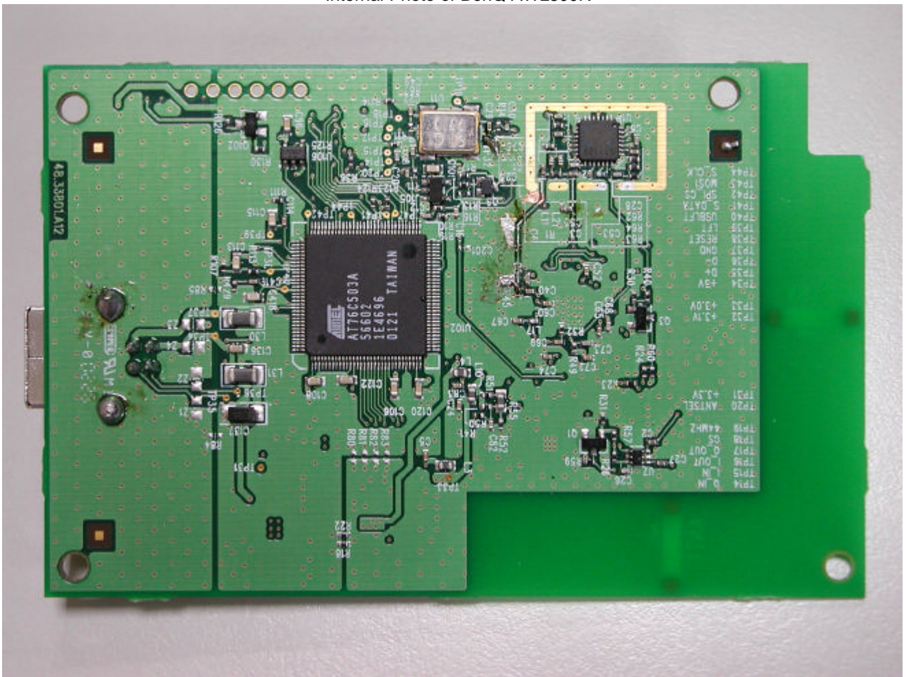
Internal Photo of BenQ AWL300R
