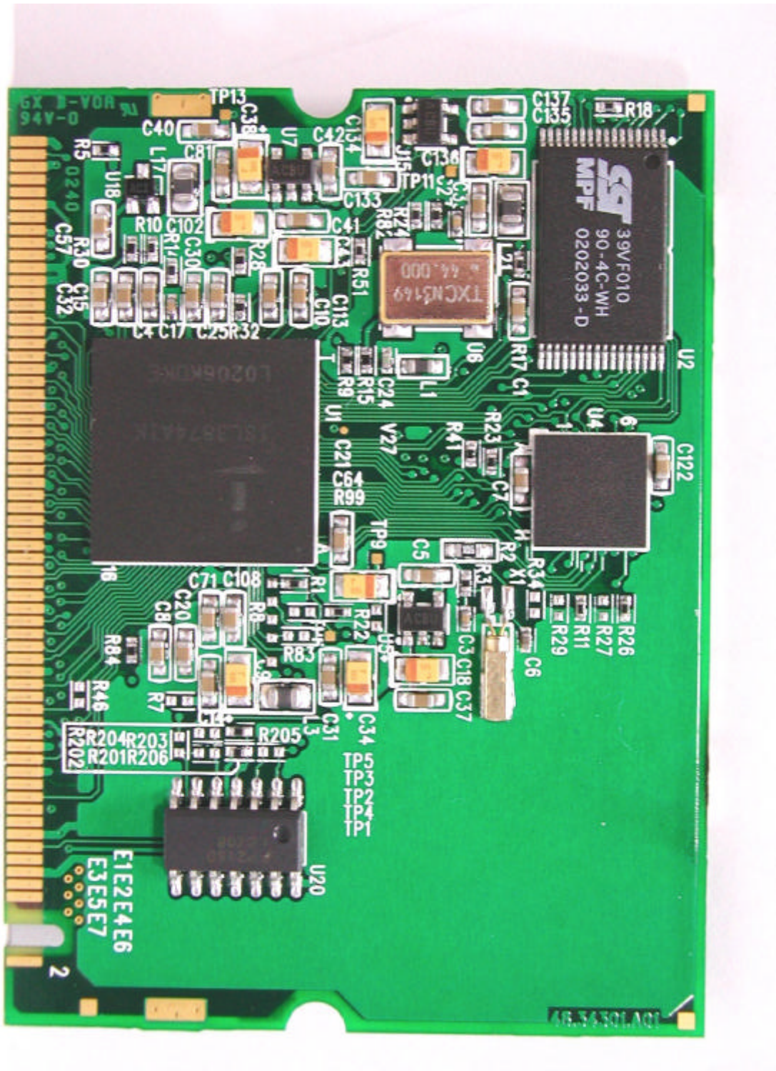
FCC ID: JVPAWL200 Rear View of the PWBA
