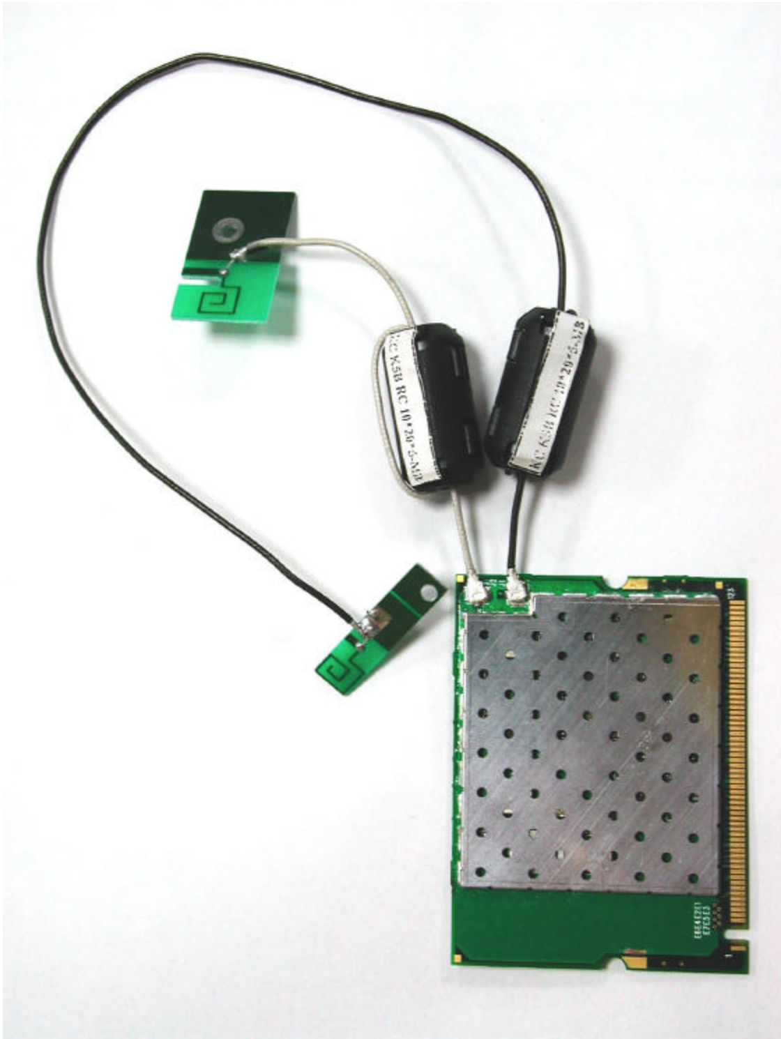
FCC ID: JVPAWL200 External Photo includes Antenna and PWBA.
