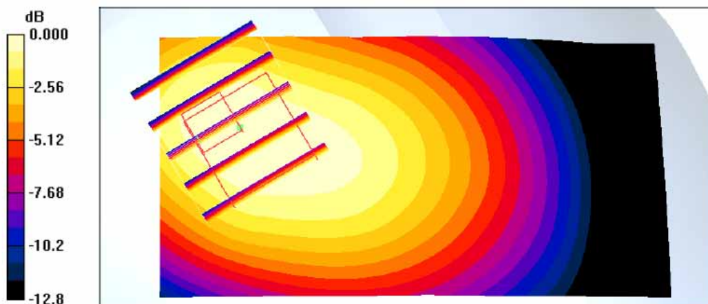
0 dB = 0.583mW/g
