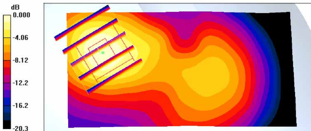
0 dB = 0.659mW/g
