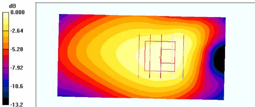
0 dB = 1.52mW/g
