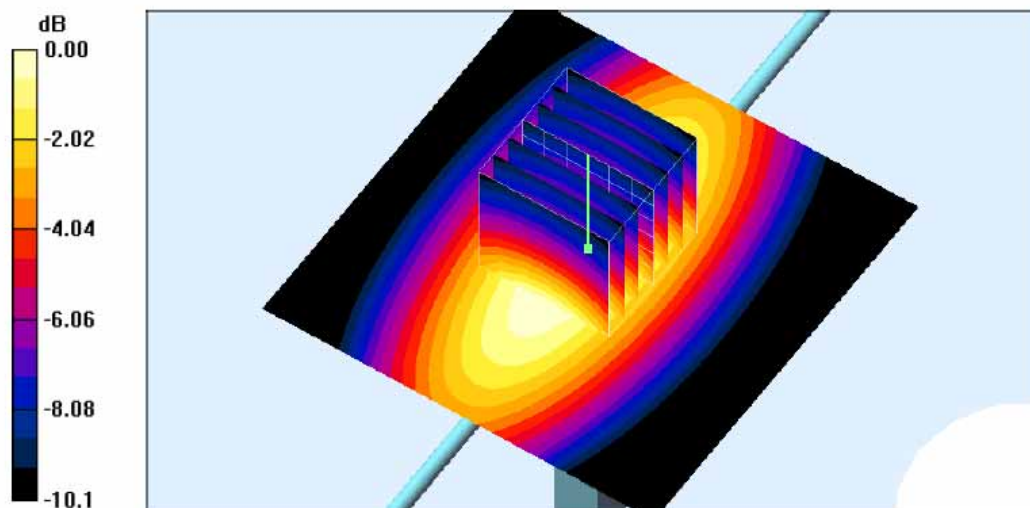
0 dB = 1.02mW/g
