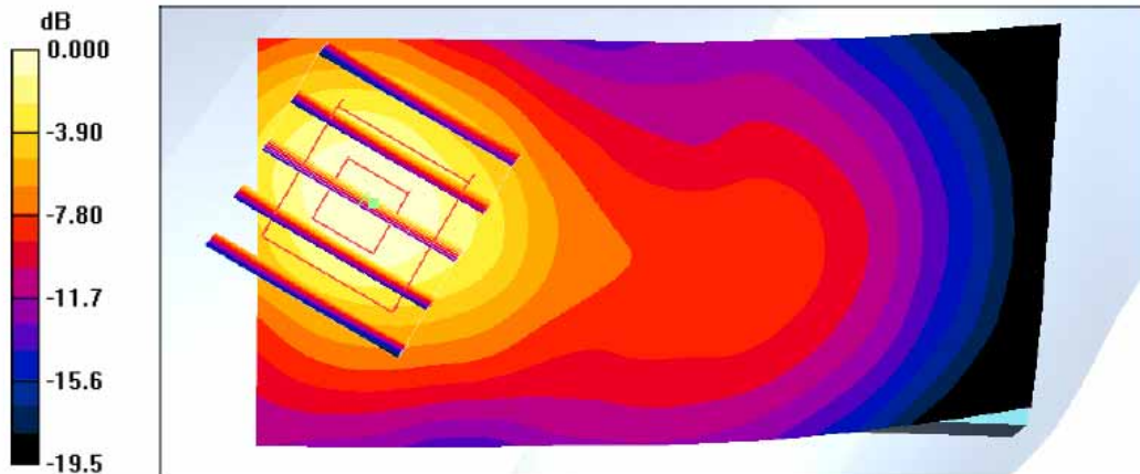
0 dB = 0.581mW/g
