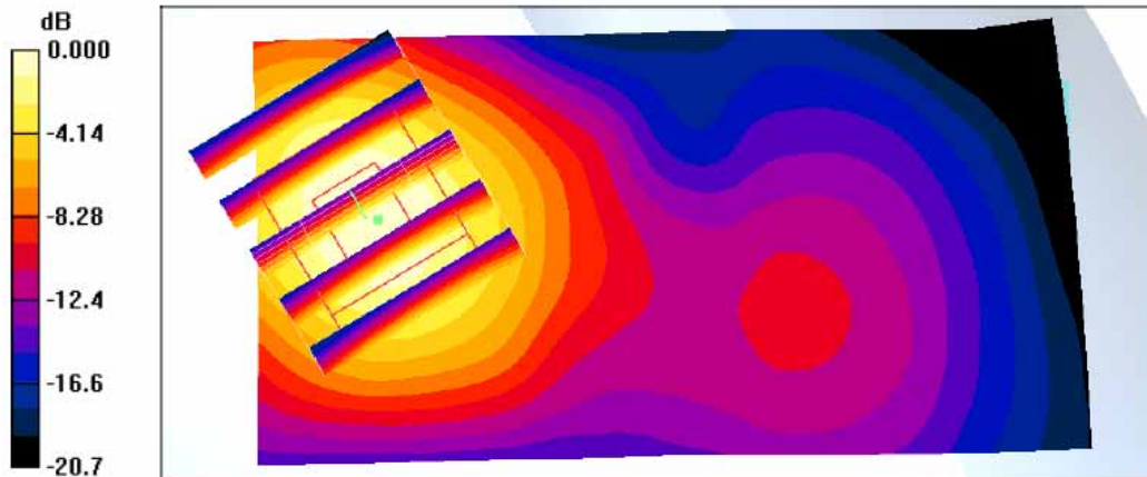
0 dB = 0.814mW/g
