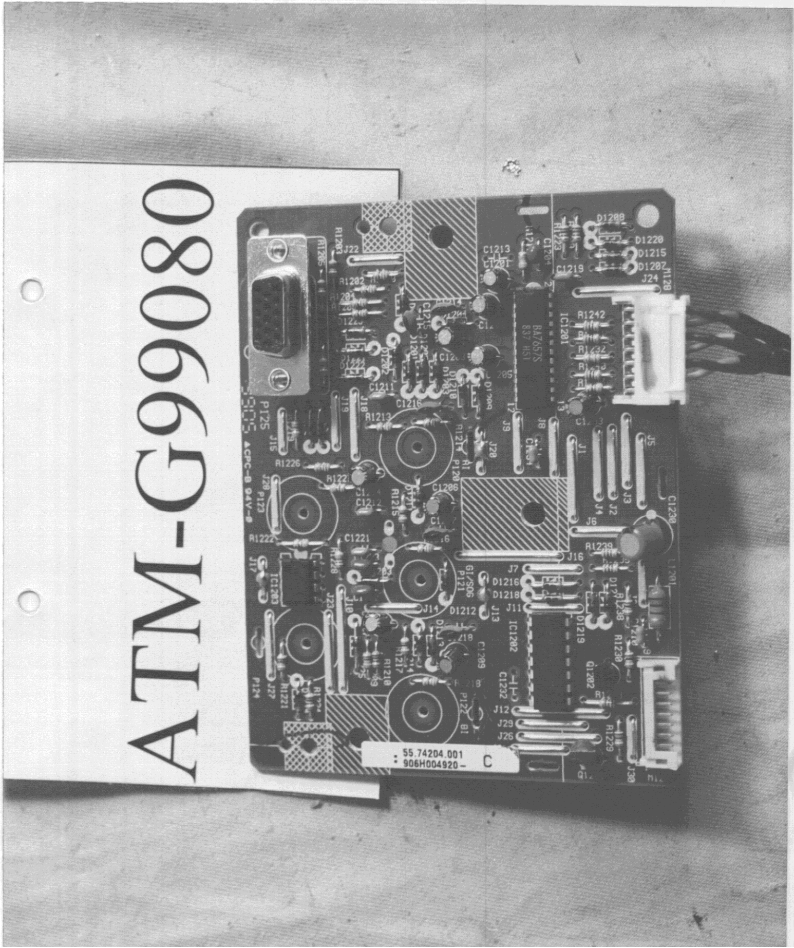
Figure 12 I/O Control Board (Component Side)
