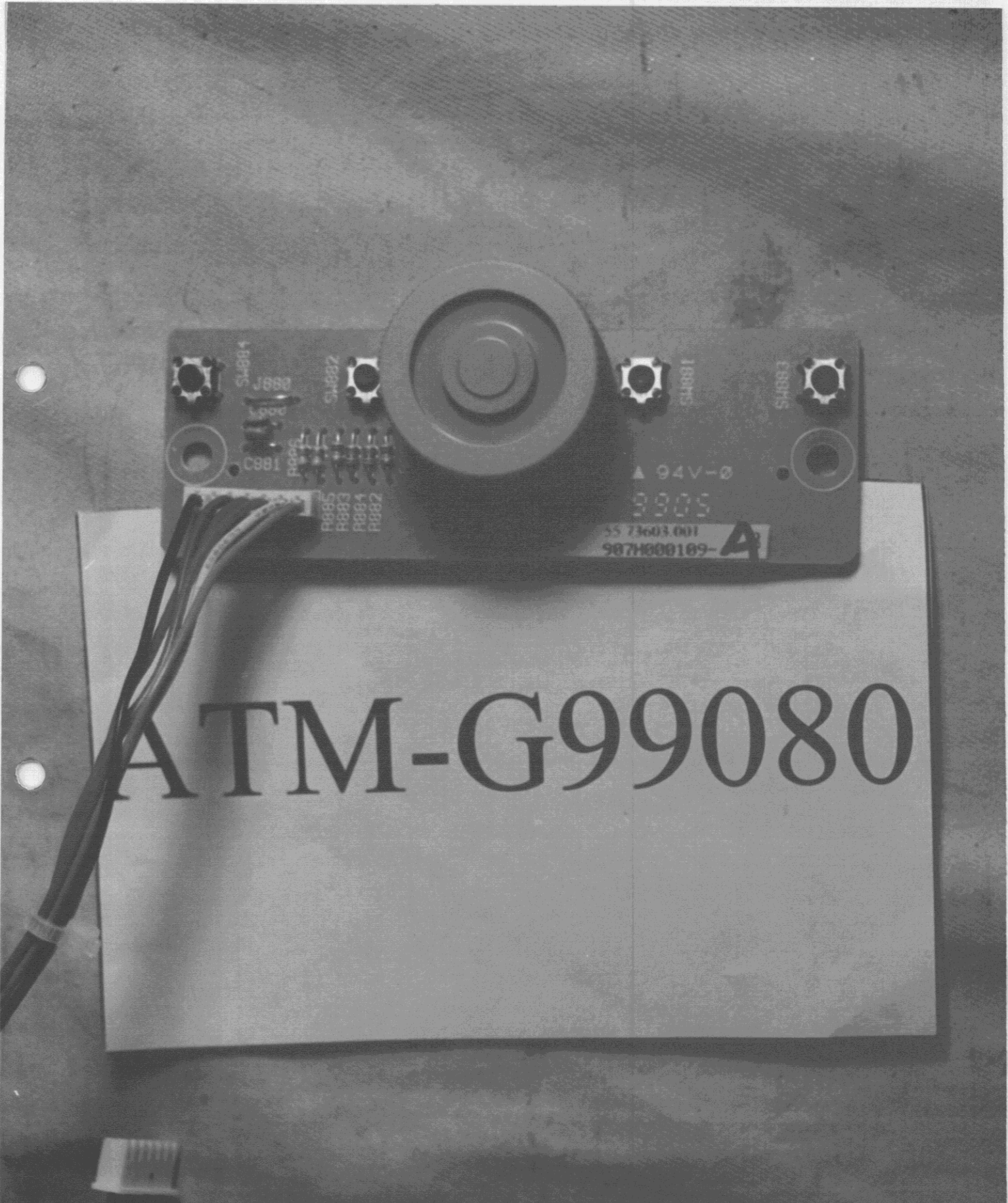
Figure 18 OSD Button Control Board (Component Side)
