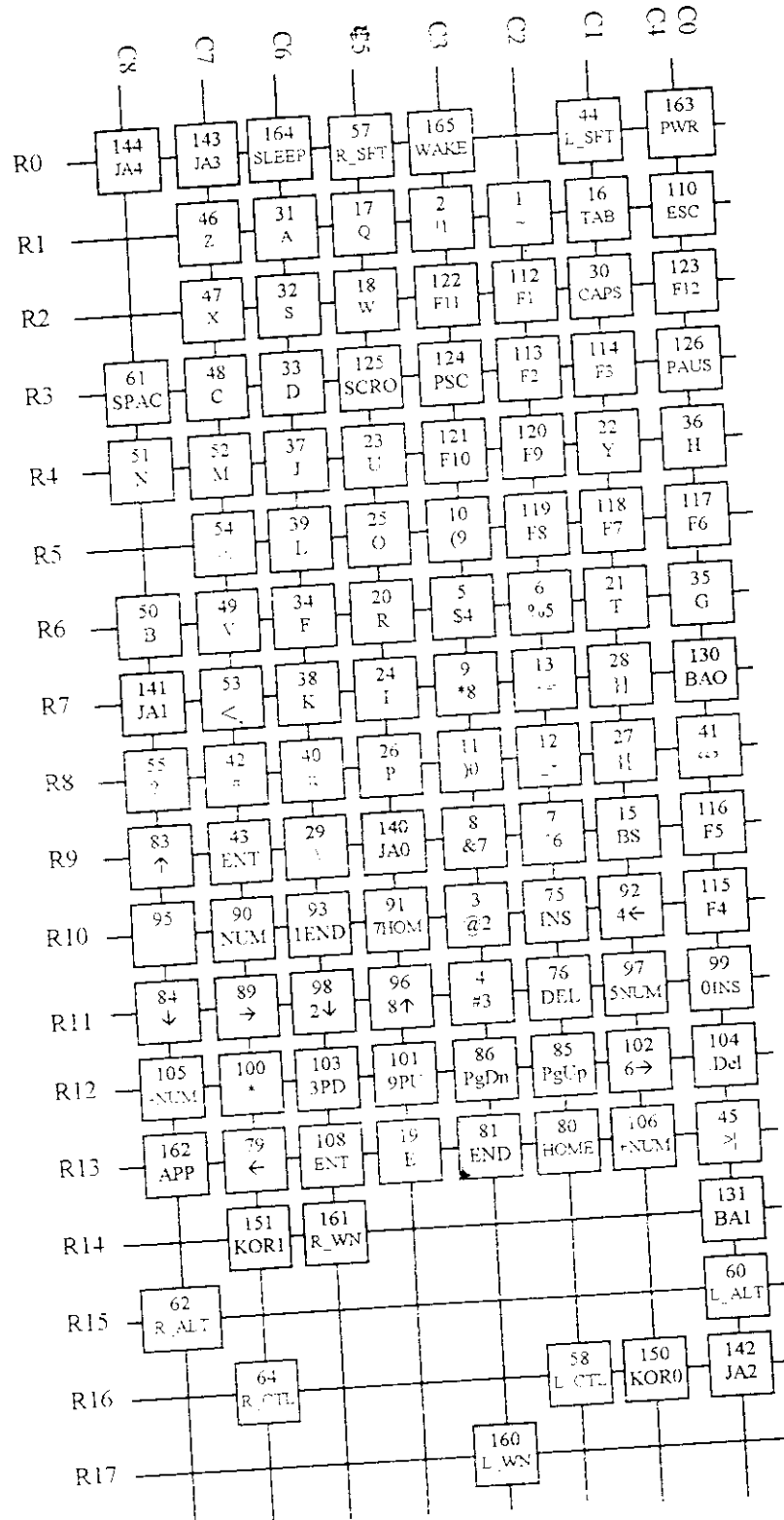
Fig. 6.1 Keyboard Matrix
