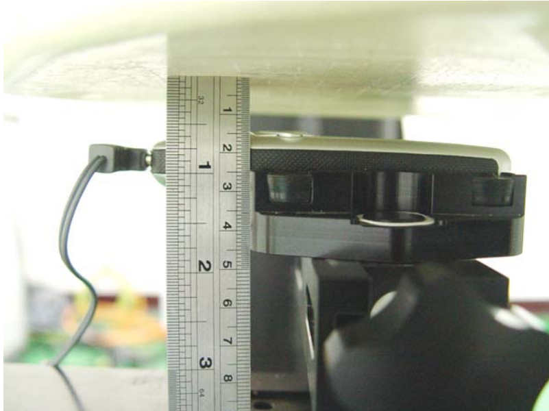
Fig. 9.7 Keypad Up With 1.5m Gap
