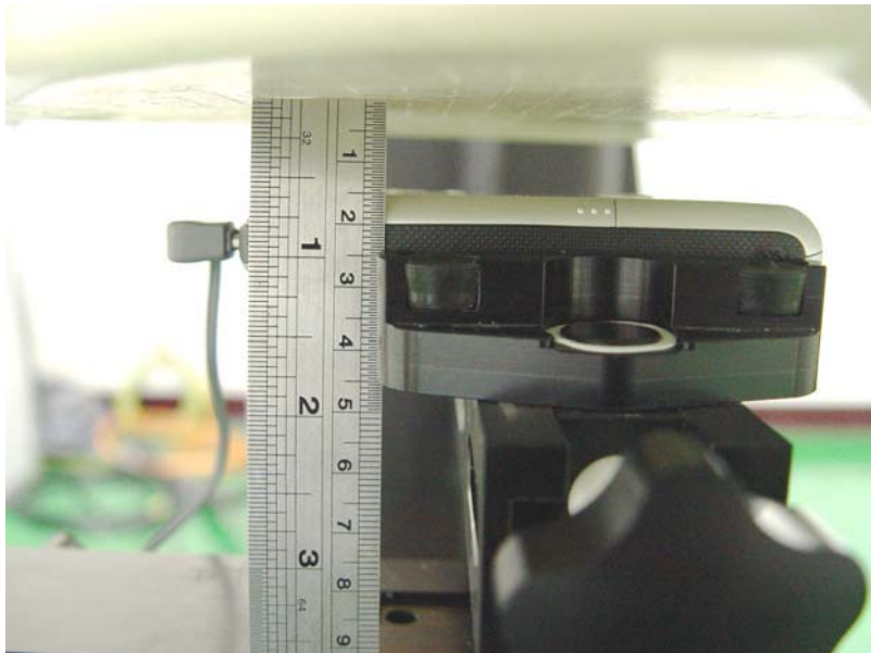
Fig. 9.8 Keypad Down With 1.5m Gap
