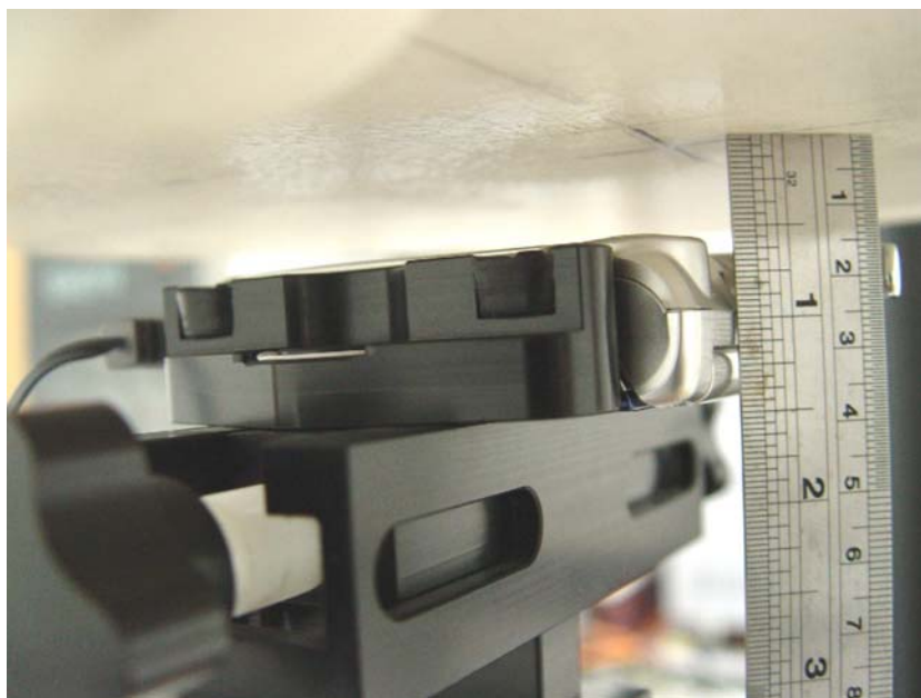
Fig. 9.8 Keypad Down with 1.5cm Gap for Standard Battery
