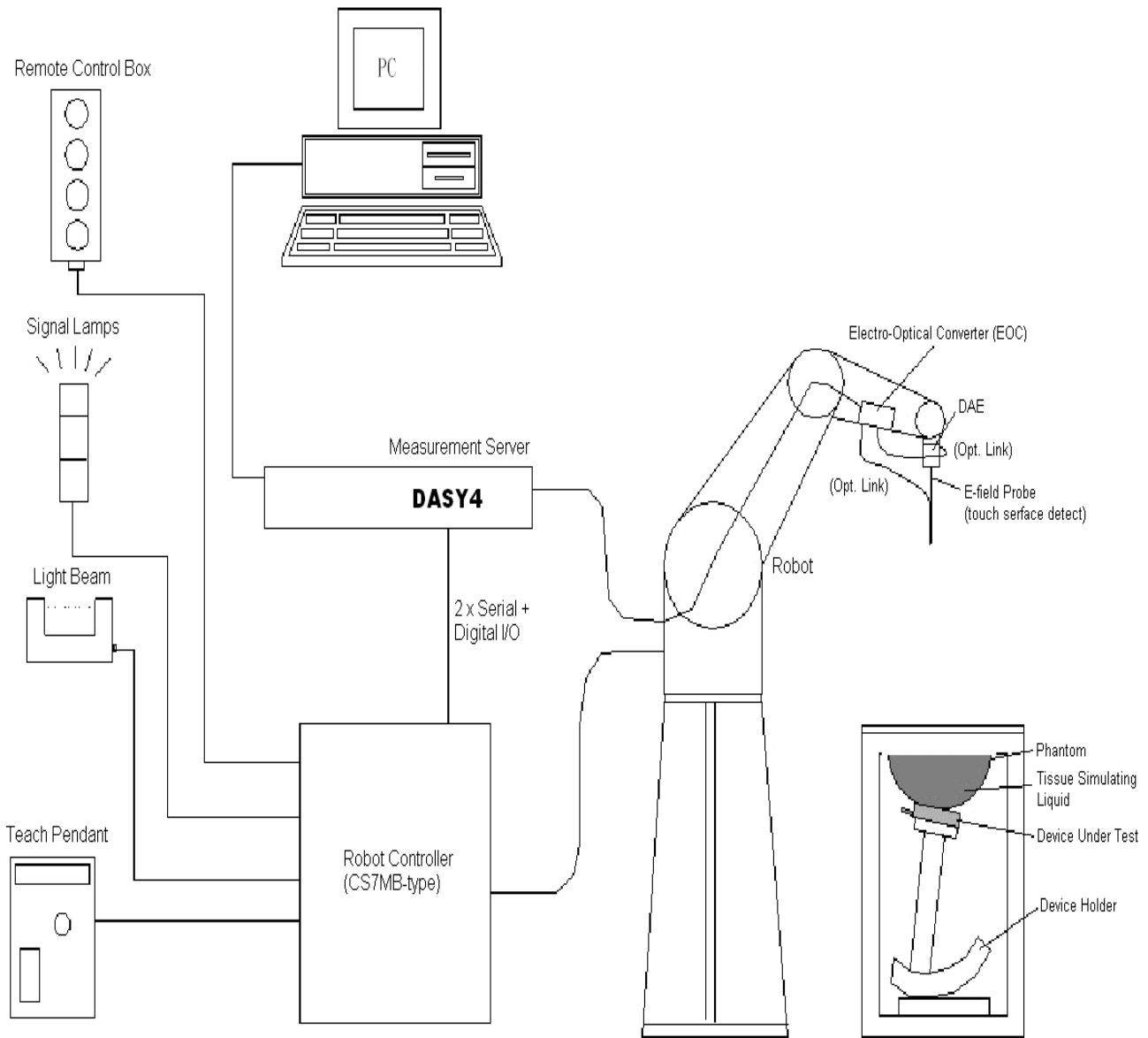
Fig. 5.1 DASY4 system
