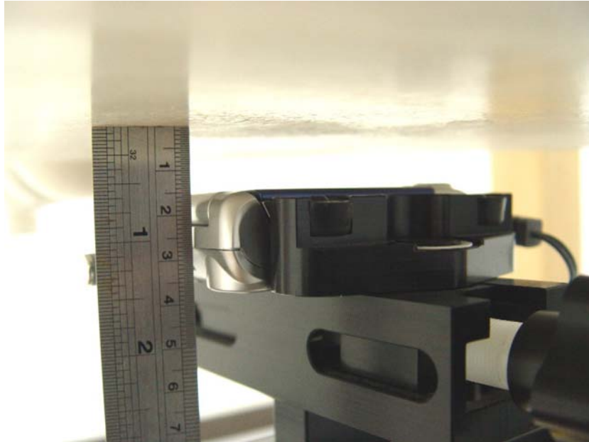
Fig. 9.7 Keypad Up with 1.5cm Gap for Standard Battery
