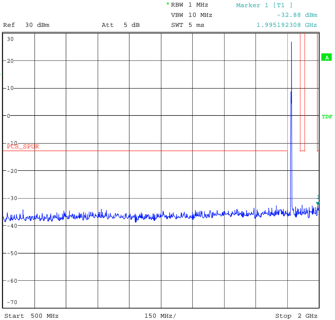
Figure 20 Spurious Emissions - GSM1900 – Channel 661
