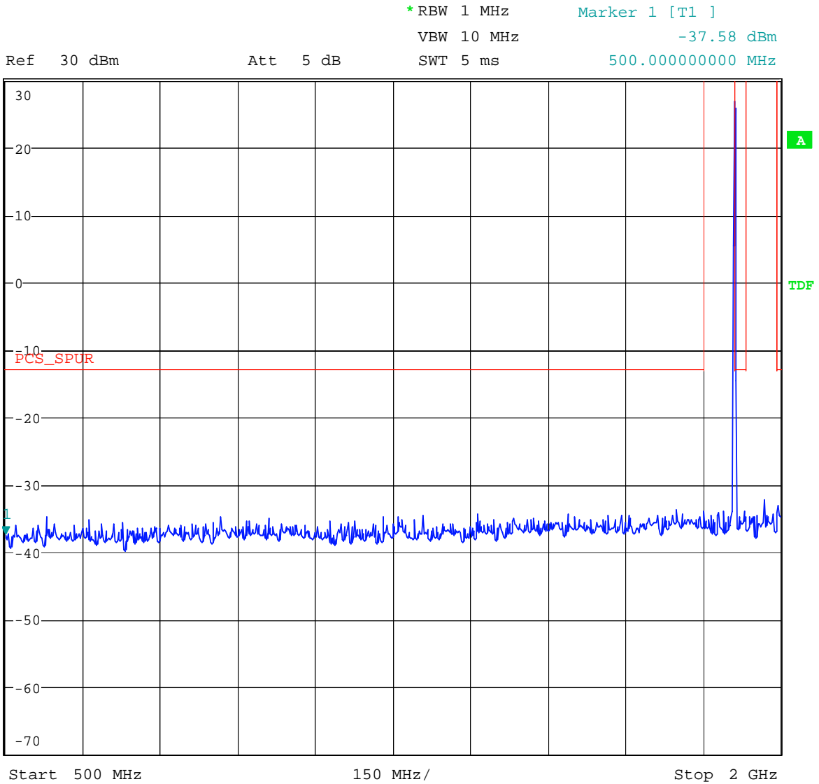
Figure 23 Spurious Emissions - GSM1900 – Channel 810
