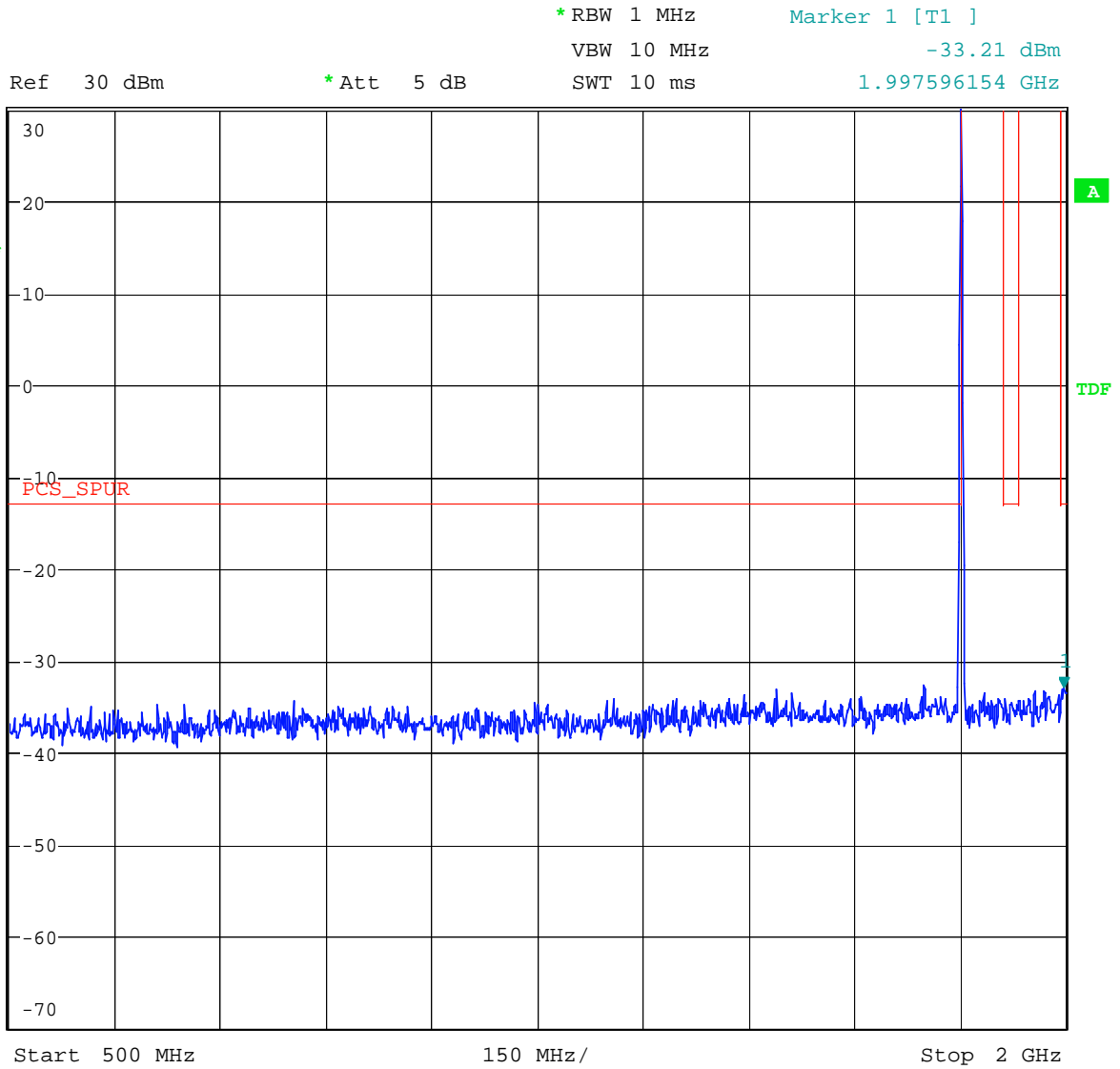
Figure 17 Spurious Emissions - GSM1900 – Channel 512
