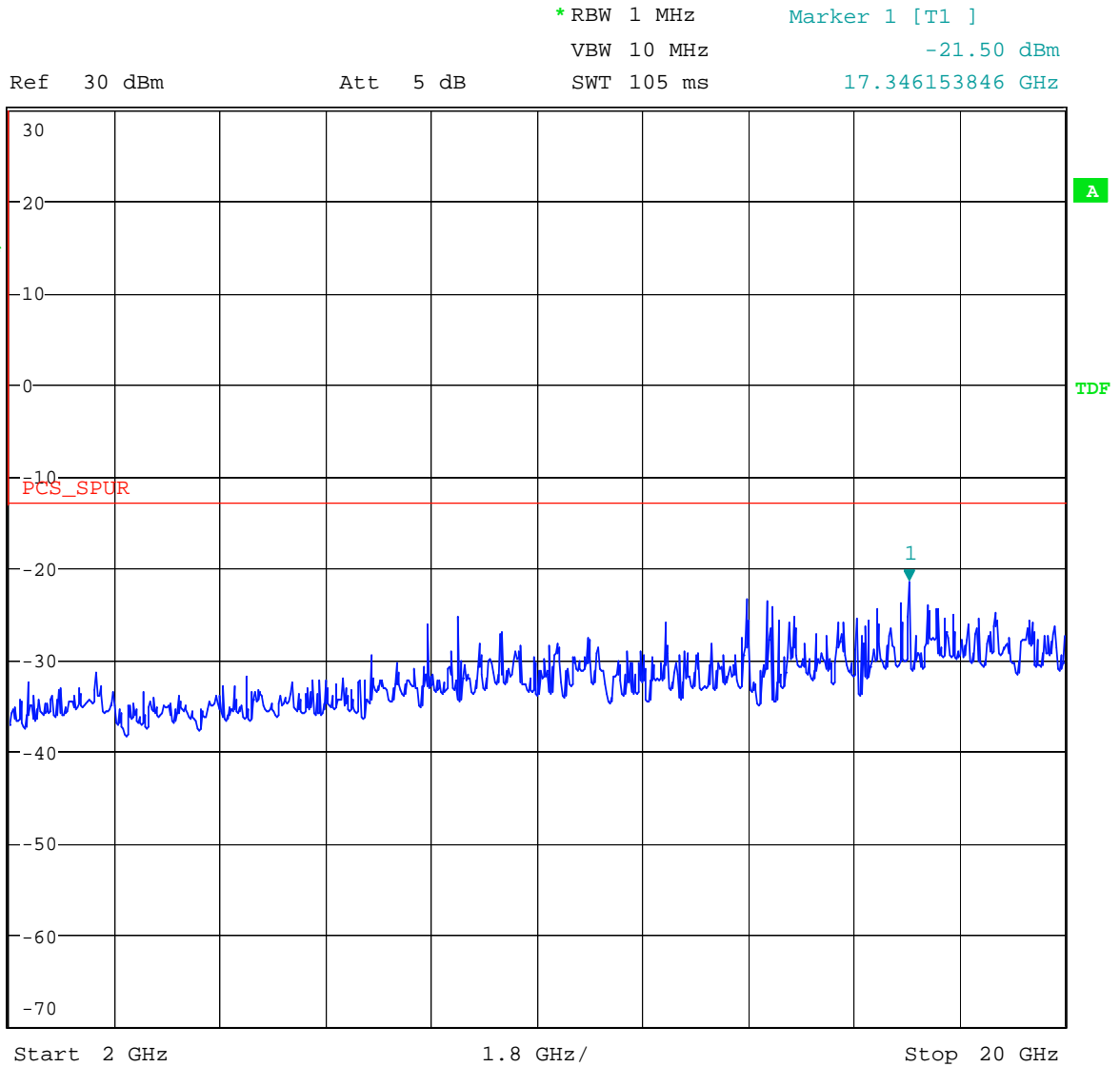
Figure 24 Spurious Emissions - GSM1900 – Channel 810
