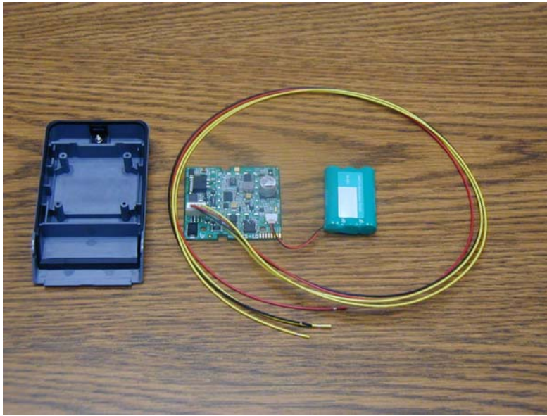
Original VAM module disassembled showing housing, PCBA, cable, and backup battery.
