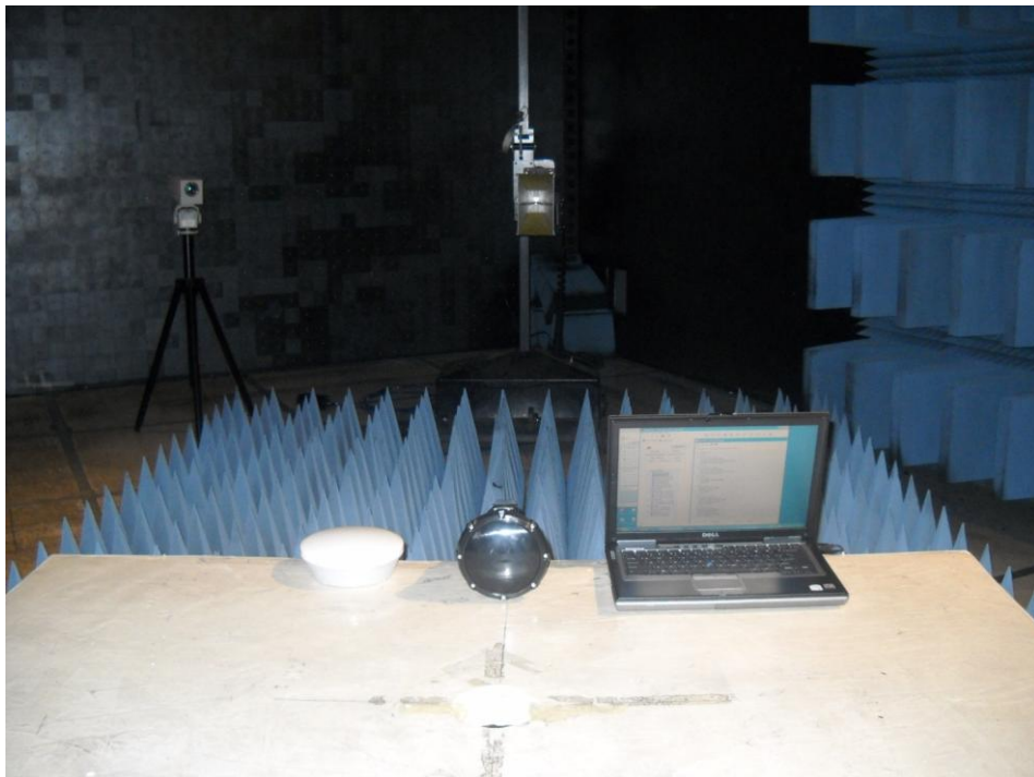
Emissions: > 1GHz (FCC 15B)
