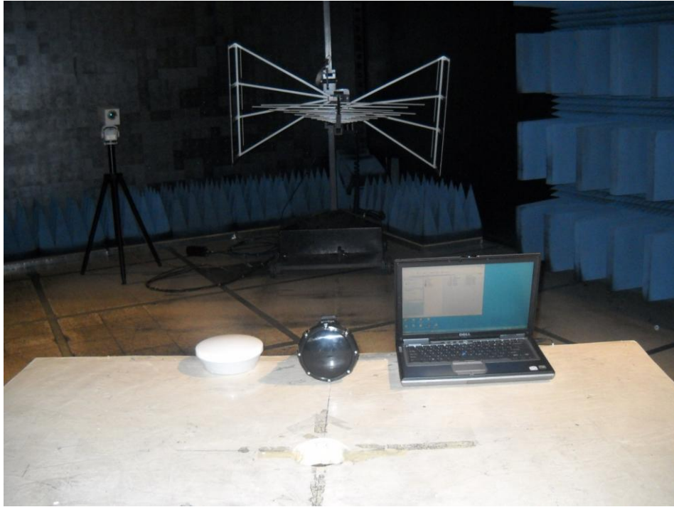
Emissions: 30MHz-1GHz (FCC 15B)
