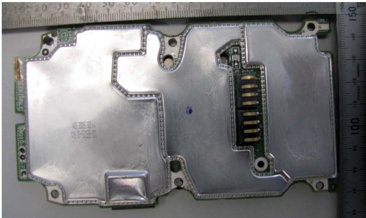
Main Board reverse (with Shields)
