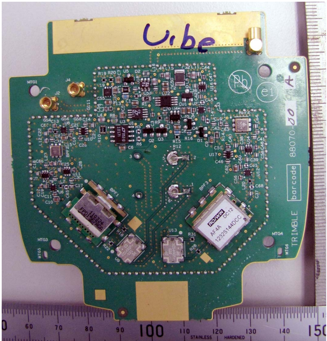
Low Noise Amplifier (LNA) board reverse (no Shield)
