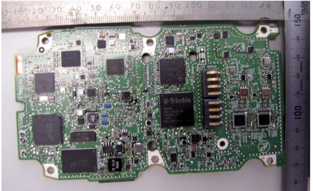
Main Board top (no Shields)
