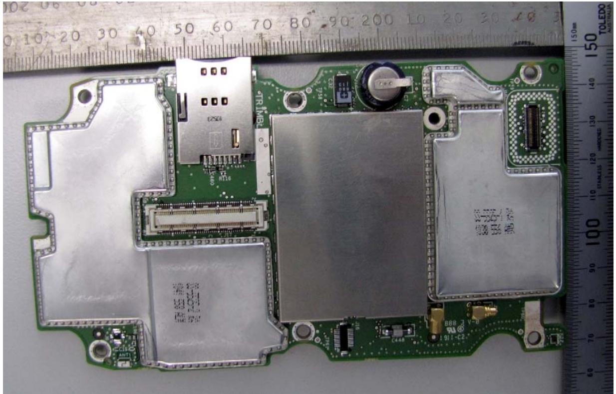
Main Board top (with Shields)
