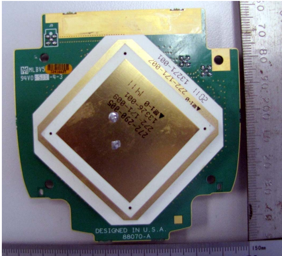
Low Noise Amplifier (LNA) board top
