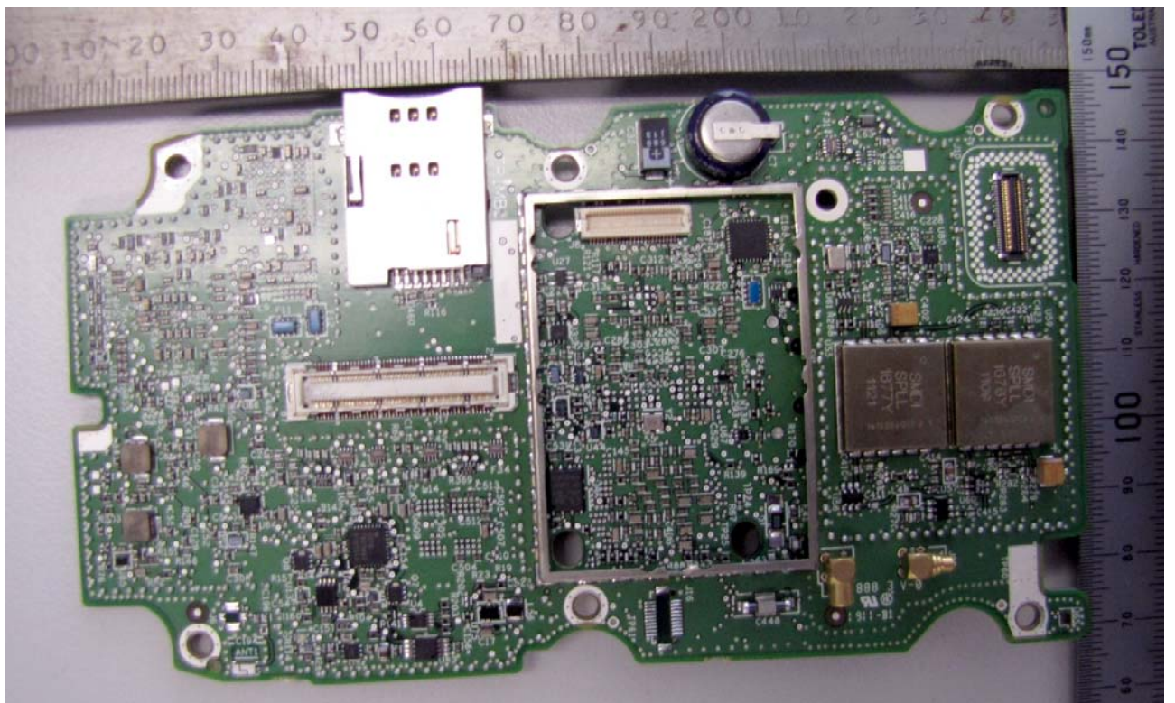
Main Board reverse (no Shields)
