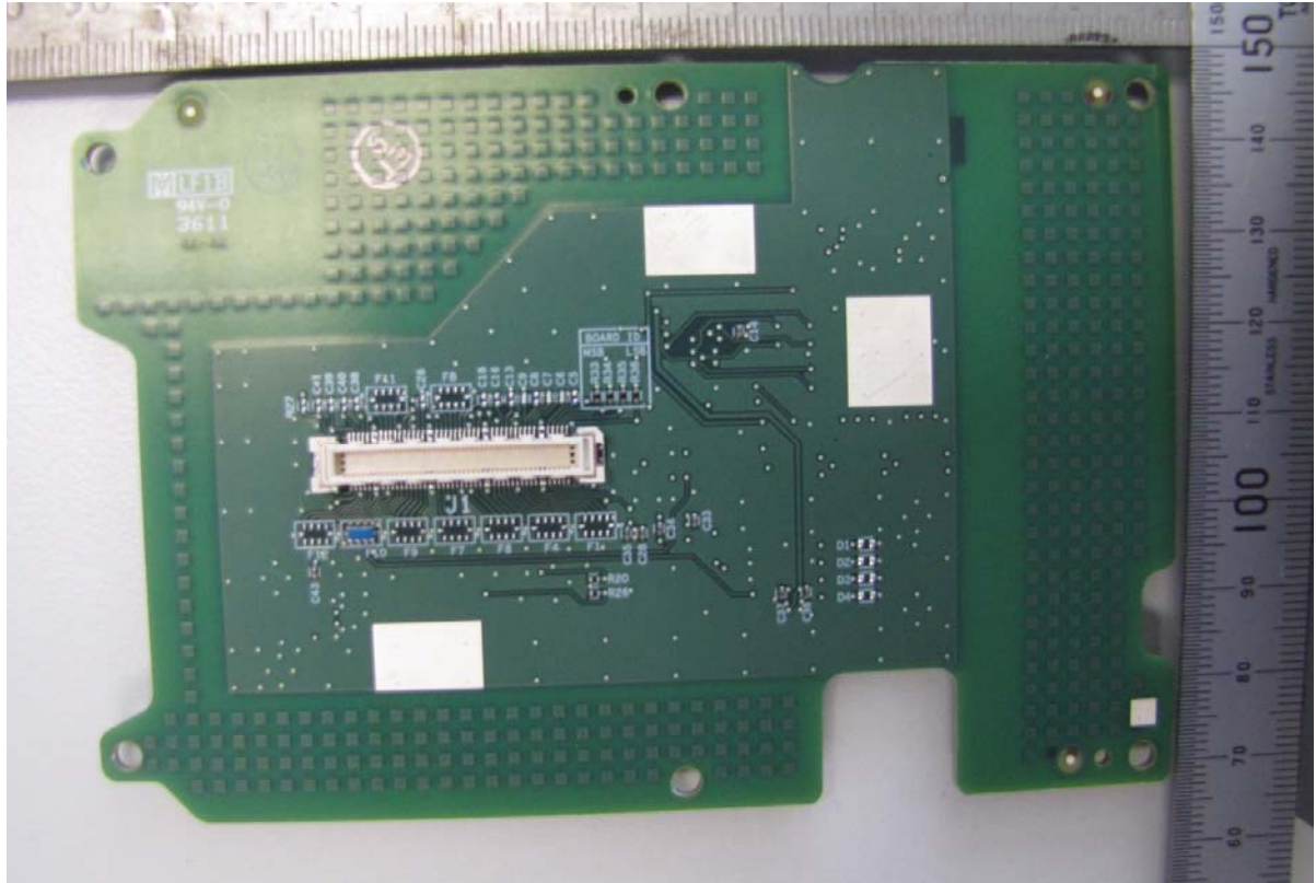
User Interface (UI) board reverse
