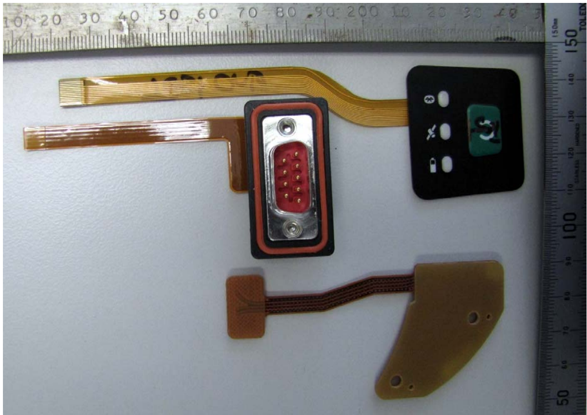
Keypad, Serial Port and Sensor Boards top
