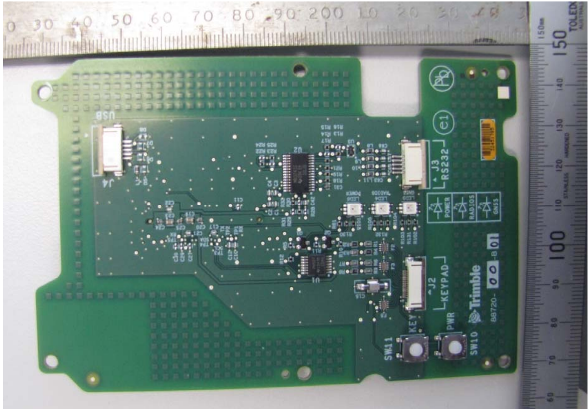
User Interface (UI) board top
