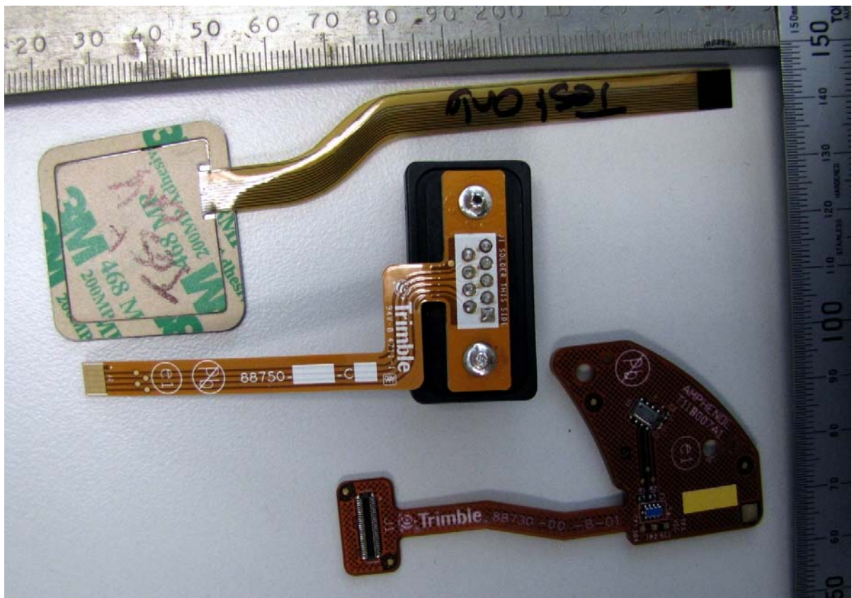
Keypad, Serial Port and Sensor Boards reverse
