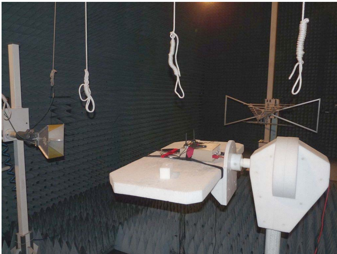
Photo 1: Test setup for radiated measurements (Enclosure, fully-anechoic chamber, 30 MHz – 10/20 GHz §22/24)
