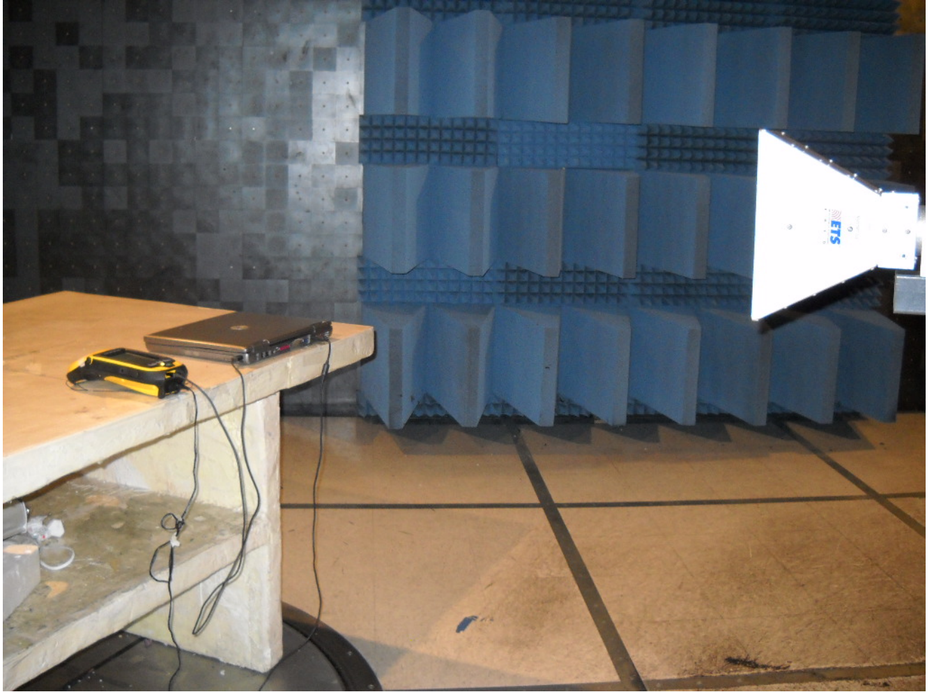
Radiated Emissions for WLAN/BT simultaneous Transmission
