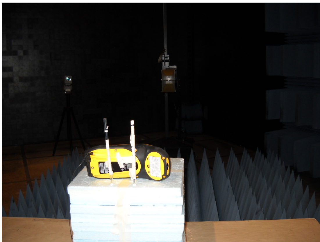
ERP/EIRP
