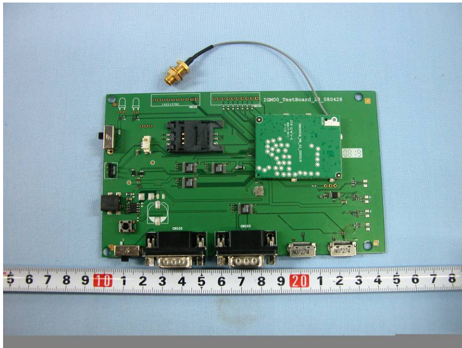
GSM/GPRS Module Host
