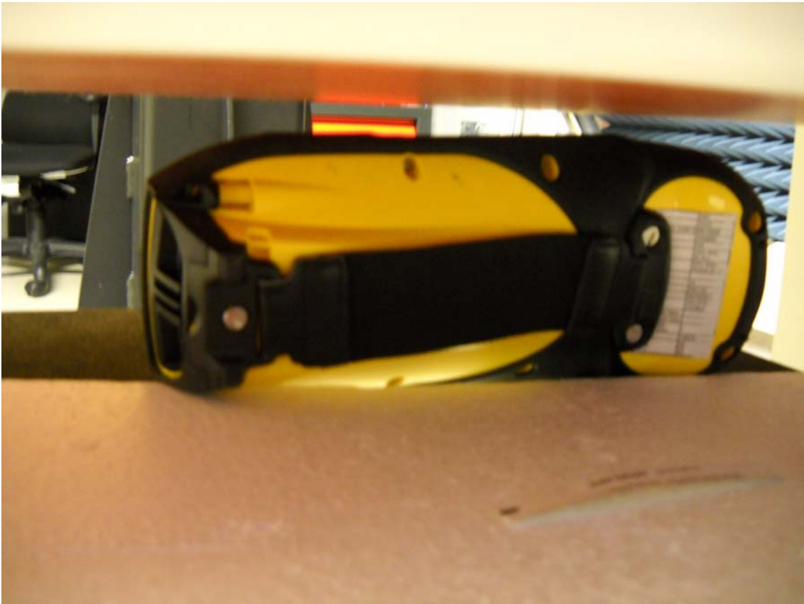
Photo 3. WLAN Right 10mm Position
