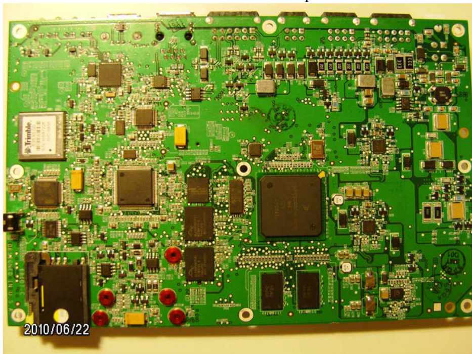
TVG-850 HSPA PCBA bottom side
