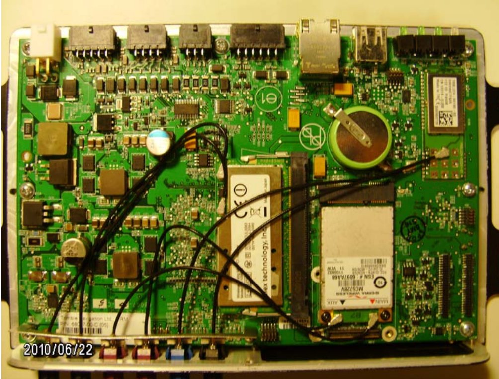
TVG-850 EVDO Internal (a) PCB Top (b) PCB Bottom
