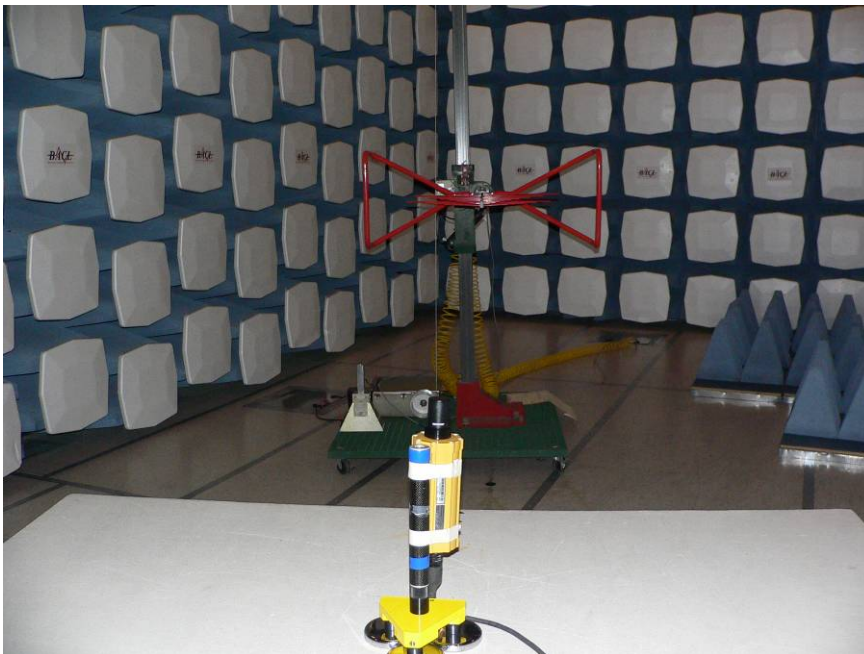
Radiated Emissions - Rear View with Omni antenna
